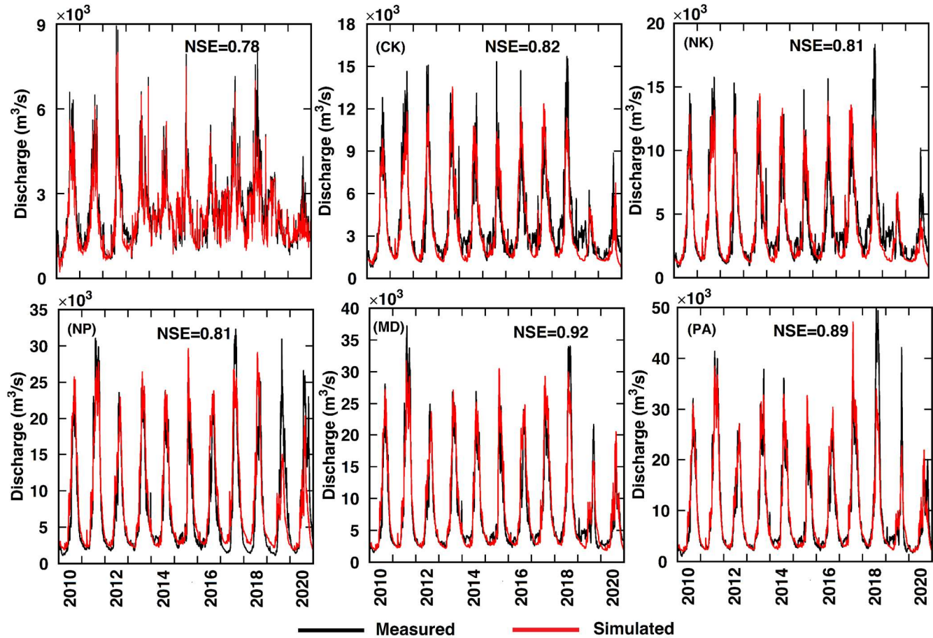
285 Figure 3. Comparison of the simulated time series discharge by the THREW hydrological model with measured data over the mega-dam period (2010-2020).
