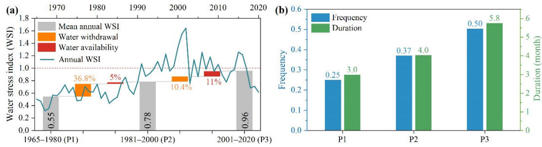
Figure 3. (a) Evolution of the regional water stress index (WSI) and its drivers. (b)
