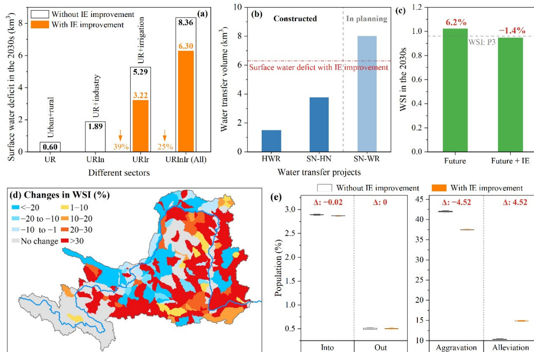
Figure 8. Impacts of improvement in irrigation efficiency (IE) on water stress
