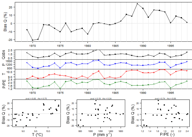
310 Figure 4: Illustration of the RAT results for the GR6J model applied to the Ognon River at Chavigny-sur-l'Ognon (north-east France): top plot represents the annual streamflow bias time series, the four middle plots represent the time series of the annual flow values and of the three climatic predictors, and bottom scatter plots represent the correlation between bias and annual temperature (left), precipitation (centre) and humidity index (right)
