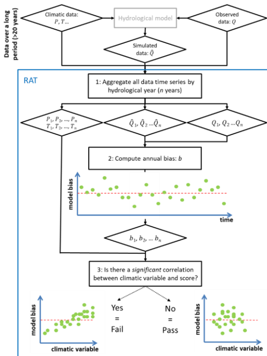
105 Figure 1: Flow chart of the robustness assessment test (RAT), with the three steps necessary to evaluate the robustness of a hydrological model (from Nicolle et al., 2021)
