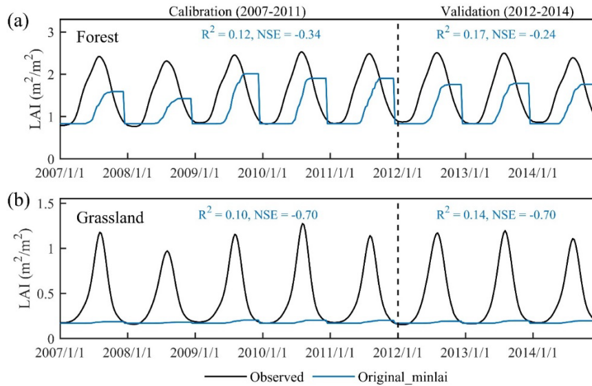
Figure S1: Temporal variability of the LAI during the calibration (2007–2011) and validation (2012–2014) periods. 8-d LAI time series observed by satellite and simulated by the original SWAT-Carbon model with adjusting non-growing season LAI for Forest (a) and grassland (b).
