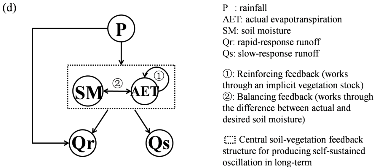
330 Figure 5: The comparison of endogenous linking structures of hydrological system built using two approaches, Granger's causality test and system dynamics approach. a-c, illustration of how the structure built using causal analysis, d structure built using system dynamics approach.
