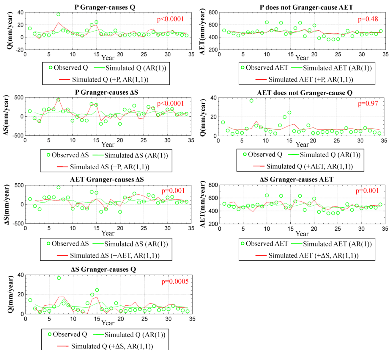
315 Figure 4: Causal relationships among four hydrological variables of FP catchment. P, Q, AET, and \Delta S indicate rainfall, streamflow, actual evapotranspiration, and catchment water storage change respectively. AR(p) represents the autoregressive model, where "p" is called the order of the model and represents the number of lagged values we want to include. AR(p,q) represents that additional q-order variable is included. The p-value indicates significance at 95% confidence. Comparable results of Granger's causality test were seen for the other catchments (not shown for clarity purpose).
