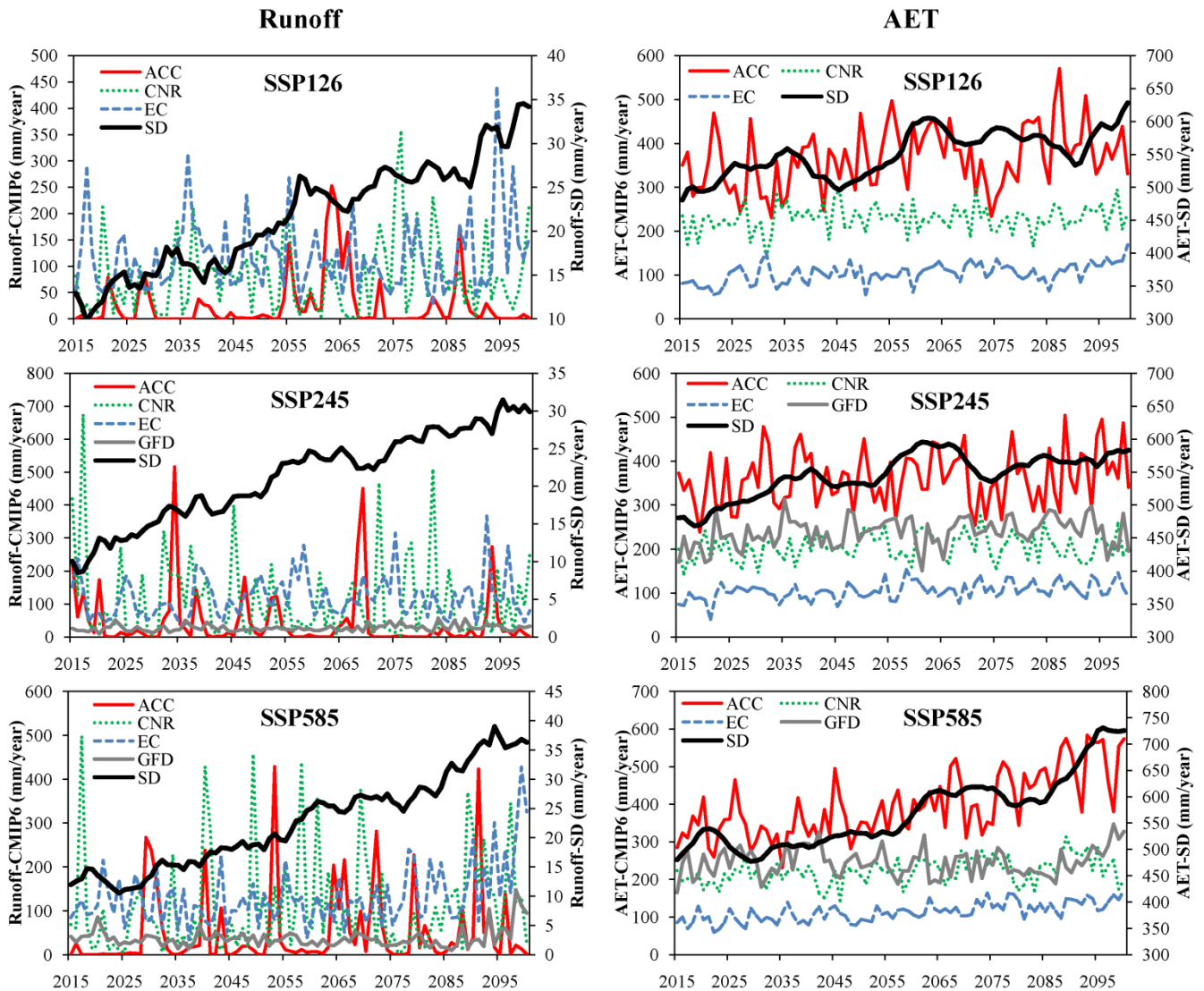
400 Figure 7: Future runoff and AET predicted by system dynamics approach under three climatic scenarios and their comparison with predictions from four GCMs. All the dynamics were simulated with fixed ESMS and without human interventions (GP and VEG = 0).
