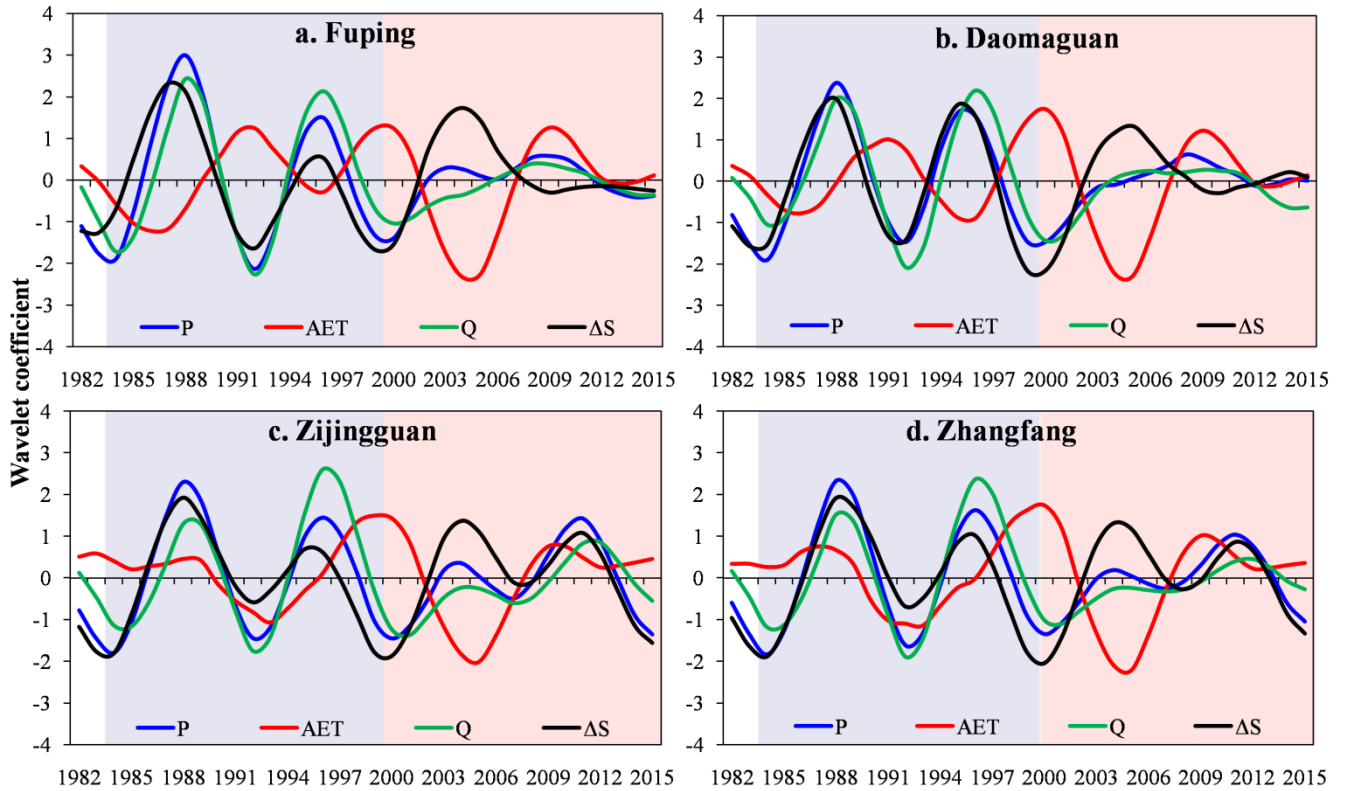
Figure 2: Wavelet coefficients of four signals (precipitation, P, actual evapotranspiration, AET, streamflow, Q, and catchment water storage change, \Delta S ) with contraction parameter of 8 in the Fuping catchment (a), Daomaguan catchment (b), Zijingguan catchment (c), and Zhangfang catchment (d). Blue background indicates wet phase from 1984 to 2000, while the red background indicates dry phase from 2001 to 2015.
