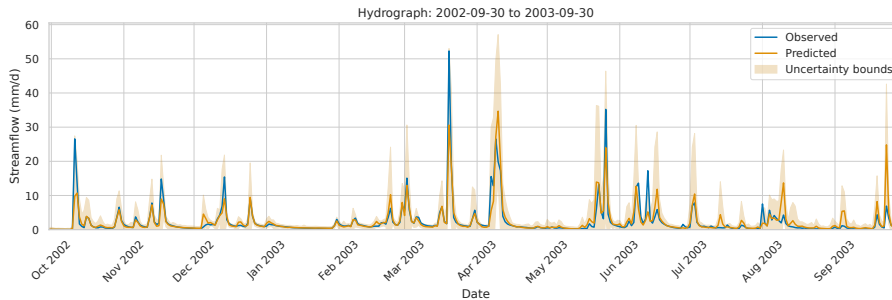
Figure 2. The observed streamflow (blue), the prediction (gold), and HopCPT’s prediction interval (light gold; offline mode and model states as input) for a random basin (id: 02077200) from October 2002 to October 2003. For the prediction interval we set \alpha = 0.05 . HopCPT generates wider prediction intervals where the prediction model is uncertain. Hence it covers the observed streamflow also for values where the predicted and the real streamflow are quite different. In confident areas, the prediction interval is much narrower.
