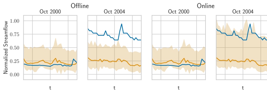
Figure 5. The real streamflow (blue), the prediction (gold), and HopCPT’s prediction interval (light gold) for a basin (id: 12447390) in October 2000 and October 2004. The two plots one the left show HopCPT in the offline mode — the right two plots in the online mode. The online mode allows HopCPT to account for the distribution shift in October 2004.
