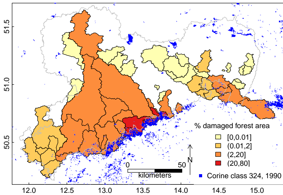
Figure 4. Map of forest damage using Corine 1990 class 324 (transitional scrub forest). Catchments are grouped by the relative area of forest damage.
