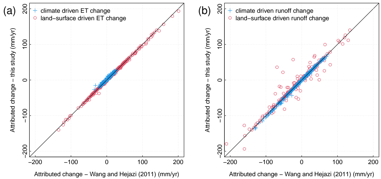
Figure B1. Comparison of the decomposition method of this study with the method of Wang and Hejazi (2011) using the Mezentsev (1955) parametric Budyko function to separate climate and land-surface induced changes on E_T (panel a) and runoff (b). Here all decadal transitions of all catchments with sufficient data are used for the comparison.
