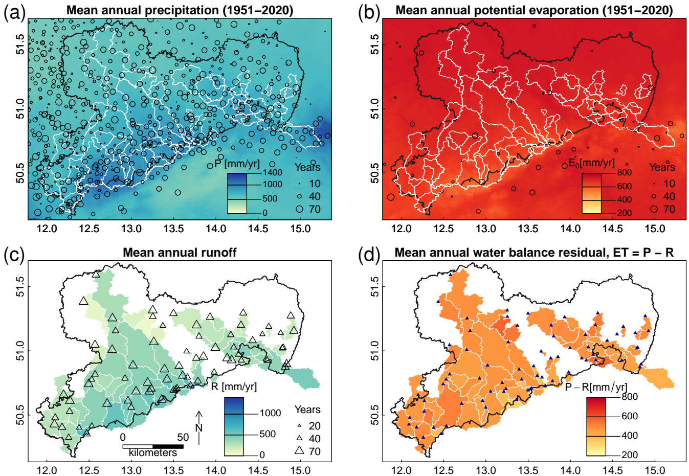
Figure 3. Maps of long term (1951–2020) annual mean (a) precipitation, (b) annual potential evapotranspiration (FAO-56 grass-reference evapotranspiration E_0 (Allen et al., 1994)), (c) annual runoff and (d) the residual water budgets ( E_T = P - R ). Observation stations which have been used to derive spatial fields of P and E_0 are depicted as circles with diameter corresponding to the number of years of available data. The maps of mean annual precipitation P and the FAO reference potential evapotranspiration E_0 have been derived by averaging the individual annual raster maps used to calculate the basin averages. Note, that panels (a) and (c) as well as (b) and (d) use the same color scale respectively.
