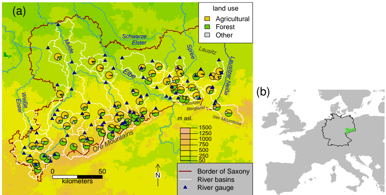
Figure 2. Map of the federal State of Saxony, its topography, catchment boundaries and river discharge measurement stations analysed analyzed in this study. Land-use fraction depicted as pie chart of each catchment is derived from CORINE Land-cover data from the year 2000. Panel b) shows the location of Saxony with Germany and Europe for orientation using polygon data from NUTS 2021 ( ec.europa.eu . europa.eu). The figure is adapted from Renner et al. (2014).
