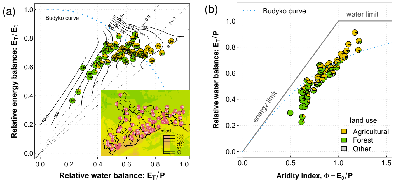
Figure 5. Long term catchment water and energy partitioning. The pie-charts show the areal percentage of land use of each basin. In the right panel, catchments. Panel a) plots the relative energy vs. water balance. The average basin elevation is used to predict the contour lines using local polynomial (LOESS) regression. This demonstrates the general height dependency of the basins-catchments climate. Further, and land-use (Corine dataset of 2000) as well as the transition from wet basins with high runoff ratio to lower values is also reflected by land-use. The inset in panel a) shows a map of the catchments, its gauge id number and altitude as background raster. Panel b) visualizes the same data but in the classic Budyko diagram with relative water balance vs. aridity index. The catchments are depicted as pie-charts which show the areal percentage of land use of each catchment.
