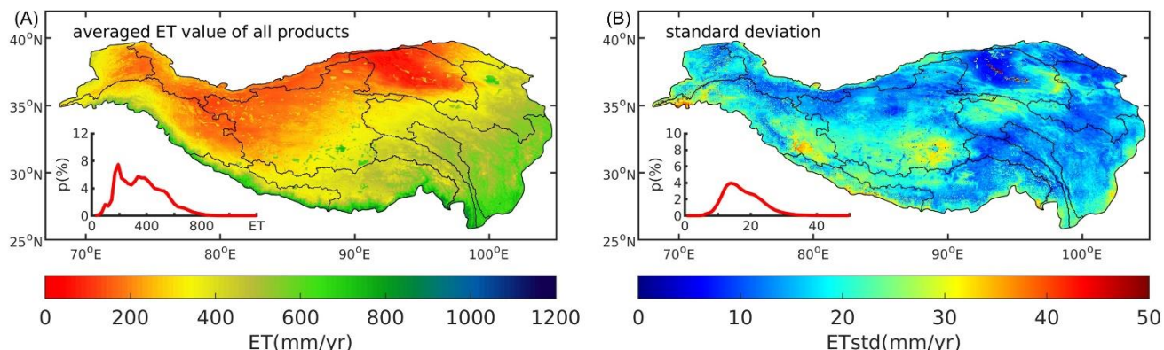
295 Figure 4: Mean multi-year average annual ET from the 22 products and the standard deviation across the TP during their overlap period (2003~2013). The inset in each panel shows the histogram.
