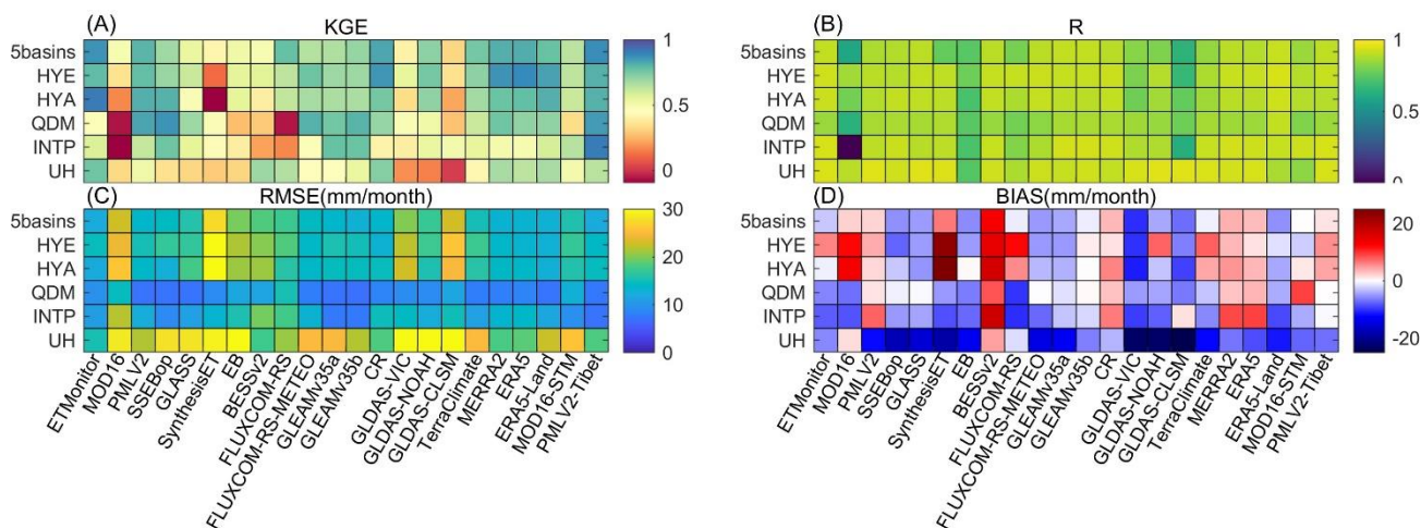
Figure 3: Summary of the evaluation of ET products against basin-scale ET based on water balance estimates for the headwaters of Yellow basin (HYE), headwaters of Yangtze basin (HYA), upper Heihe basin (UH), Inner TP (INTP) and Qaidam (QDM). ‘5basins’ presents the validation results when timeseries from all five basins were appended together to calculate the performance indicators.
