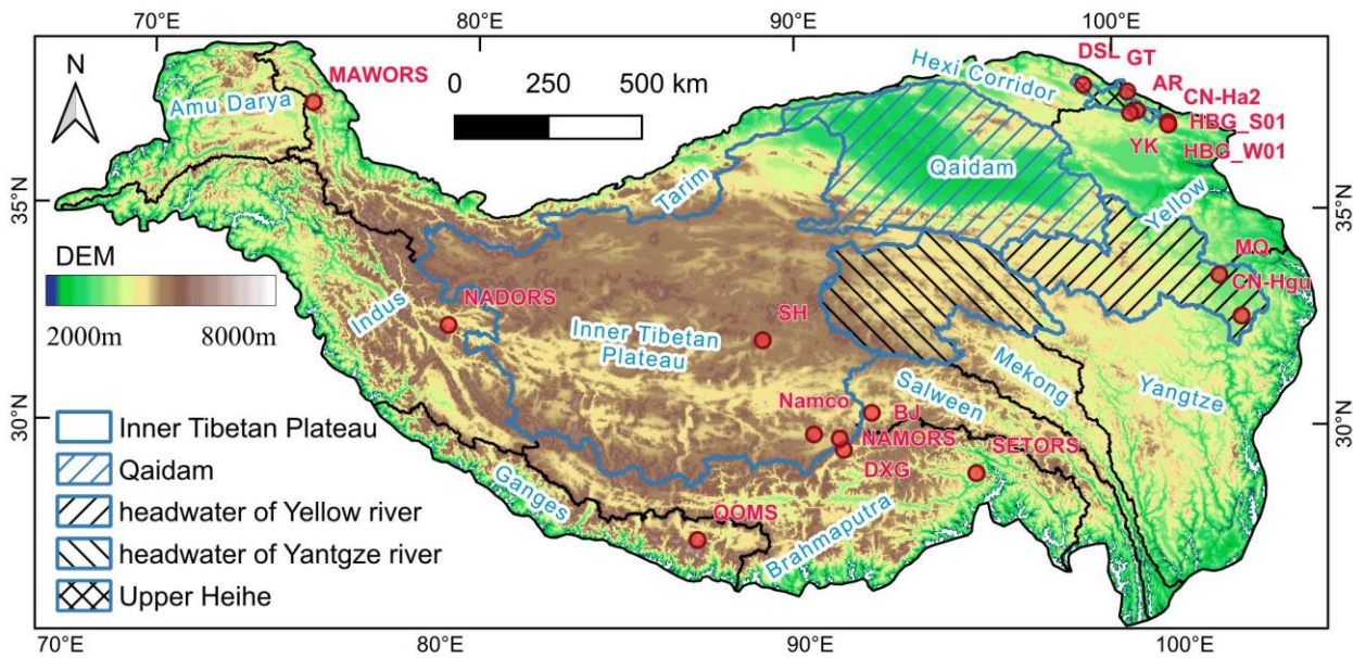
120 Figure 1: Location of the selected ground flux tower observation sites and major river basins in the TP, with elevation shown as background. The selected basins where the evaluation of ET products using water balance-based data was carried out are also shown.
