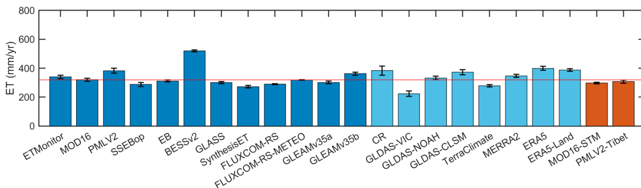
310 Figure 5: Bar plot of the multi-year (2003~2013) averaged ET of different products in the TP. The red horizontal line represents the average ET of all products. The global ET datasets based on satellite remote sensing are in dark blue, the global ET datasets based
