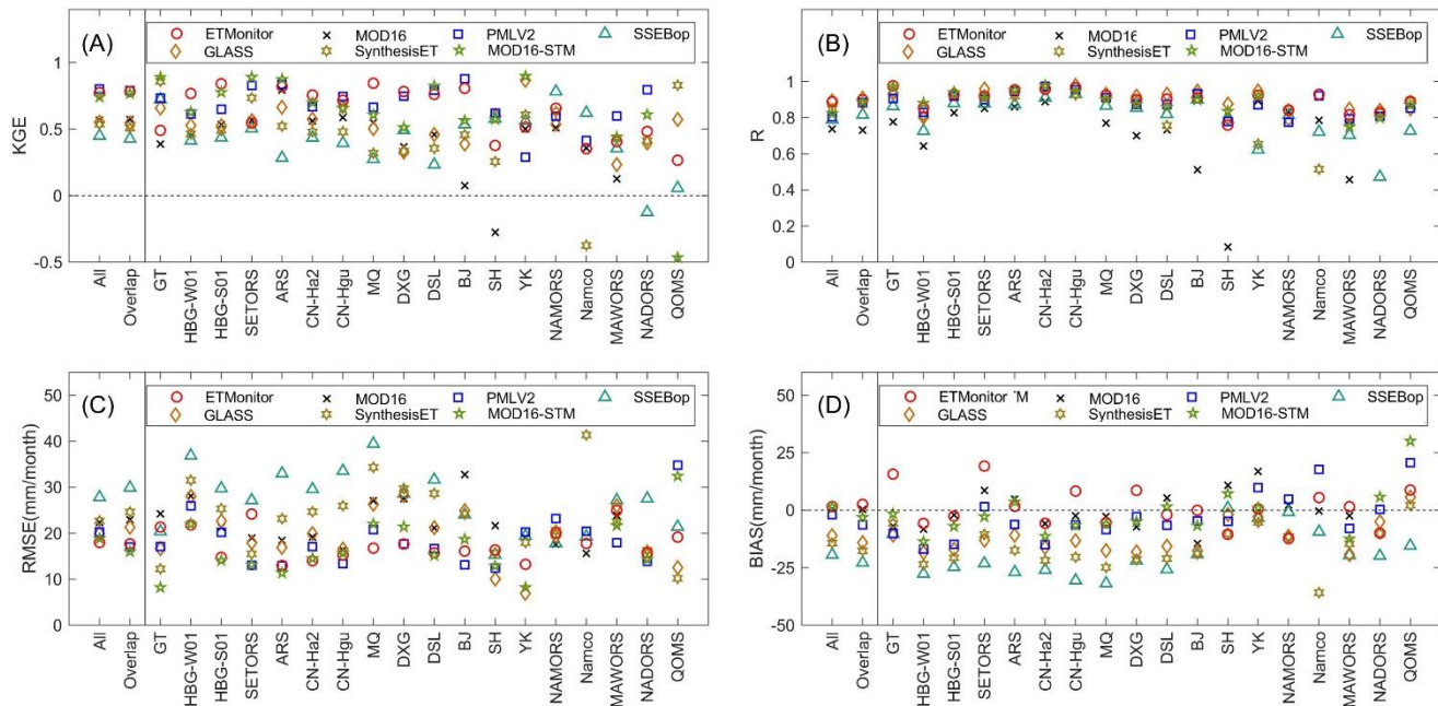
255 Figure 2: Summary of the validation results of high-resolution ET products against flux tower measurements. ‘All’ indicates that the validation results are obtained based on different samples depending on the availability of each product, while ‘Overlap’ represents the validation results are obtained based on consistent time frame and same sample numbers (mainly vegetation covered sites) for every product.
