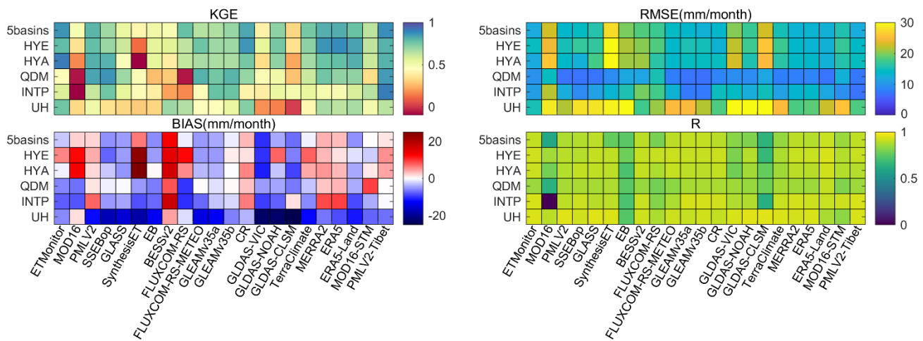
270 Figure 3: Summary of the evaluation of ET products against basin-scale ET based on water balance estimates for the headwaters of Yellow basin (HYE), headwaters of Yangtze basin (HYA), upper Heihe basin (UH), Inner TP (INTP) and Qaidam (QDM). ‘5basins’ presents the validation results when data from all five basins were used together.
