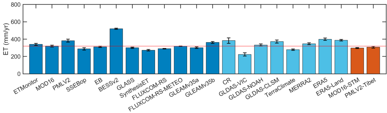
305 Figure 5: Bar plot of the multi-year (2003~2013) averaged ET of different products in the TP. The red horizontal line represents the average ET of all products. The global ET datasets based on satellite remote sensing are in dark blue, the global ET datasets based on land surface models and analysis global ET dataset are in light blue, the regional ET datasets are in red. It should be noted that some products only provide ET values for the vegetation-covered regions, e.g., MOD16, FLUXCOM-RS and FLUXCOM-RS-Meteo, and there are two products (MOD16-STM, PMLV2-Tibet) cannot cover the regions outside of China.
