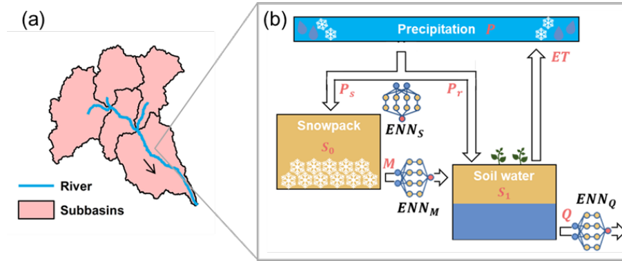
Figure 1. The schematic diagram of hybrid distributed-semi-distributed models. (a) The basin is first divided into many sub-basins; (b) All meteorological and hydrological processes included in the EXP-Hydro model are calculated in each sub-basin. The precipitation partition, snowmelt, and runoff modules can be optionally replaced by embedded neural networks. Detailed formulations of these processes refer to the main text.
