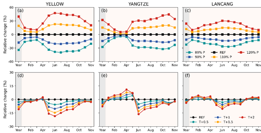
Figure 7. Relative change of annual (grey shadingsbackground ) and monthly(yellow shadingsbackground ) runoff response to the perturbed precipitation (a-c) and air temperature (d-f) in Yellow, Yangtze, and Lancang, respectively.
