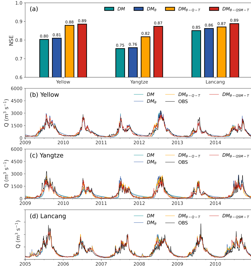
Figure 3. The comparison of simulated ( DM , DM_{\theta} , DM_{\theta-Q-T} , and DM_{\theta-QSM-T} models) and observed runoff processes in the evaluation period at the trained TNH, ZMD, and JZ station in Yellow, Yangtze, and Lancang, respectively.
