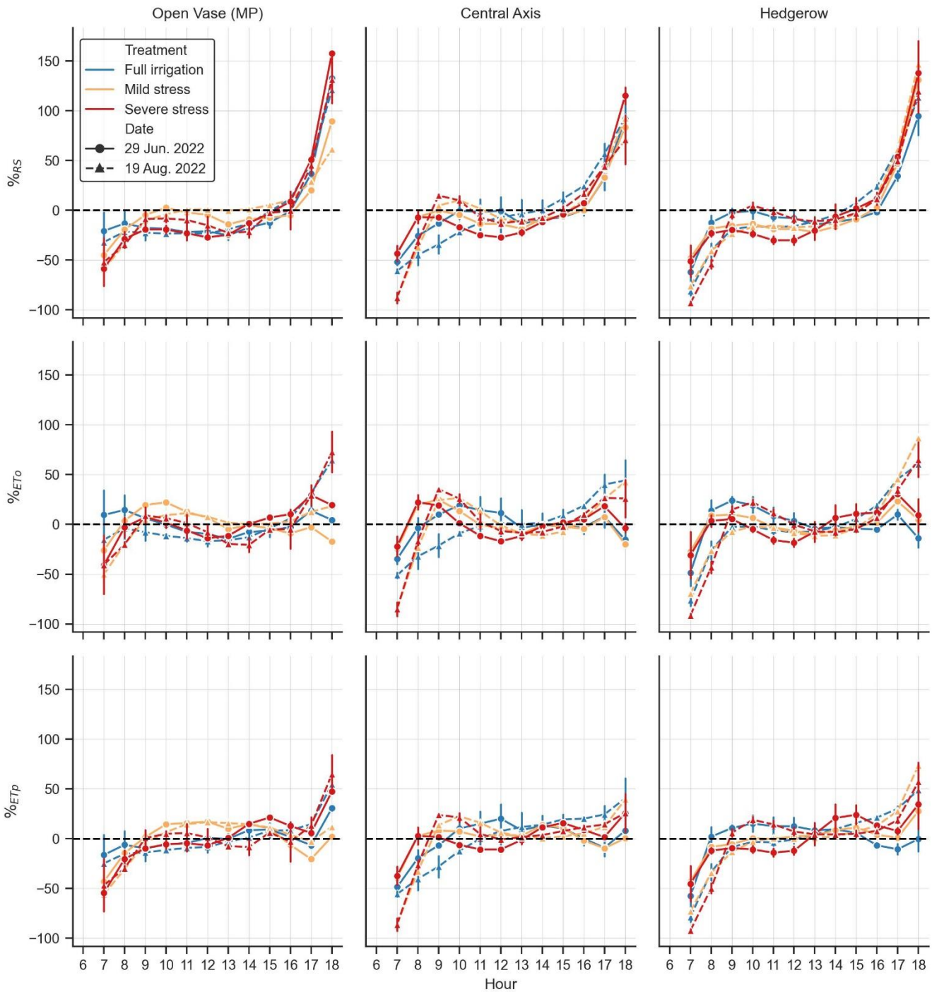
Figure 6. Daily evolution of difference between hourly and daily mean of \alpha_{RS} , \alpha_{ETo} and \alpha_{ETp} . \alpha represents the ratio between transpiration and the reference variable, while '%' corresponds to the formula 100 \times (\alpha_{Hour} - \alpha_{Day}) / \alpha_{Day} , where the subindex indicates the respective method.
