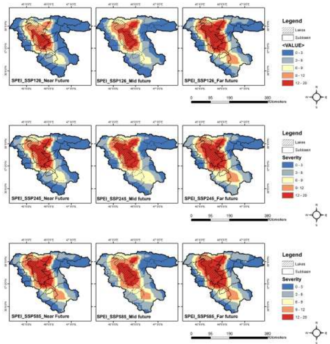
Figure S2. Maps showing SPEI drought severity over ULB in the near (2021-2040), mid (2041-2060), and far (2081-2100) future under SSP1-2.6, SSP2-4.5, and SSP5-8.5
