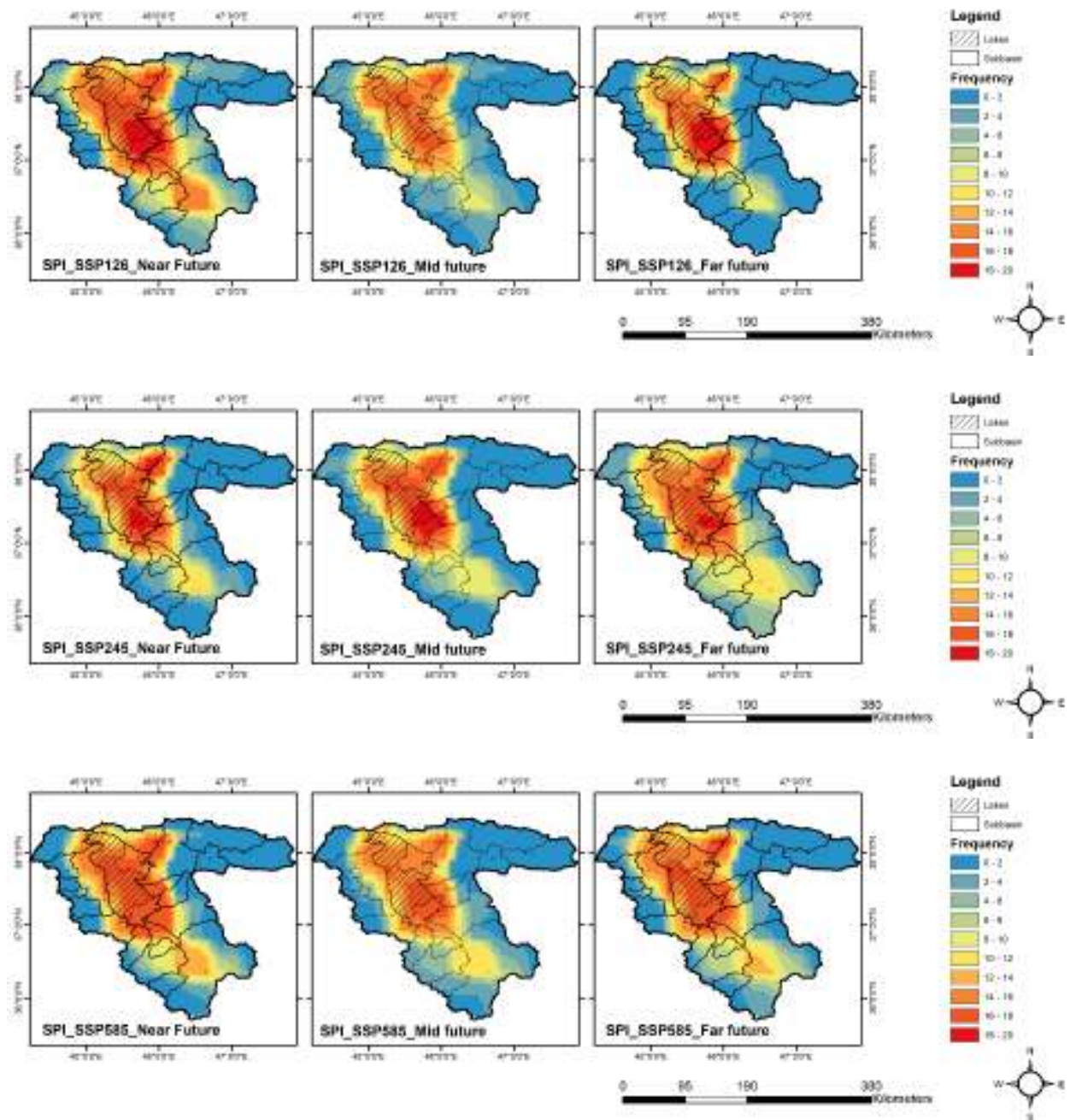
Figure S4. Maps showing SPI drought frequency over ULB in the near (2021-2040), mid (2041-2060), and far (2081-2100) future under SSP1-2.6, SSP2-4.5, and SSP5-8.5
