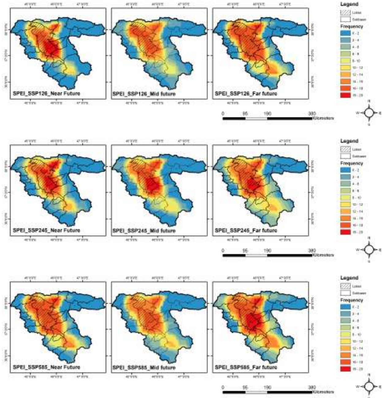
Figure S1. Maps showing SPEI drought frequency over ULB in the near (2021-2040), mid (2041-2060), and far (2081-2100) future under SSP1-2.6, SSP2-4.5, and SSP5-8.5
