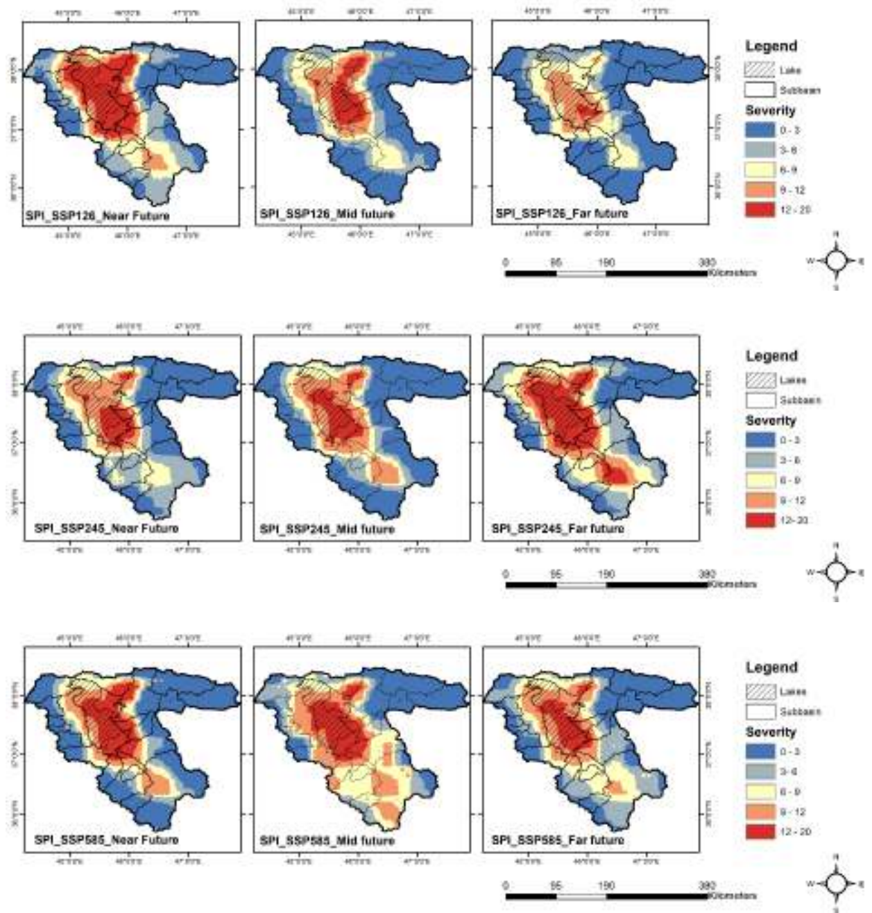
Figure S3. Maps showing SPI drought severity over ULB in the near (2021-2040), mid (2041-2060), and far (2081-2100) future under SSP1-2.6, SSP2-4.5, and SSP5-8.5
