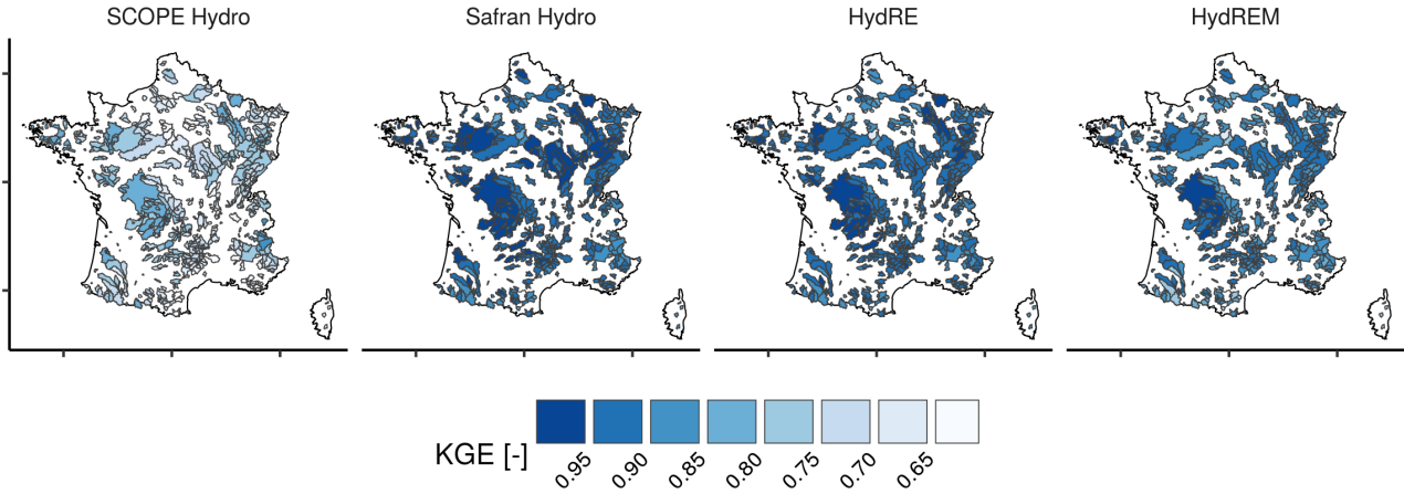
Figure 5. Map of the KGE(\sqrt{Q}) computed during the calibration period 1973–2006 for different hydrological reconstructions. For SCOPE Hydro, HydRE and HydREM the score is computed as the median of 25-member values.
