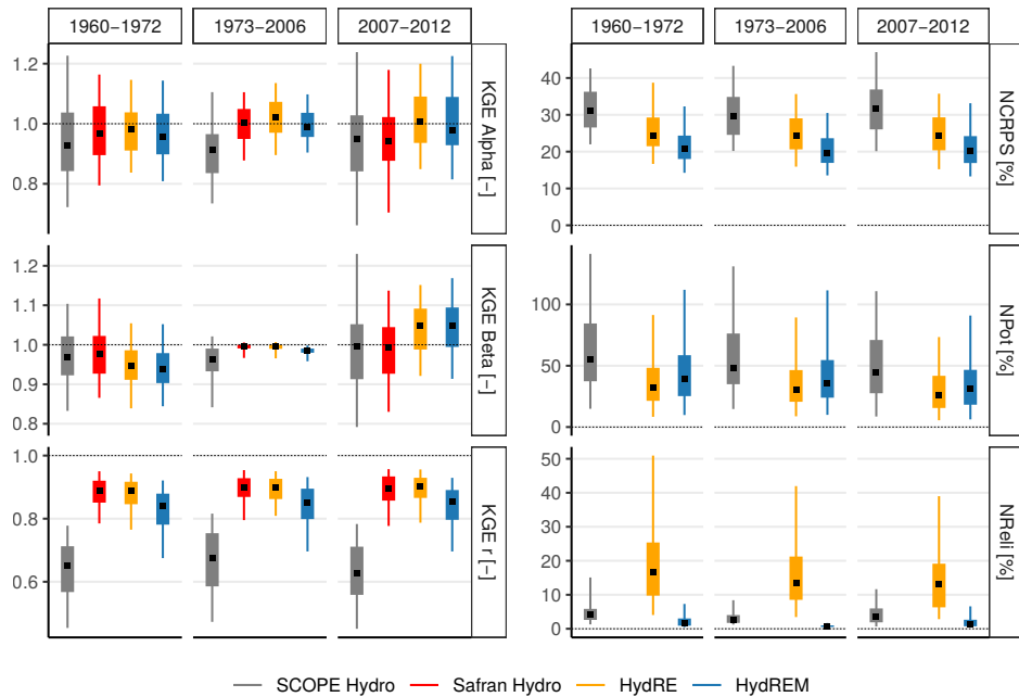
Figure 6. Boxplot of different metrics over 3 distinct periods using 173 stations. For SCOPE Hydro, HydRE and HydREM the score displayed is computed as the median of 25-member metrics. The square correspond to the median, the thick lines to the 25th and 75th quantiles and the narrow lines to the 5th and 95th quantiles. The black dotted lines represent the optimal values for each metrics.
