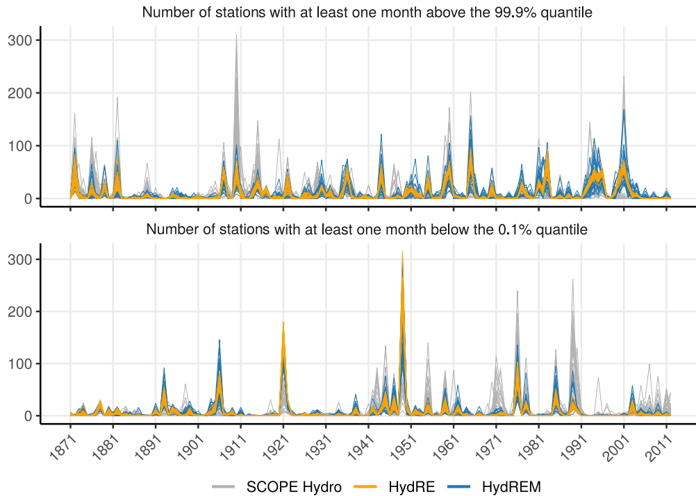
Figure 9. Evolution of the number of stations with at least one monthly streamflow above (below) the 99.9% (0.1%) monthly quantile during a year. This is applied separately for each of the 25 member and the period of reference used to computed the quantile is 1871-2012.
