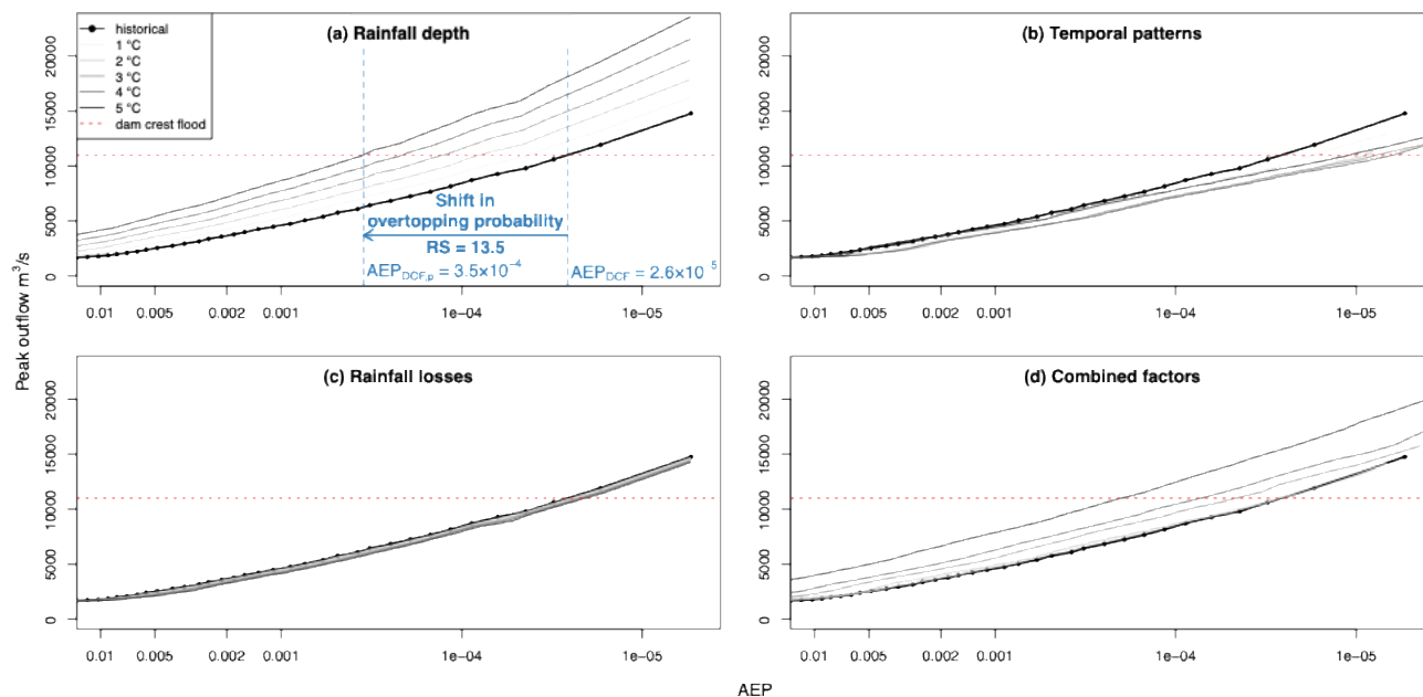
Figure 4 Example of derived outflow flood frequency curves resulting from changes in the flood driver of (a) rainfall depth; (b) temporal patterns; (c) rainfall losses; and (d) a combination of all three flood drivers.
