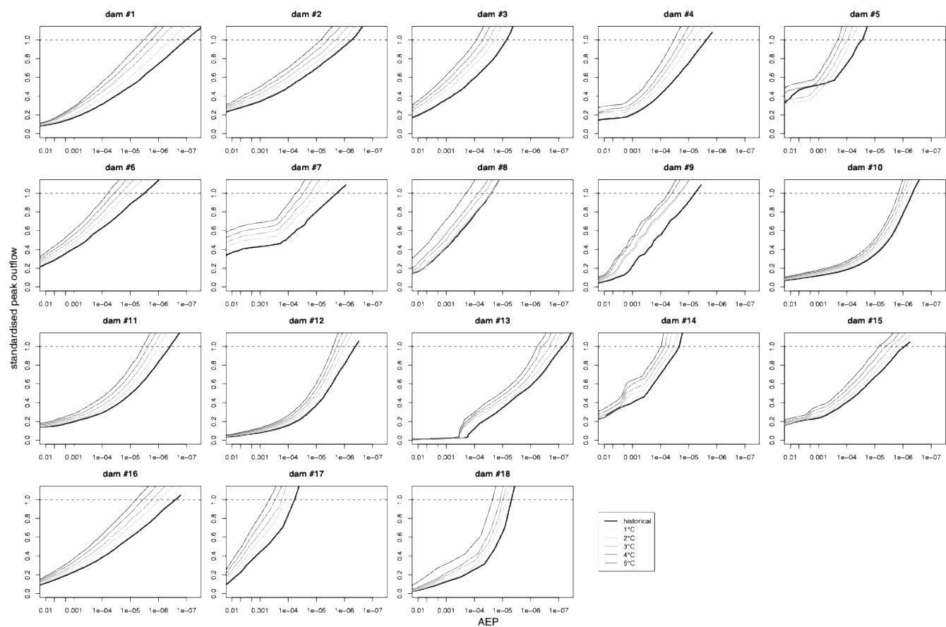
565 Figure C 1. Outflow flood frequency curves for historical conditions and climate change conditions resulting from a combination of all three flood drivers under 1-5°C of global warming. Results anonymised for all 18 dams and outflows are standardised by the dam crest flood.
