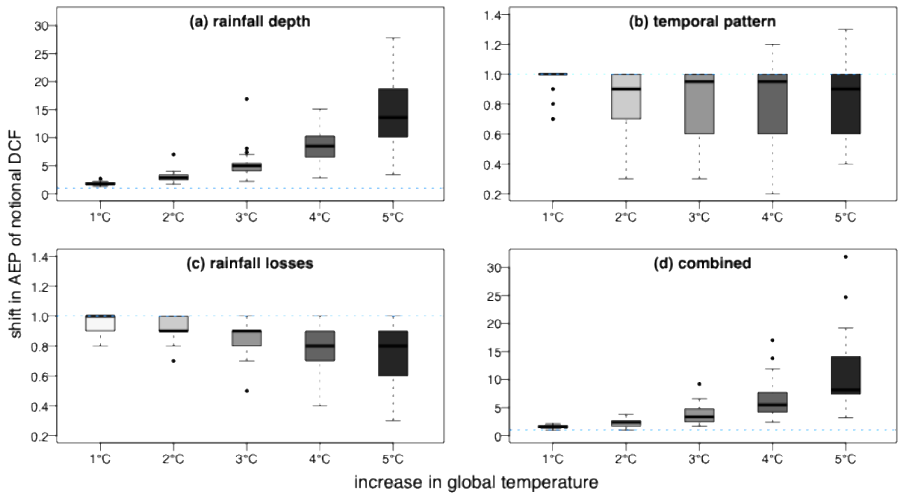
370 Figure 5. Box plots of the relative shift in the annual exceedance probability (AEP) of the dam crest flood (DCF) for all 18 dams resulting from changes in (a) rainfall depth, (b) temporal pattern, (c) rainfall losses, and (d) all three flood drivers combined. Box plots show the median and interquartile range (IQR). Whiskers show the minimum and maximum values that lie within 1.5 times the IQR of the median value. Dashed blue line represents the historical baseline.
