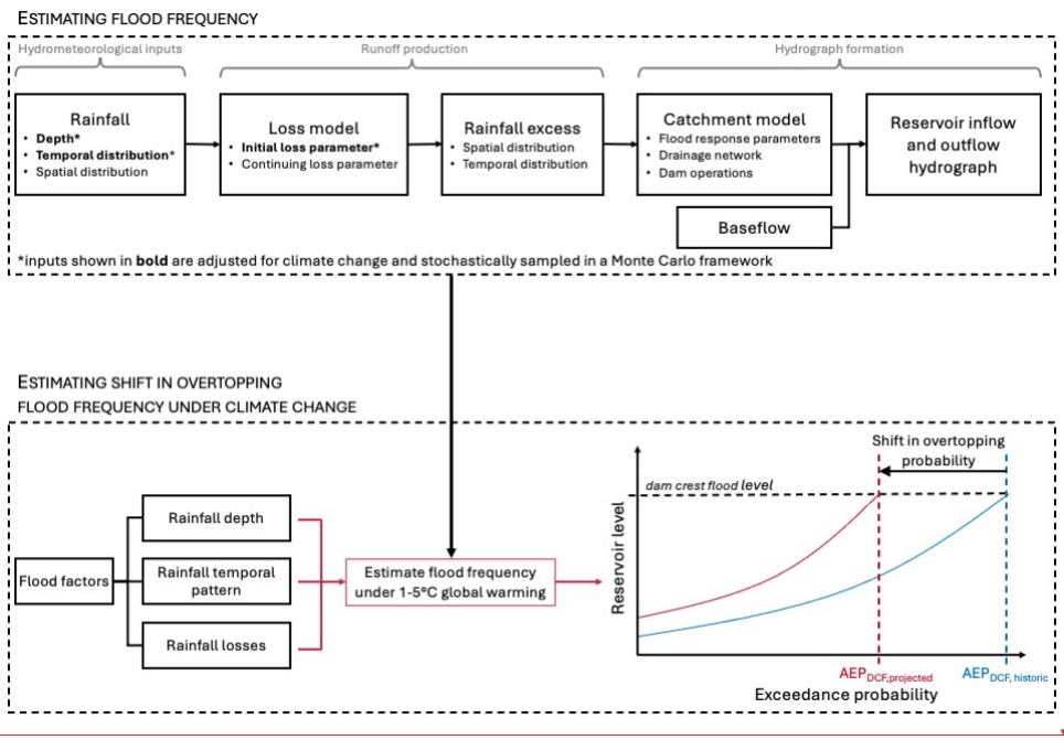
Figure 2: Schematic of event-based flood modelling and flood modelling under climate change.
