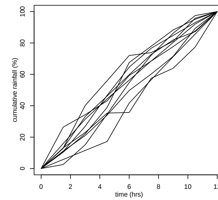
GTSMR coastal_storms 100km 2 12hr
