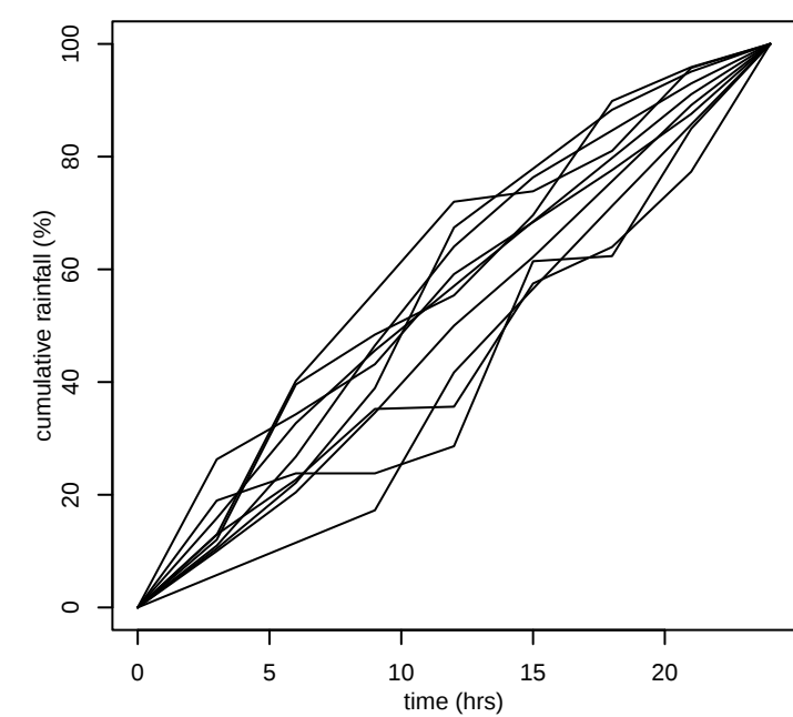
GTSMR coastal_storms 1000km 2 24hr
