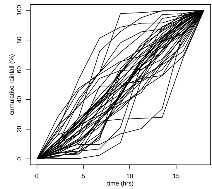
GSAM coastal 2500km 2 18hr
