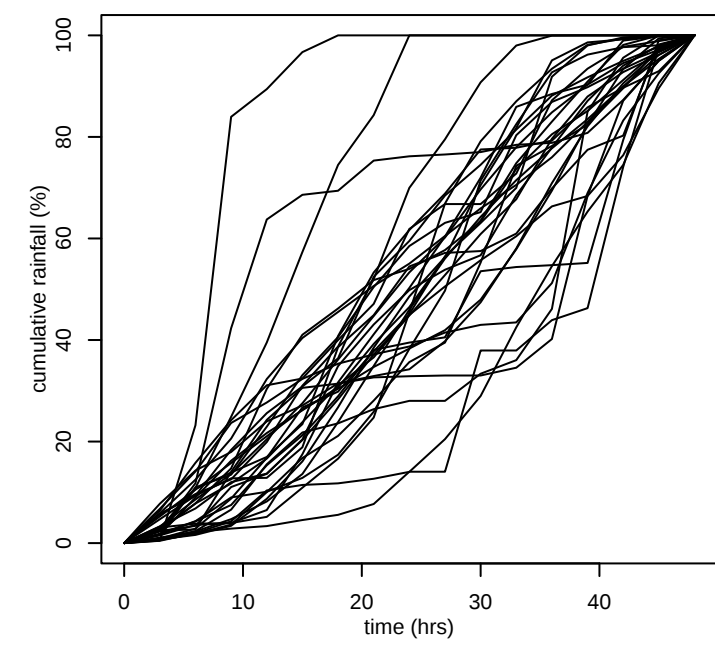
GSAM coastal 100km 2 48hr
