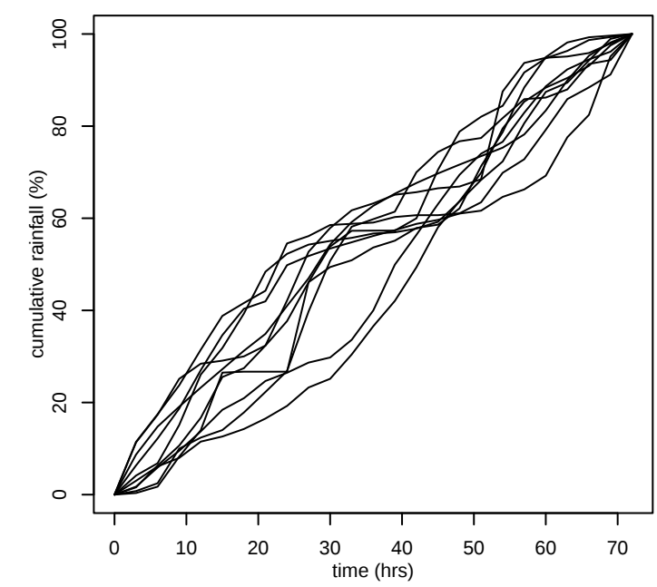
GTSMR coastal_storms 100km 2 72hr
