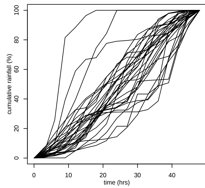
GSAM coastal 500km 2 48hr
