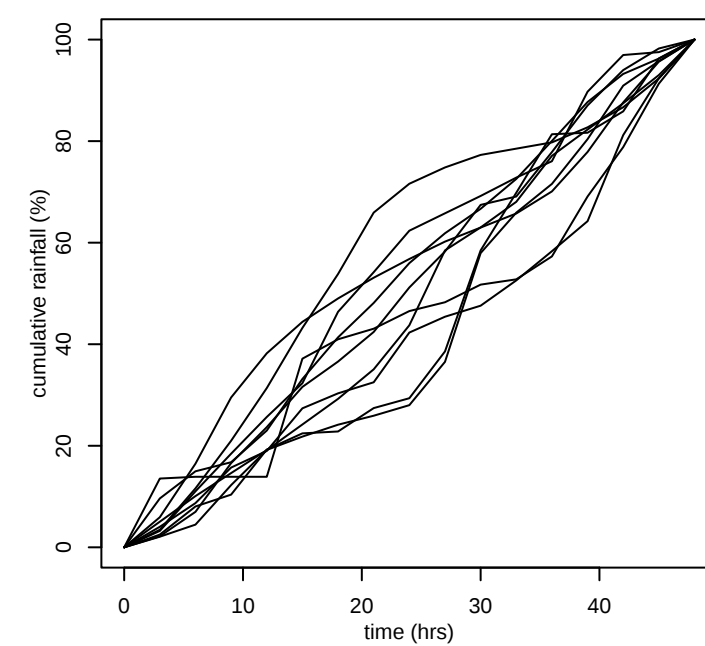
GTSMR coastal_storms 5000km 2 48hr
