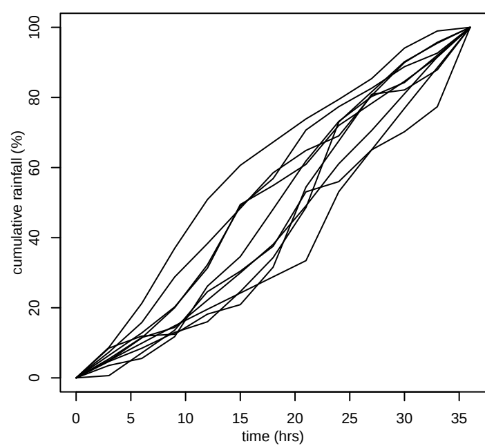
GTSMR coastal_storms 1000km 2 36hr
