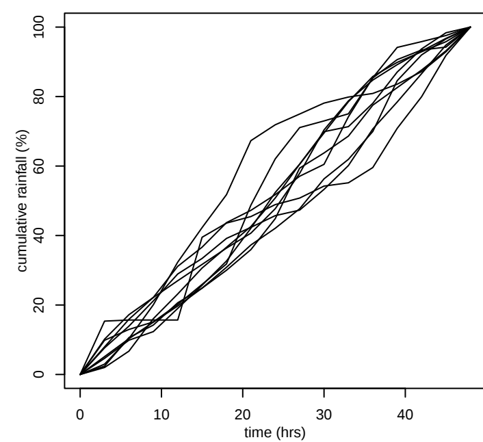
GTSMR coastal_storms 1000km 2 48hr
