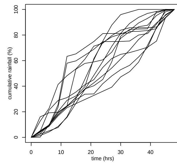
GSAM inland 20000km 2 48hr
