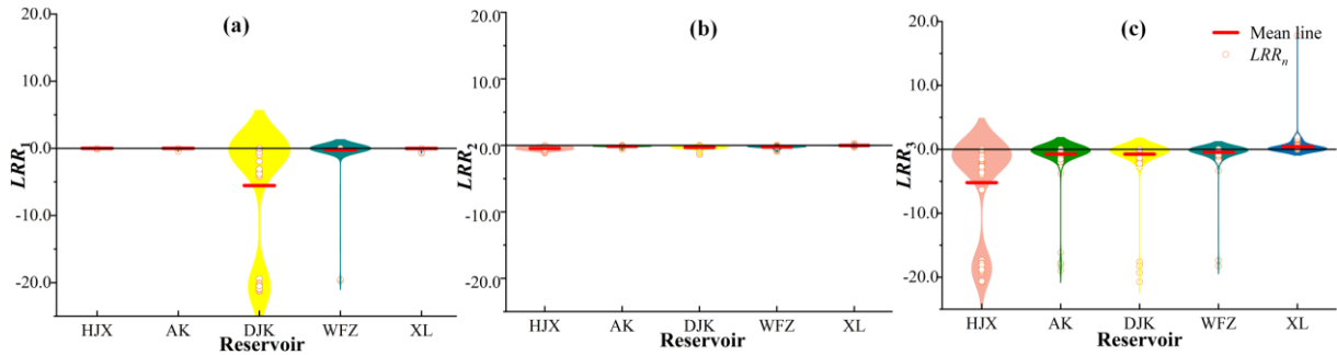
525 Figure 14. the differences of indexes (i.e., (a) LRR_1 , (b) LRR_2 , (c) LRR_3 for log response ratio of the S, H, and E component) between S_{3-4-n} and S_{0-4-n} at the monthly scale.
