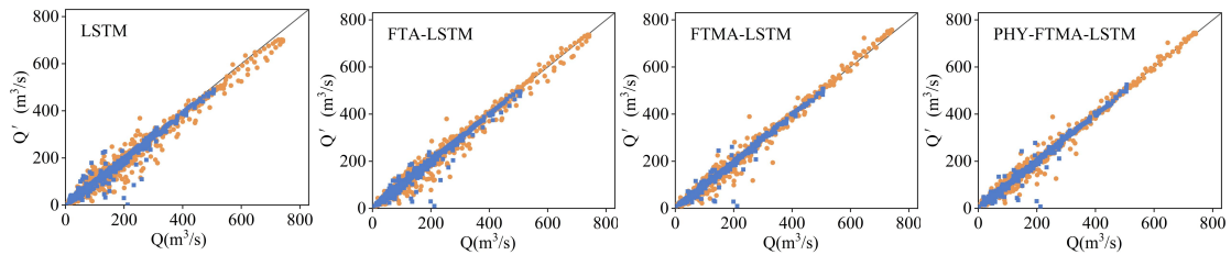
(a) t+1
