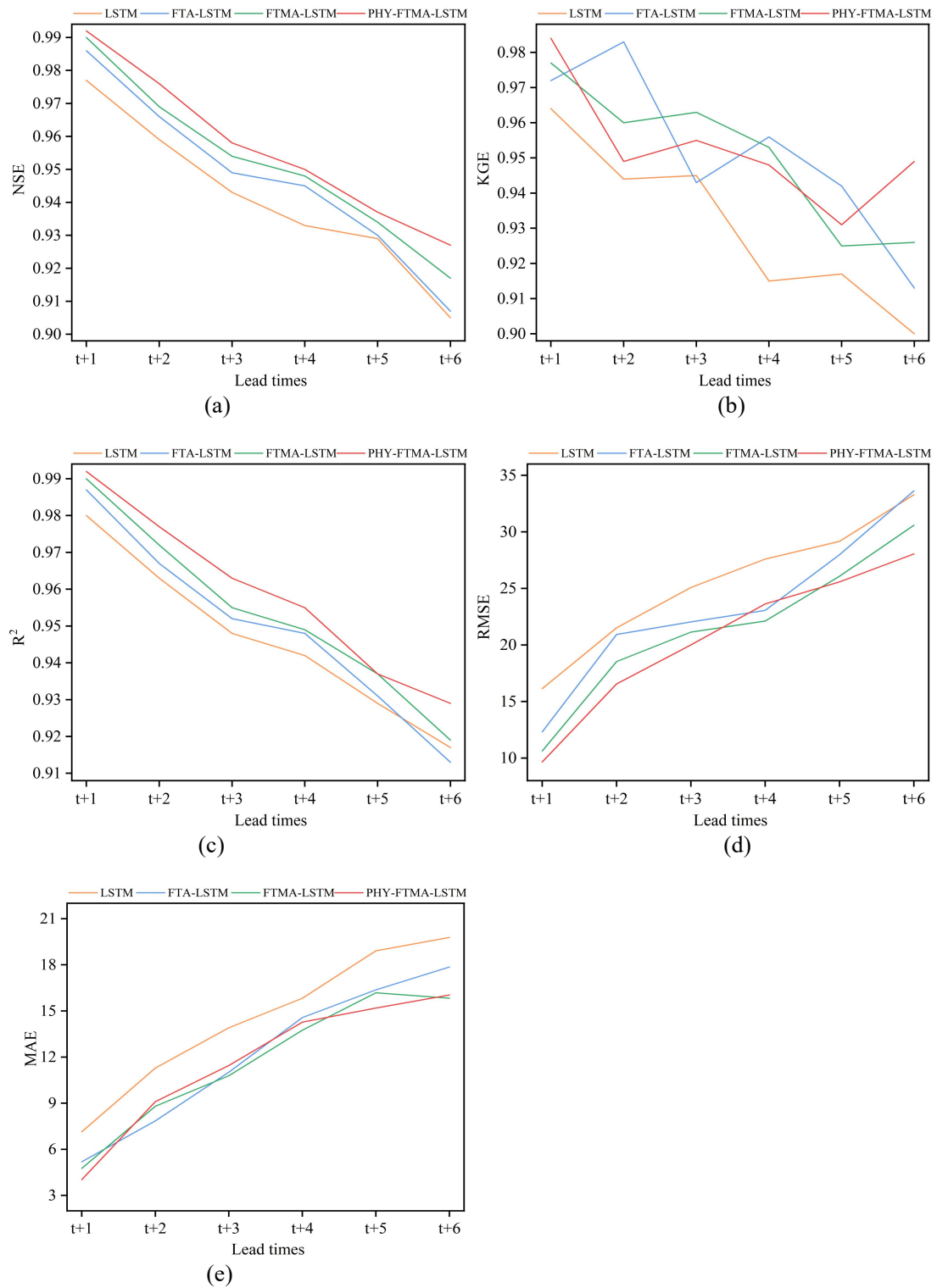
Fig.4. Performance of the four models for flood forecasting at different lead times for training (a) NSE, (b) KGE, (c) R 2 , (d) RMSE and (e) MAE.
