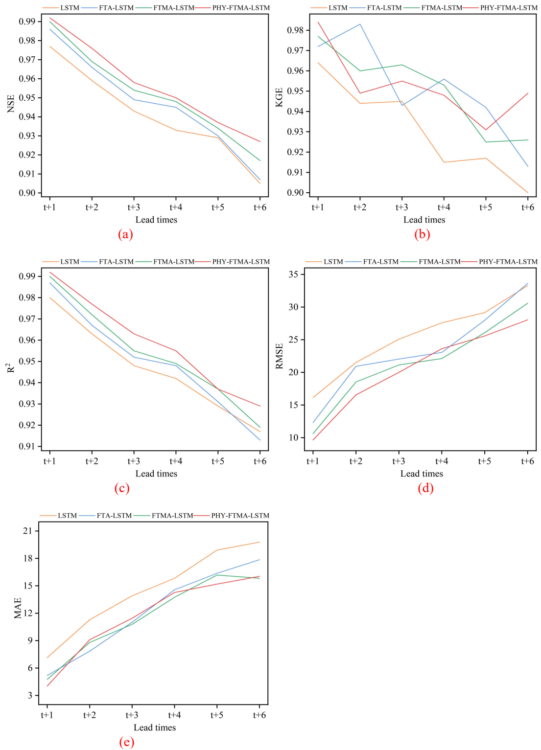
Fig.4. Performance of the four models for flood forecasting at different lead times for training (a) NSE, (b) KGE, (c) R 2 , (d) RMSE and (e) MAE.
