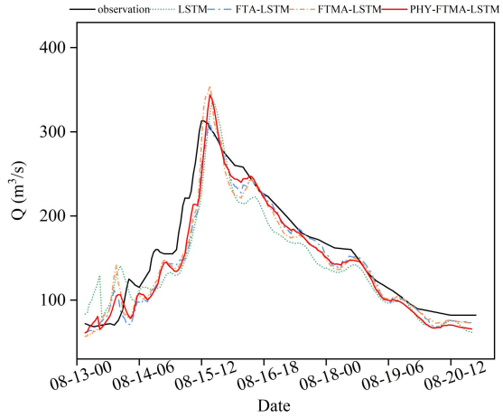
(e) t+5
