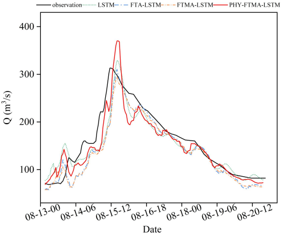
(f) t+6
