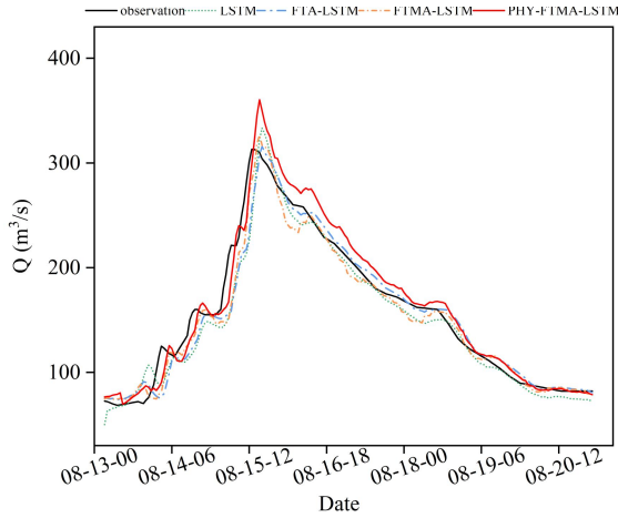
(c) t+3
