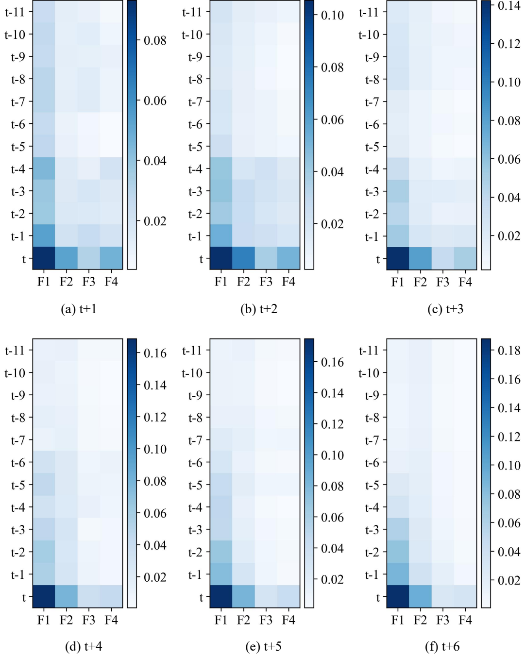
Fig.9. The visualization of feature-time-based attention weights of the PHY-FTMA-LSTM. The X-coordinate variables F1 to F4 represent the input features of runoff, rainfall, evapotranspiration, and initial soil moisture of the watershed, respectively. The Y-coordinate variables represent the input history moments.
