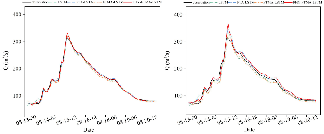
(a) t+1
