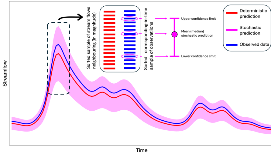
Figure 2: Conceptual illustration of BLUECAT methodology. Blue colour represents observed (streamflow) data, whereas red and pink colours are deterministic and stochastic predictions respectively.
