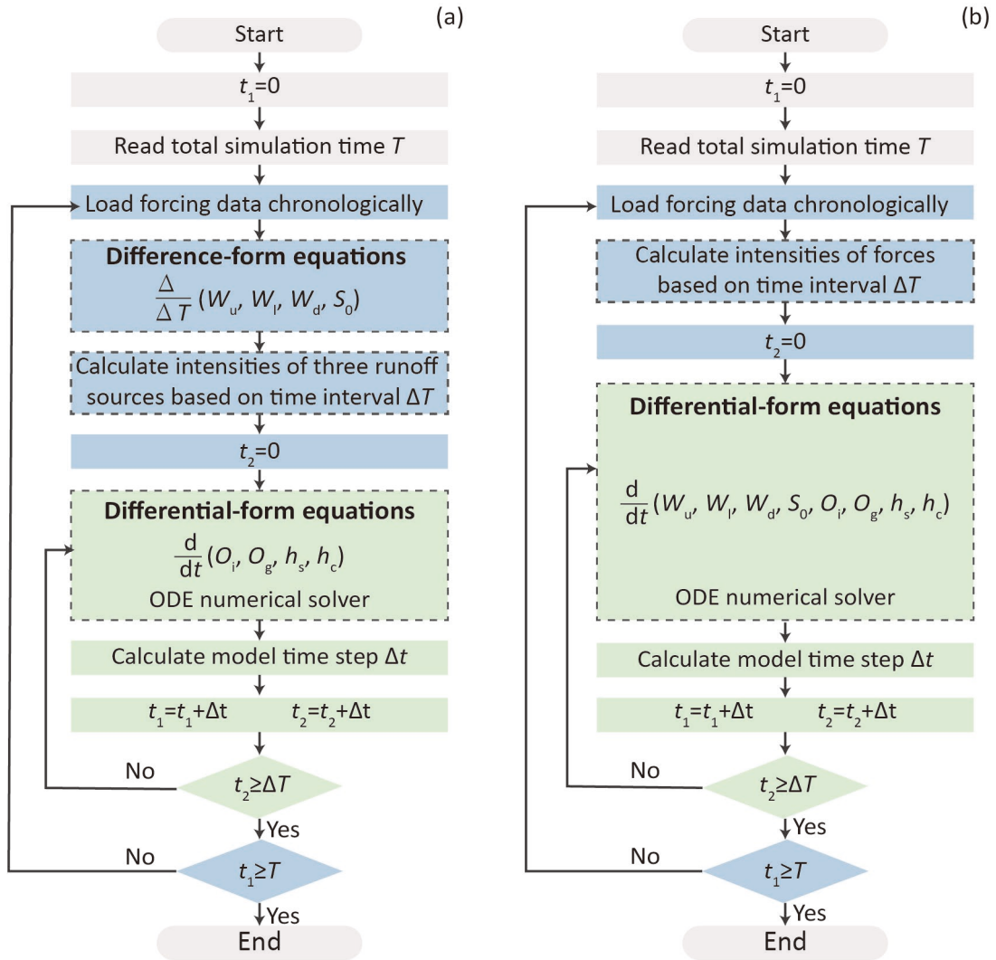
335 Figure 3. Diagram of the loosely-coupled (a) and fully-coupled (b) numerical implementation framework. t_1 and t_2 are two variables to store time. W_u , W_l , W_d , and S_0 are state variables related to runoff generation process, while O_i , O_g , h_s , and h_c are state variables related to runoff concentration process. The differences between the two frameworks are highlighted with dash boxes.
