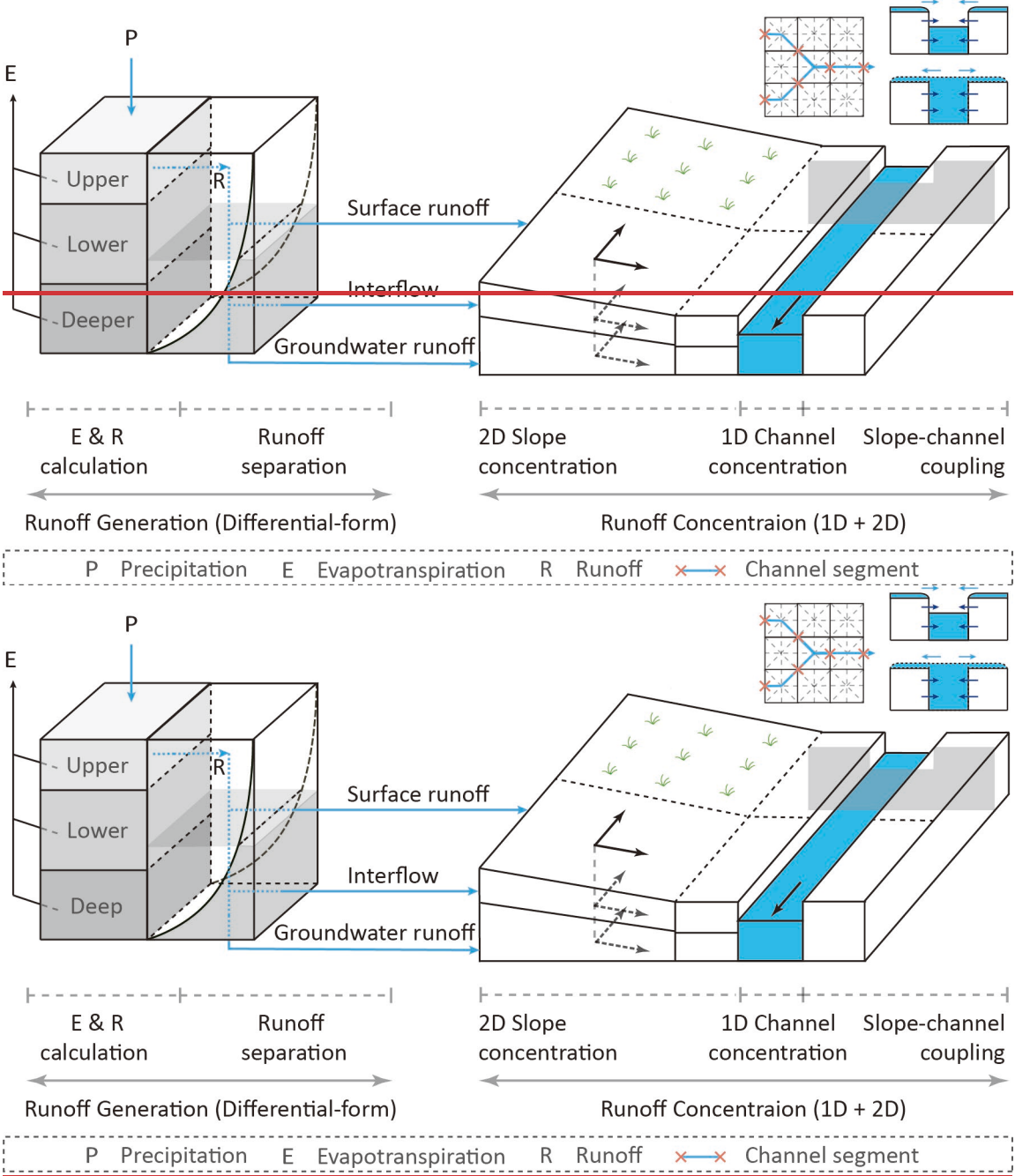
135 Figure 1. Diagram of the two-dimensional differential-form of distributed Xinanjiang model.
