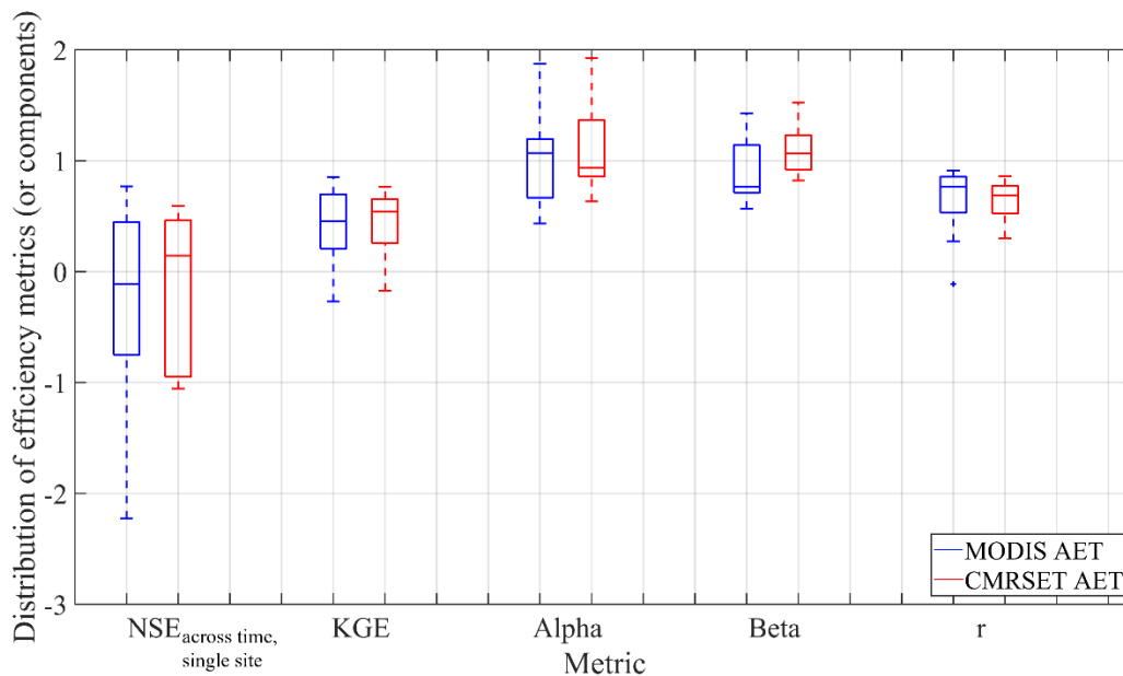
315 Figure 8: Distribution of conventional efficiency metrics, all calculated on a monthly timestep: 1) Nash Sutcliffe efficiency ( NSE_{\text{across time, single site}} ), 2) Kling Gupta Efficiency (KGE), 3) Alpha ( \alpha – ratio of standard deviations), 4) Beta ( \beta – ratio of means), and r (r – Pearson correlation coefficient), calculated using monthly MODIS and CMRSET AET with flux tower AET (Note that there are two outliers not shown in the NSE calculated for MODIS and CMRSET, which are lower than -3).
