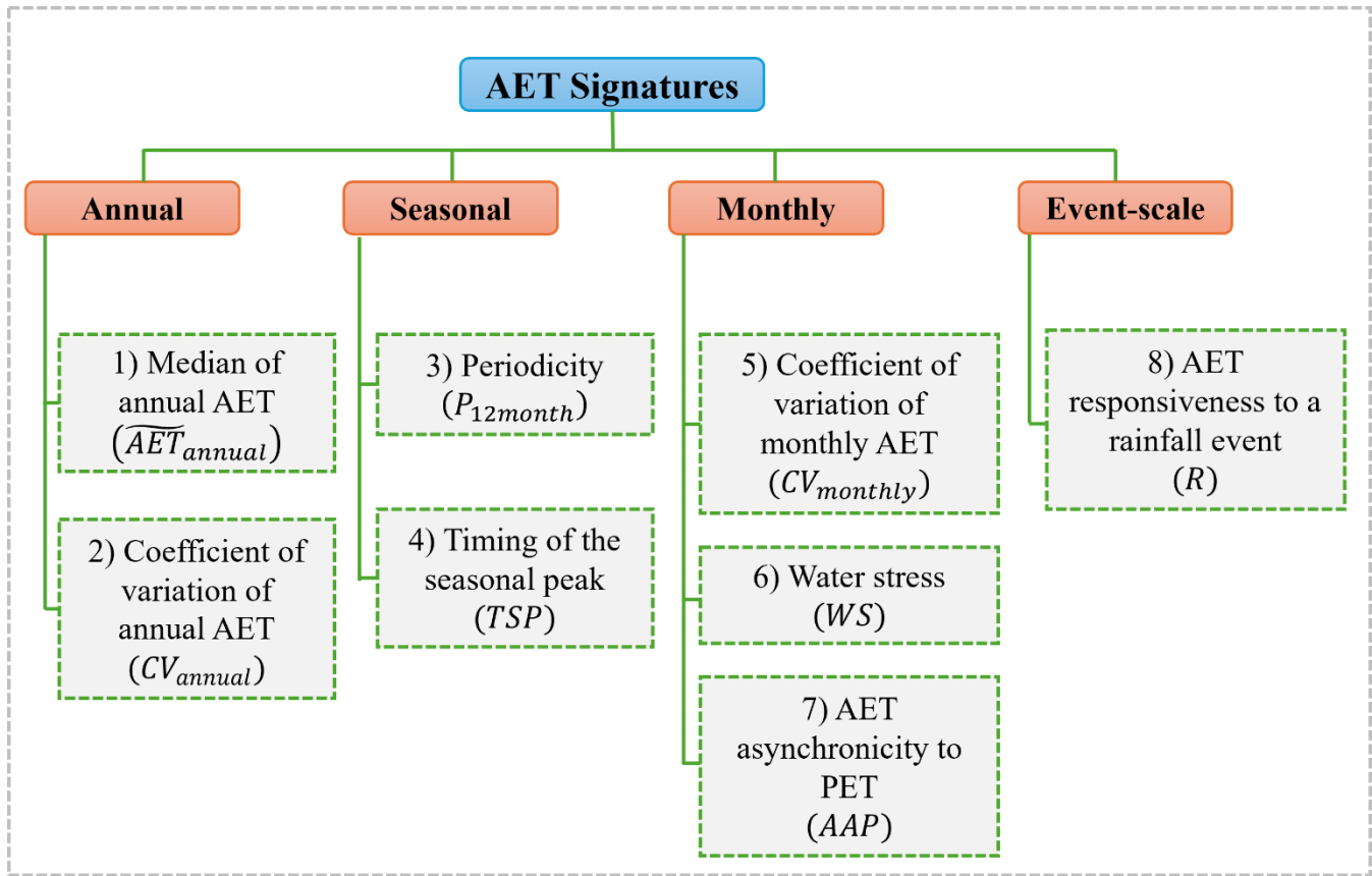
Figure 1: AET signatures.
