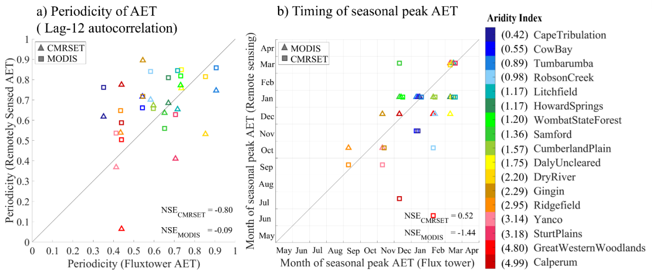
270 Figure 5: Comparison of seasonal AET signatures, a) Periodicity of AET (Lag-12 autocorrelation), b) Timing of seasonal peak, between remotely sensed AET (MODIS and CMRSET AET) and flux tower AET. Note that Figure 5b values take integer values only (i.e., either one calendar month or the next), leading to several points overlying the same plotting position; to make every point visible we subject each point to a jitter (i.e., a unique offset within the same grid cell).
