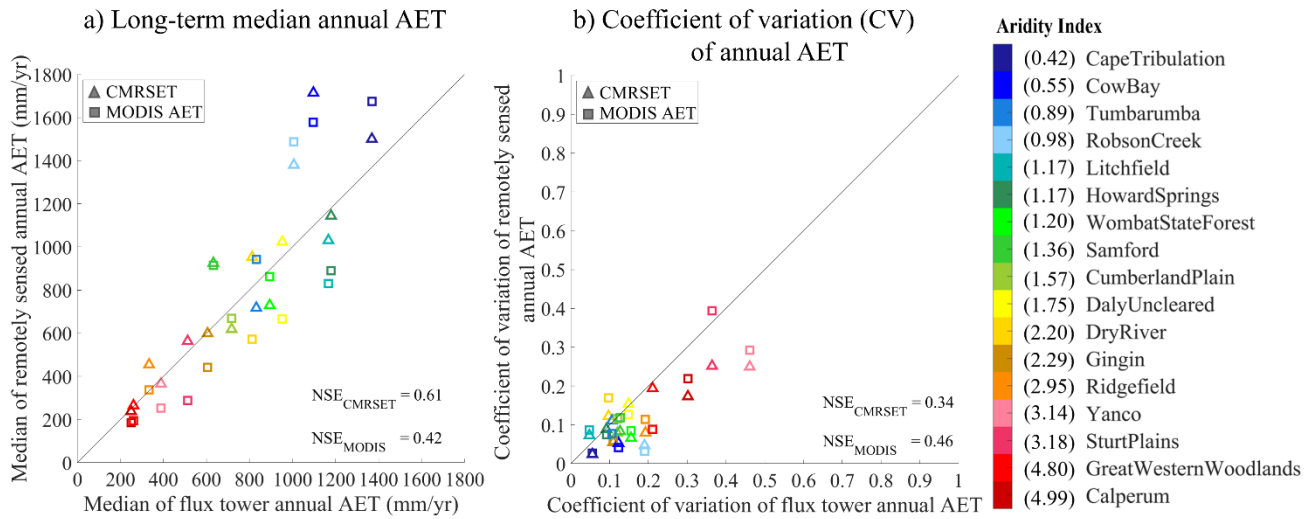
265 Figure 4: Comparison of annual AET signatures; a) Long-term median AET, b) Coefficient of variation (CV) of annual AET, between remotely sensed AET (MODIS and CMRSET AET) and flux tower AET. (Note that the flux towers are ordered by aridity index – from Cape Tribulation (Lowest aridity) to Calperum (Highest aridity)).
