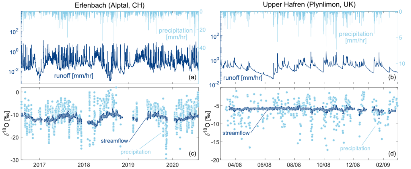
Figure 1. Streamflow (dark blue) and precipitation water fluxes (light blue) as well as oxygen-18 data in streamflow (dark blue) and precipitation (light blue) at Erlenbach (Alptal – a, bc) and Upper Hafren (Plynlimon – eb, d).
