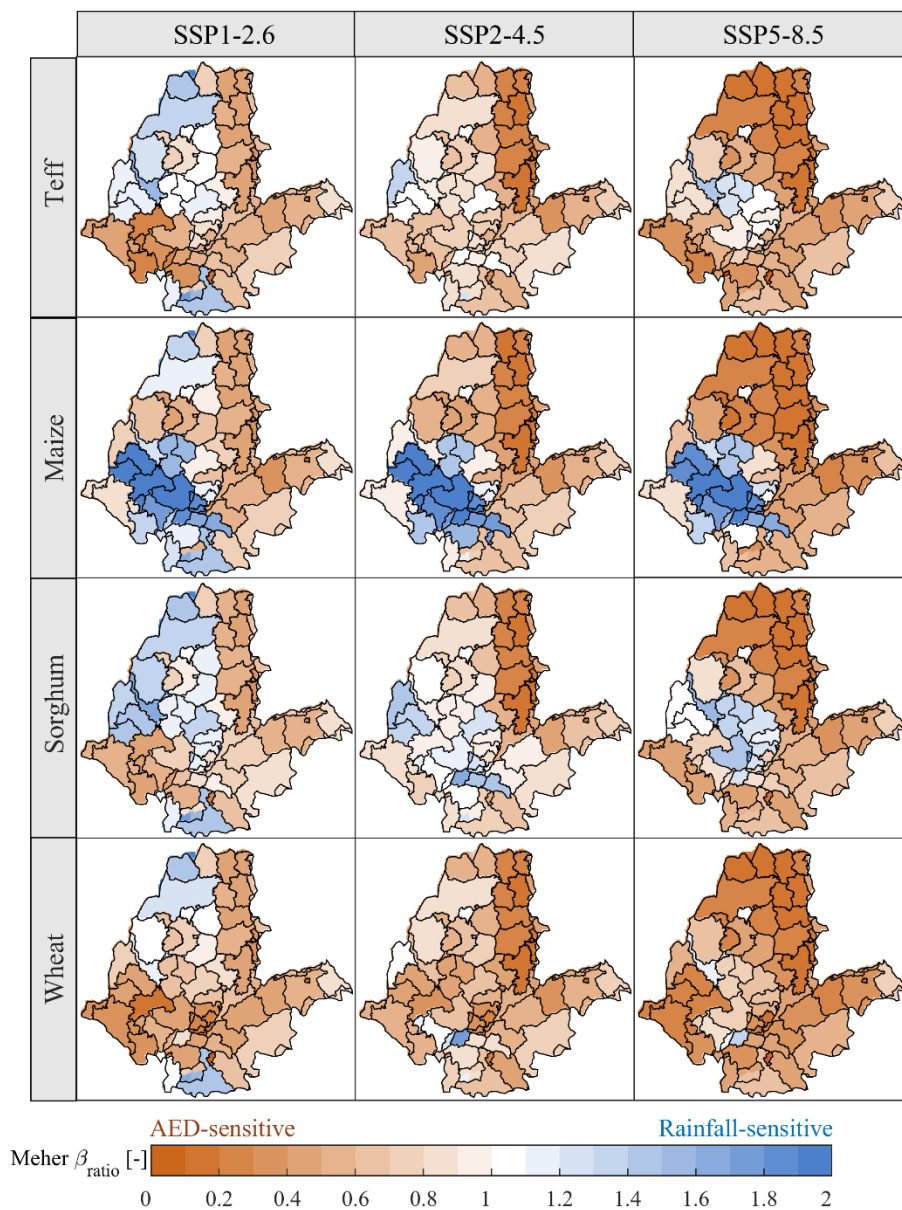
Figure 11: Area-averaged relative sensitivity ( \beta_{\text{ratio}} ) of water-limited attainable yields (AY) to rainfall and atmospheric evaporative demand (AED) for the Meher growing season at the administrative zone level under the low, intermediate, and high emission scenarios. The mapped values represent the average of \beta_{\text{ratio}} of all grid cells within each zone, and all three future periods. The names of the administrative zones are indicated in Figure 1 and Table S1.
