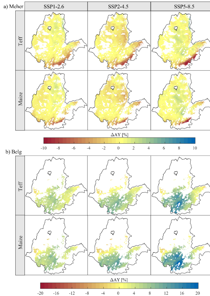
420 Figure 99: Projected changes in water-limited attainable yield for teff and maize in Meher (a) and Belg (b) during the 2060s under the SSP1-2.6, SSP2-4.5, and SSP5-8.5. The RFA region was masked using cropland suitability maps (Wakjira et al., under review) to restrict the analysis to areas potentially suitable for each crop. The non-producing areas during both seasons were also masked out following the Atlas of Ethiopian Rural Socioeconomy (IFPRI and CSA, 2006).
