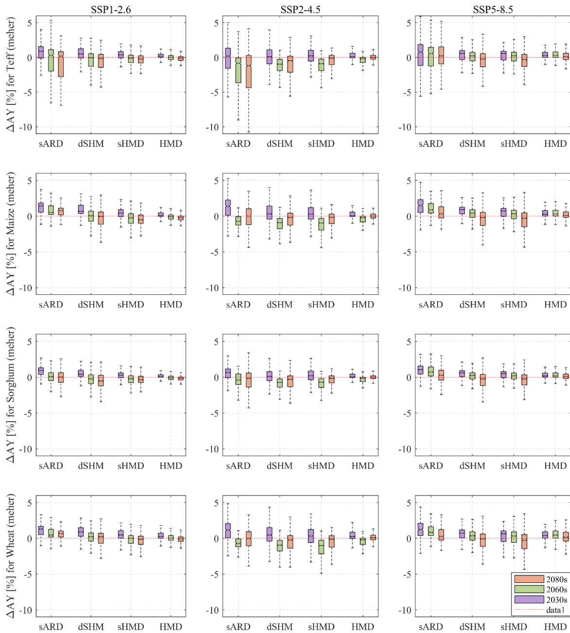
Figure 1010: Boxplots of the projected changes in water-limited yields (AY) of the four major cereal crops produced in Ethiopia in different climatic regimes under the three SSPs during the three future periods, during the Meher growing season. Each boxplot represents the distribution of AY changes within Meher-producing areas for all grid cells in the respective climatic regime. Outlier values have been excluded.
