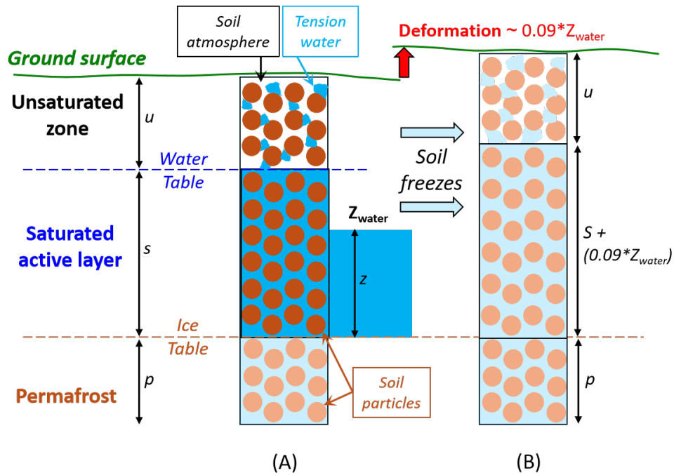
Figure 2. Conceptual diagram of how the depth of saturated water ( z_{water} ) affects soil surface deformation. (A) The summer case when the entire active layer is thawed. Here the soil is divided into three zones: (1) the active layer unsaturated zone (thickness of u ), which contains soil particles (dark circles) and soil atmosphere (white open space). It may also contain tension (capillary) water (shown in light blue); (2) the water-saturated active layer (thickness of s ). The upper surface defines the water table, and the lower surface defines the ice table that separates the thawed active layer from frozen ground (or the permafrost layer at maximum annual thaw depth); and (3) the frozen permafrost (thickness of p ). (B) The winter case when the entire active layer is frozen. Water stored in the saturated active layer leads to frost heave ( 0.09z_{water} ) during freezing. By contrast, water in the unsaturated zone can expand to fill the empty pore space (soil atmosphere) during freezing without contributing to surface deformation (thickness u does not change).
