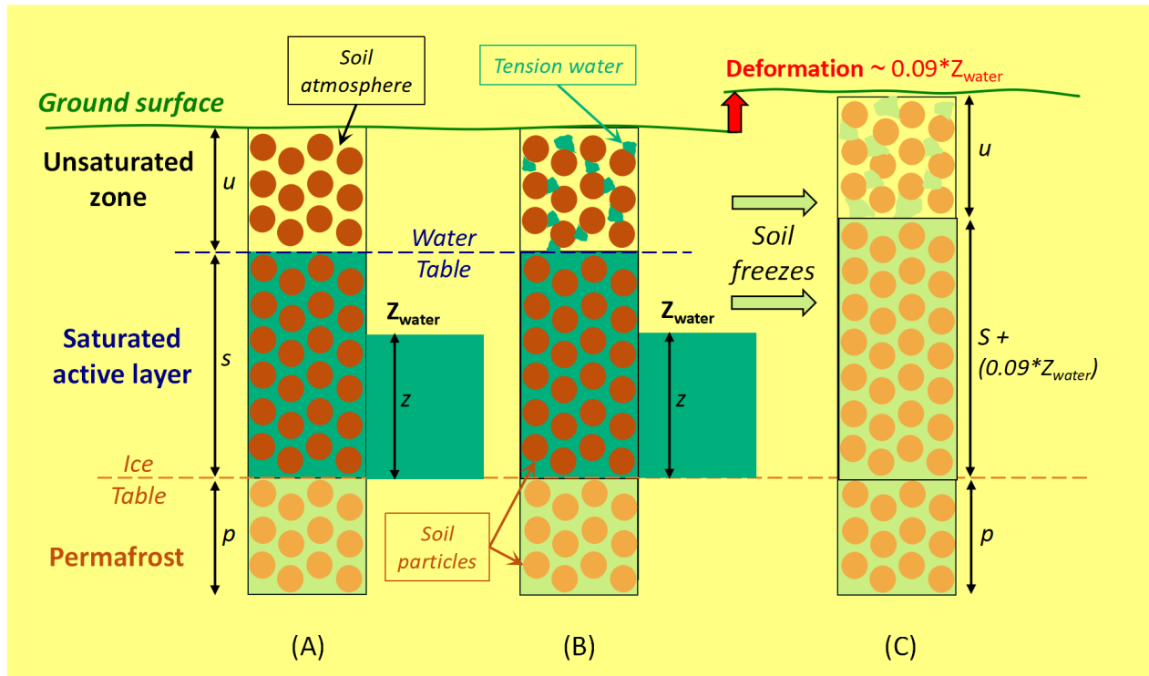
Figure 2. Conceptual diagram of how the depth of saturated water ( z_{\text{water}} ) affects soil surface deformation. The soil is divided into three zones: (1) the active layer unsaturated zone (thickness of u ), which contains soil particles (dark circles) and soil atmosphere (white open space). It may also contain tension (capillary) water (shown in light blue in column (B)); (2) the water-saturated active layer (thickness of s ). The upper surface defines the water table, and the lower surface defines the ice table that separates the thawed active layer from frozen ground (or the permafrost layer at maximum annual thaw depth); and (3) the permafrost (thickness of p ), which may or may not be saturated with water as ice. In column (A), z_{\text{water}} represents the amount of water stored in the saturated active layer. While there is tension water in the upper unsaturated zone in (B), z_{\text{water}} is the same in columns (A) and (B). The reason is shown in (C), where the entire soil column has now frozen. The saturated water freezes and the expansion heaves the soil column above and the ground surface ( s + 0.09z_{\text{water}} ), while the tension water freezes but expands into pores containing soil atmosphere and thus does not contribute to deformation of the ground surface (thickness u does not change).
