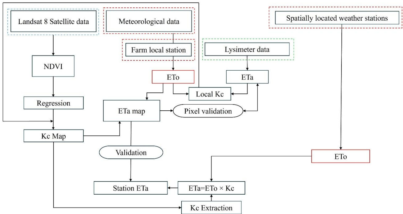
Figure 3. The workflow for VI-ETa algorithm’s actual evapotranspiration estimation and validation. The workflow integrates various steps including data processing, generation of the ETa maps and accuracy validation steps.
