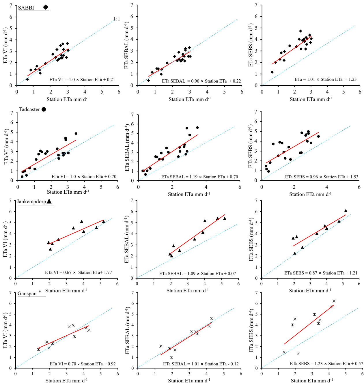
555 Figure 8. Scatter plots between ETa estimated using VI-ET, SEBAL and SEBS algorithms compared to extrapolated ETa on weather stations.
