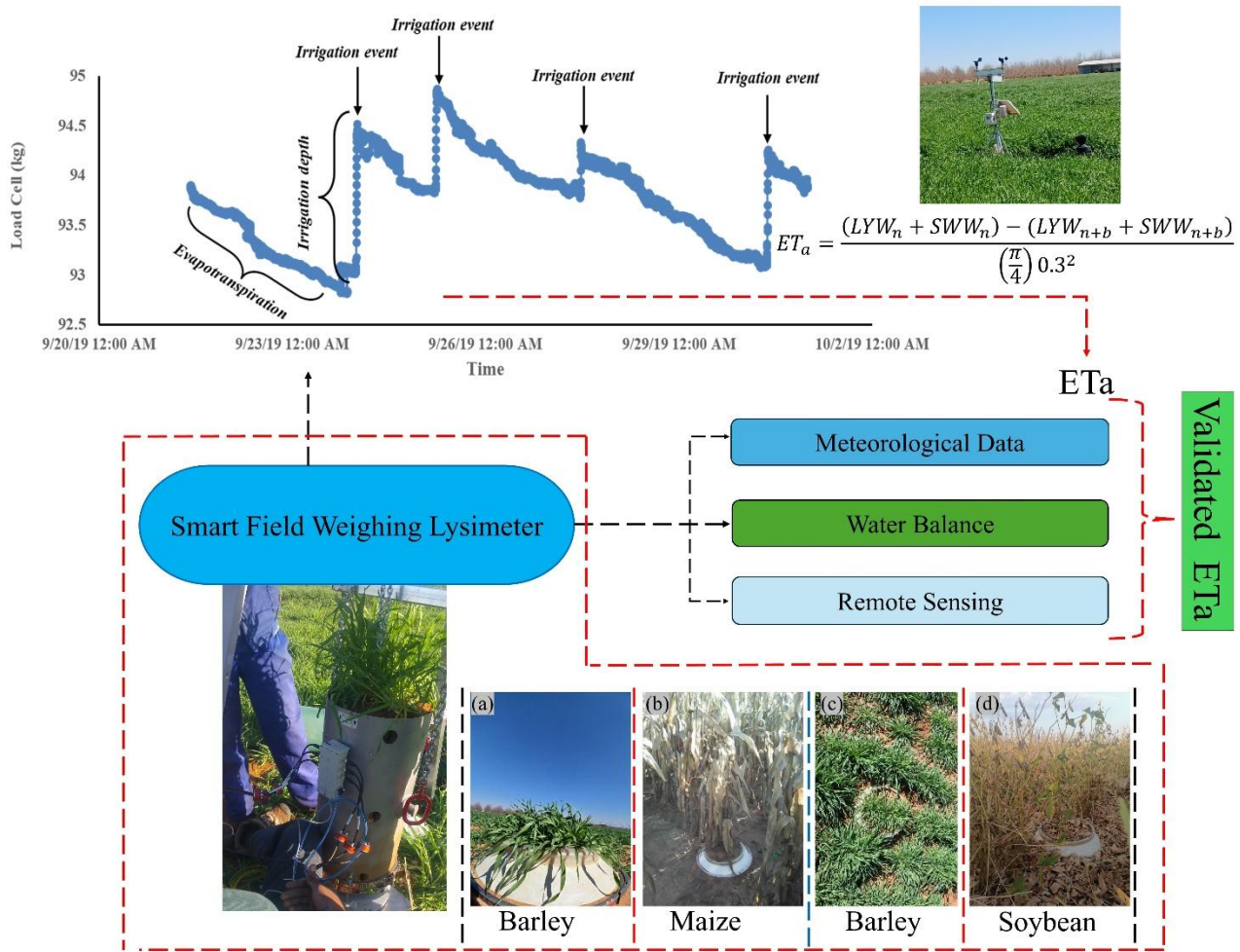
175 Figure 2. Conceptual framework for the study approach linking satellite data and ground measurements.
