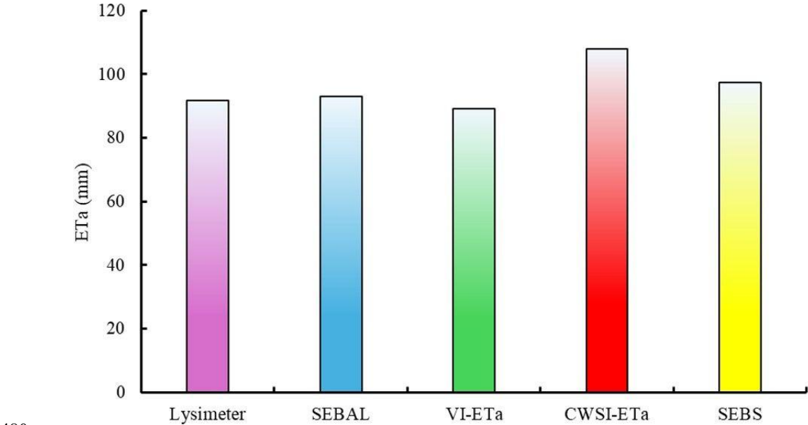
Figure 6. Total lysimeter measured and estimated ETa by SEBAL (blue), VI-ETa (green), CWSI (red) and SEBS (yellow) during the study period.
