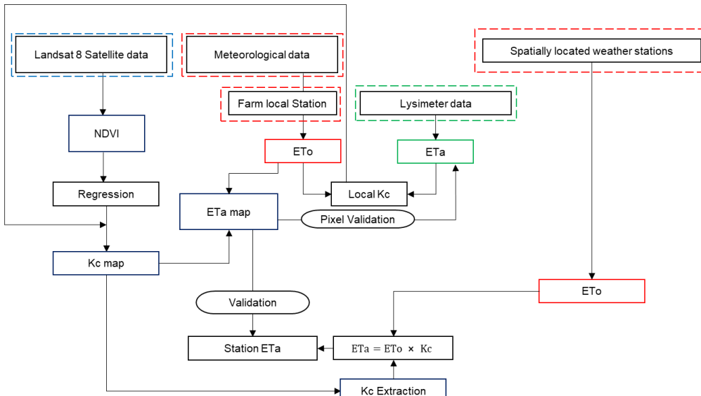
300 Figure 3. The workflow for VI-ETa algorithm’s actual evapotranspiration estimation and validation. The workflow integrates various steps including data processing, generation of the ETa maps and accuracy validation steps.
