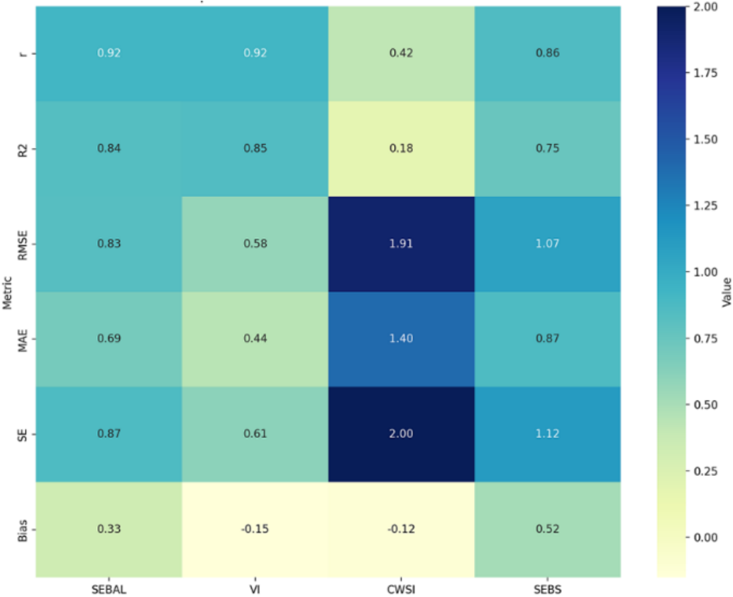
Figure 8. Evaluation best performing algorithms at the experimental site.
