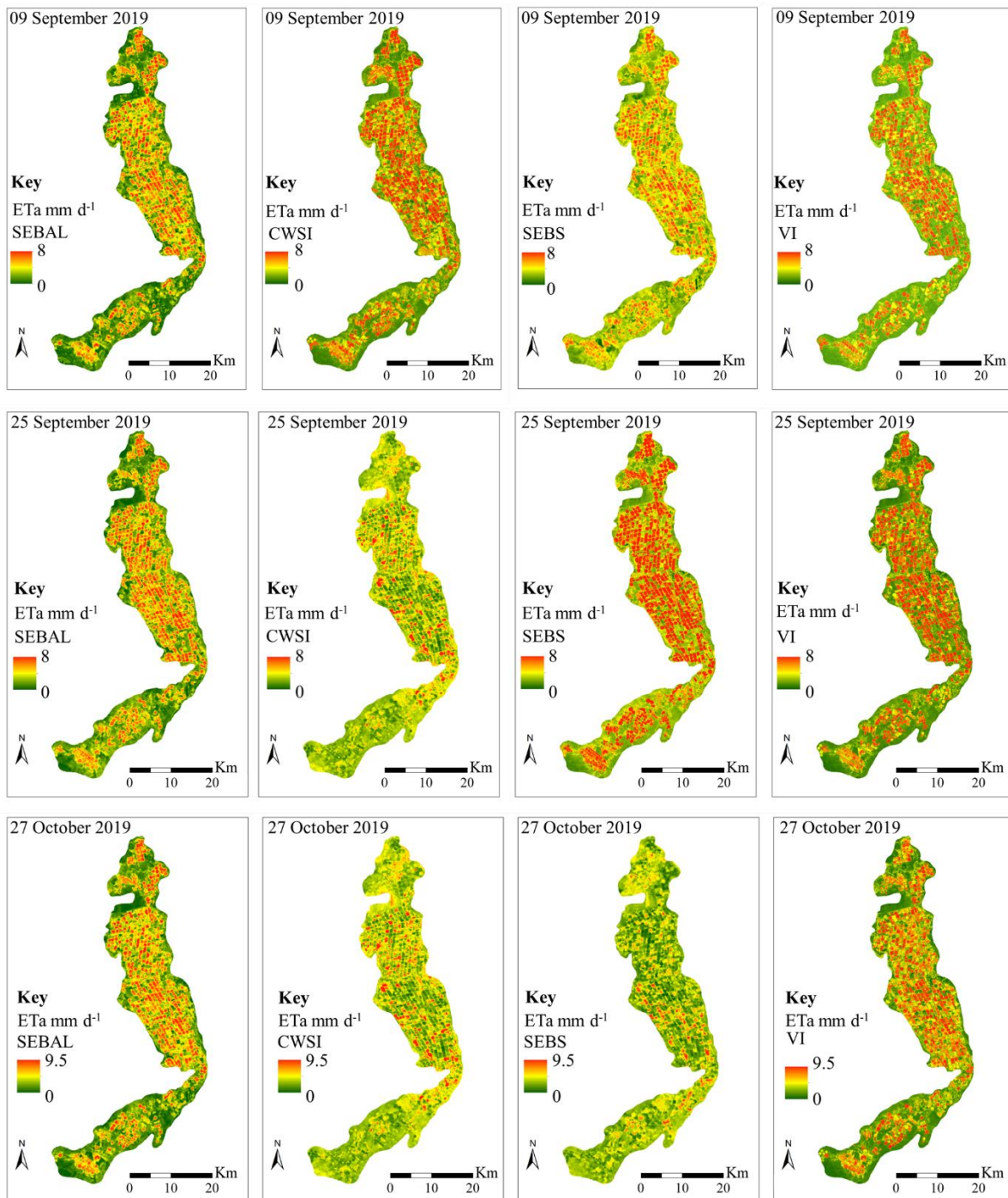
Figure 5. An example of the spatial distribution of ETa within Vaalharts irrigation scheme estimated by SEBAL, CWSI, SEBS and VI-based algorithms for the 9 th of September 2019 to 27 th October 2019.
