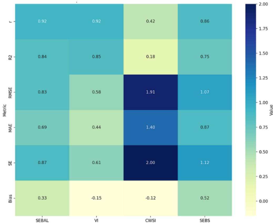
Figure 87. Evaluation best performing algorithms at multi-stations the experimental site .
