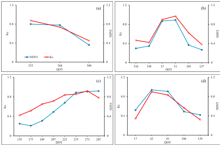
440 Figure 4. The variability of Kc values in relation to the changes in NDVI for the period 2019–2021 where (a) is the winter cropping season in 2019, (b) relates to 2019–2020 summer season, (c) is the 2020 winter season and (d) is the 2021 summer season calculated in the Southern Hemisphere.
