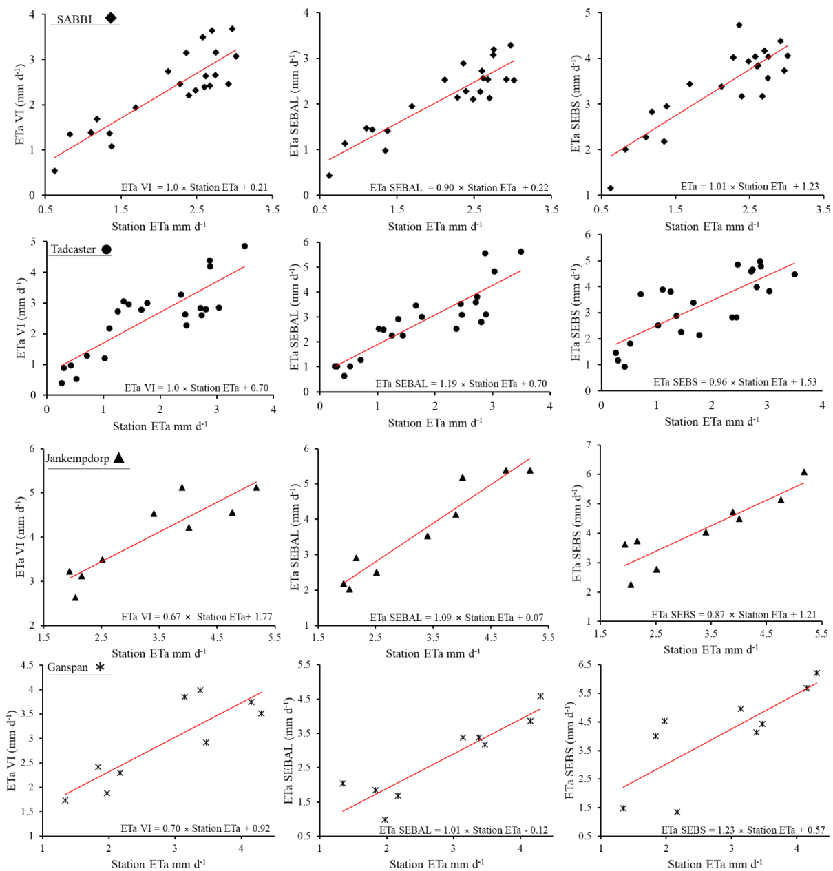
560 Figure 9. Scatter plots between ETa estimated using VI-ET, SEBAL and SEBS algorithms compared to extrapolated ETa on weather stations.
