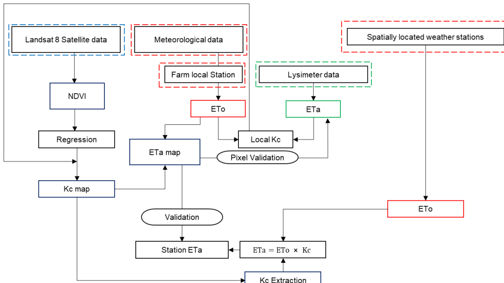
Figure 3. The workflow for VI-ETa algorithm’s actual evapotranspiration estimation and validation. The workflow integrates various steps including data processing, generation of the ETa maps and accuracy validation steps.
