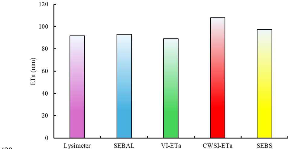
490 Figure 6. Total lysimeter measured and estimated ETa by SEBAL (blue), VI-ETa (green), CWSI (red) and SEBS (yellow) during the study period.
