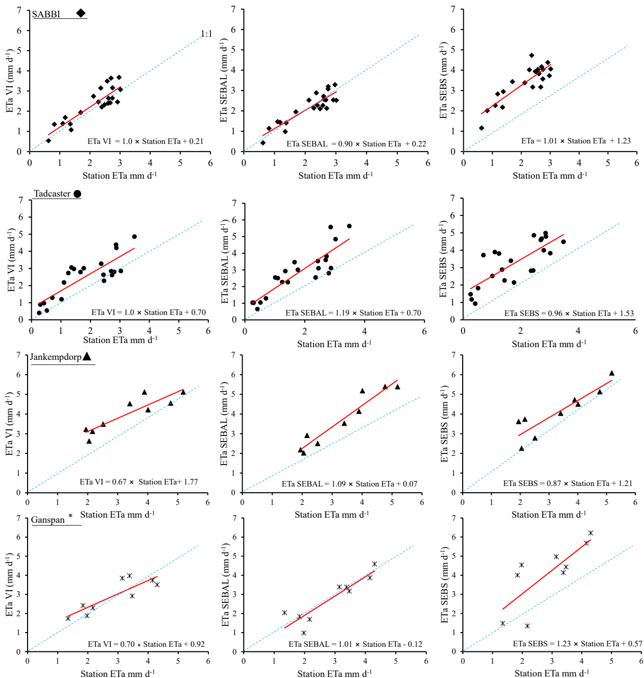
Figure 98. Scatter plots between ETa estimated using VI-ET, SEBAL and SEBS algorithms compared to extrapolated ETa on weather stations.
