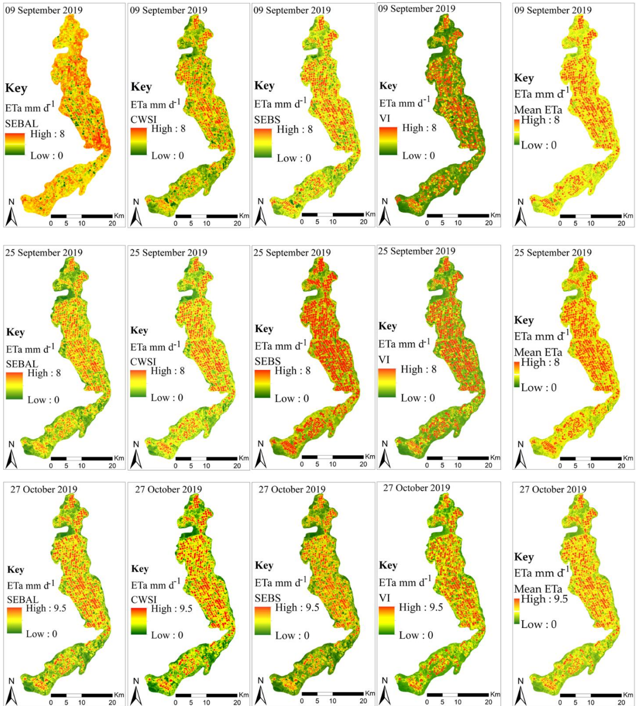
Figure 87. An example of the spatial distribution of ETa within Vaalharts irrigation scheme estimated by SEBAL, CWSI, SEBS and VI-based algorithms for the 9 th of September 2019 to 27 th October 2019.
