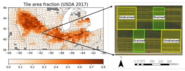
430 Figure 4: Tile fractions over the U.S. Midwest region, and the location and layout of the selected experiment field. The yellow boxes represent sub-fields without tile drainage, and the green boxes represent sub-fields with conventional drainage.
