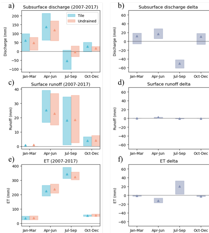
Figure 8: Ecosys-simulated water fluxes under tile and undrained conditions from 2007 to 2017. a) Boxplot of the quarterly net subsurface discharge (subsurface discharge - subsurface recharge); b) Boxplot of the quarterly net subsurface discharge difference between tile and undrained conditions; c) Boxplot of the quarterly surface runoff; d) Boxplot of the quarterly surface runoff difference between tile and undrained conditions; e) Boxplot of the quarterly ET; f) Boxplot of the quarterly ET difference between tile and undrained conditions. The upper and lower parts of the boxplots indicate 25% and 75% quantiles, and the boxes indicate the interquartile variation. The triangles indicate the mean values. Delta is the difference between tile and undrained conditions. The corresponding monthly results are shown in Fig. S10.
