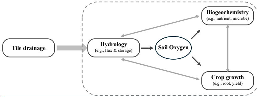
Figure 1: Hypothesis on how tile drainage impacts hydrology, soil biogeochemistry, and crop growth. Tile drainage directly changes field hydrology, and then changes soil biogeochemistry and crop growth. Among those, soil oxygen is a key mediator that links hydrology, soil biogeochemistry and crop growth in the coupled system.
