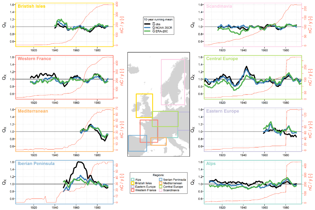
315 Figure 9: 10-year running means of the QX observations (black) and simulations (blue: NOAA 20CR simulations, green: ERA-20C simulations) for each region studied. Only years with at least 10 available catchments per region are considered. The red y axis shows the number of available catchments per year and region.
