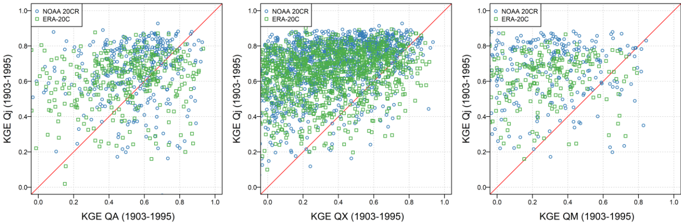
FigureB: Comparison between simulation performance of mean- (left), high- (center), and low-flow (right) simulations (smoothed over 10 years) and the performance of simulations of daily streamflows.
