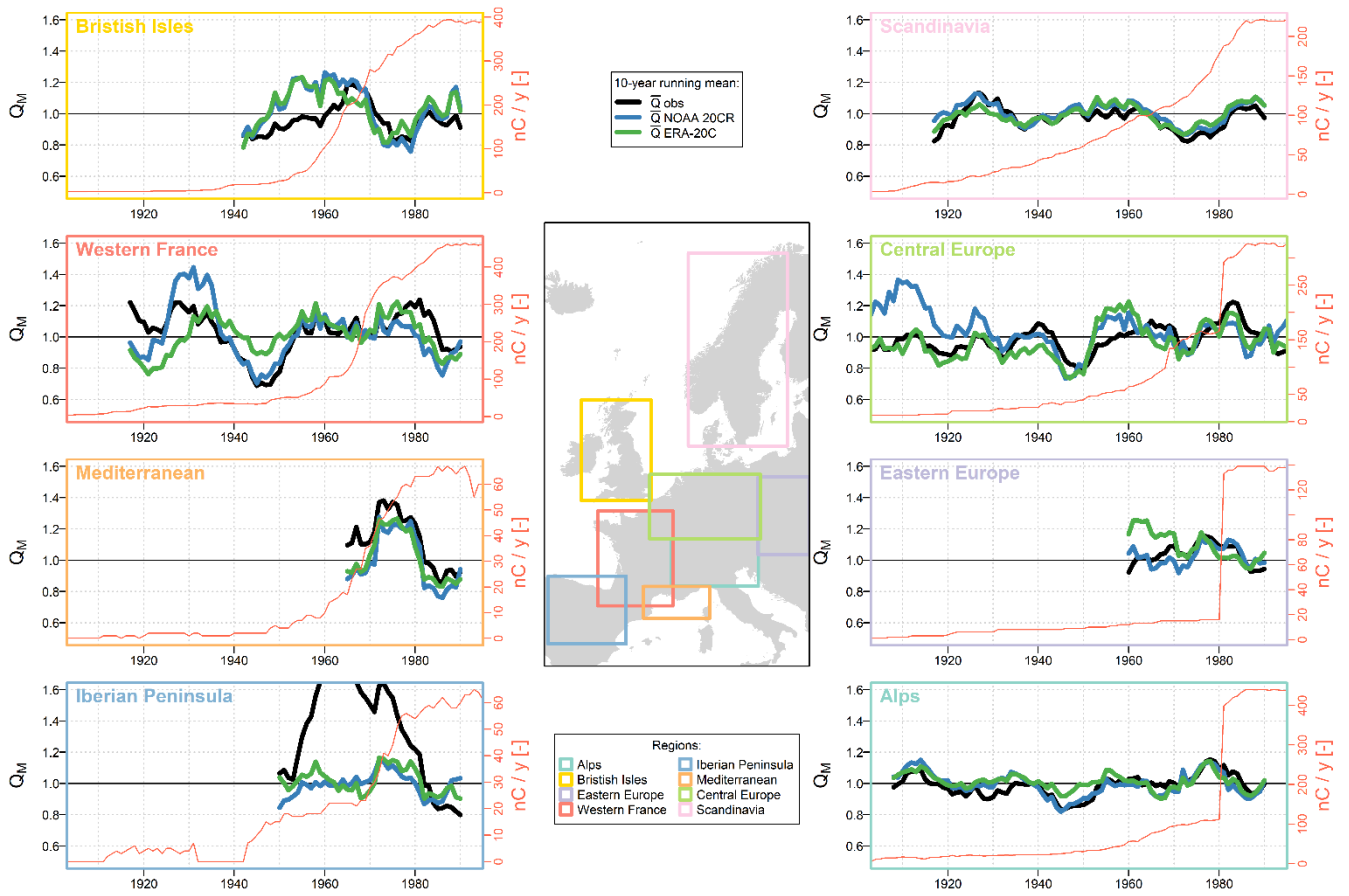
310 Figure 8: 10-year running means of the QM observations (black) and simulations (blue: NOAA 20CR simulations, green: ERA-20C simulations) for each region studied. Only years with at least 10 available catchments per region are considered. The red y axis shows the number of available catchments per year and region.
