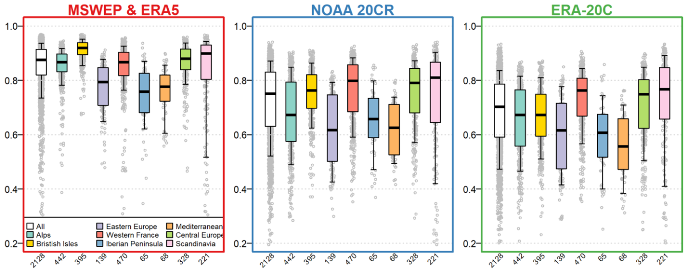
250 Figure 3: Calibration performance (KGE) for three different climate forcings (MSWEP & ERA5, NOAA 20CR, and ERA-20C, from left to right) according to region. Boxplots are constructed with the 0.10, 0.25, 0.50, 0.75, and 0.90 quantiles.
