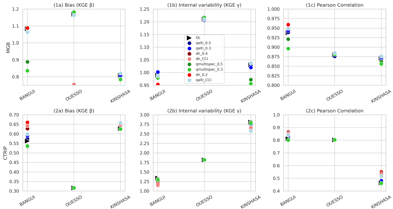
Figure 14. Comparison of bias (KGE \beta ), internal variability (KGE \gamma ), and Pearson correlation for different assimilation experiments in MGB and CTRIP models: daily scores at Ouesso, Bangui, and Kinshasa stations.
