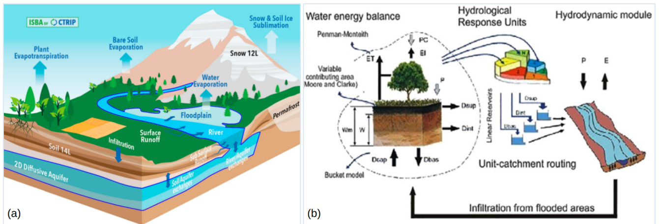
Figure 1. Schematic representation of the two large-scale hydrological models used in this study. Panel (a) illustrates the ISBA-CTRIP model (Decharme et al., 2019a), a global river routing model coupled to the ISBA land surface model, which simulates river discharge at continental scale. Panel (b) presents the MGB model (Collischonn et al., 2007; Pontes et al., 2017), a semi-distributed hydrological model incorporating two-way coupling between hydrology and hydrodynamics, enabling the explicit simulation of floodplain processes such as evapotranspiration from inundated areas.
