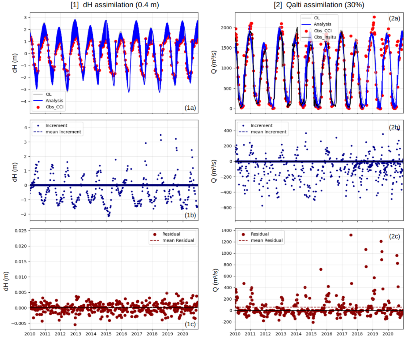
Figure 9. Comparison of dH and Q assimilation at Ansongo, Niger, over the 2010-2020 period: Top panels show time series of (a) dH assimilation with 0.4m uncertainty and (b) Qalti assimilation with 30% uncertainty, with open-loop, analysis, and observed data. The middle and lower panels show the corresponding innovation and residuals, with the mean innovation and residuals represented by dashed lines, illustrating the model’s performance and adjustments after assimilation.
