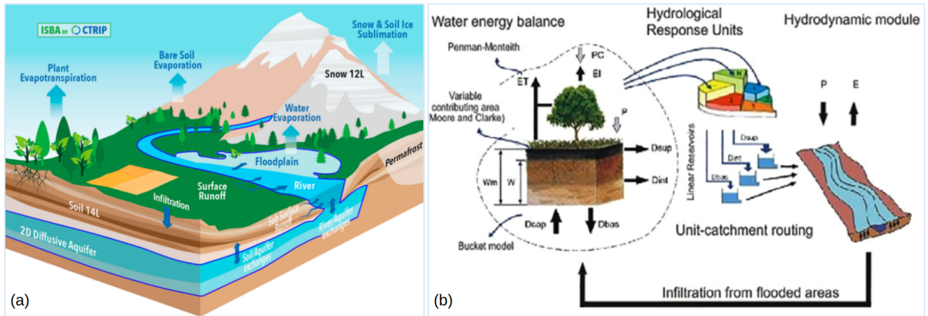
Figure 2. Schematic representation of the two large-scale hydrological models used in this study. Panel (a) illustrates the ISBA-CTRIP model (Decharme et al., 2019), a global river routing model coupled to the ISBA land surface model, which simulates river discharge at continental scale. Panel (b) presents the MGB model (Collischonn et al., 2007; Pontes et al., 2017), a semi-distributed hydrological model incorporating two-way coupling between hydrology and hydrodynamics, enabling the explicit simulation of floodplain processes such as evapotranspiration from inundated areas.
