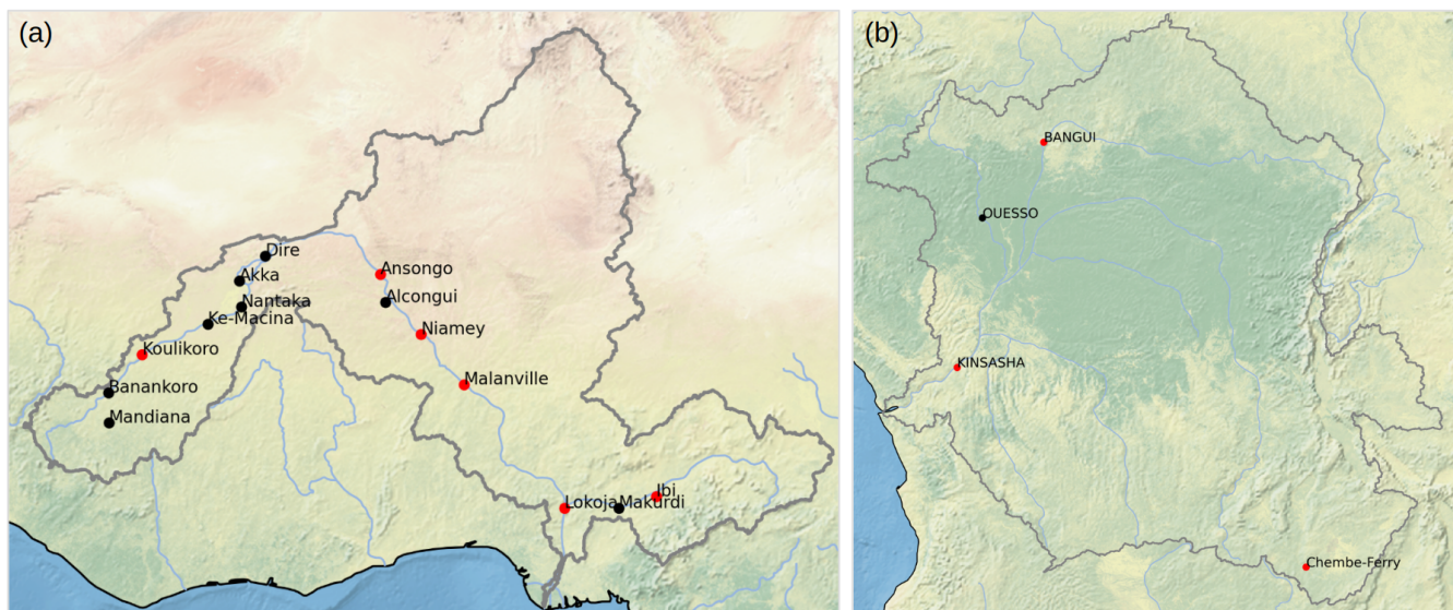
Figure 1. Maps showing the locations of stations in both the Niger and Congo basins. Red markers represent stations where data assimilation is conducted, and black markers indicate the remaining stations with in-situ data used for performance assessment of the assimilation experiments in both the MGB and CTRIP models.
