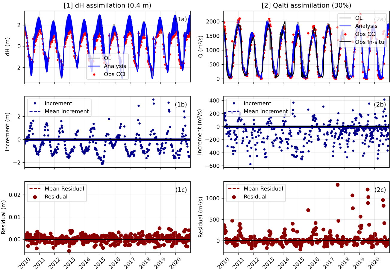
Figure 9. Comparison of dH and Q assimilation at Ansongo, Niger, over the 2010-2020 period, within MGB-HYFAA : Top panels show time series of (a) dH assimilation with 0.4m uncertainty and (b) Qalti assimilation with 30% uncertainty, with open-loop, analysis, and observed data. The middle and lower panels show the corresponding innovation and residuals, with the mean innovation and residuals represented by dashed lines, illustrating the model’s performance and adjustments after assimilation.
