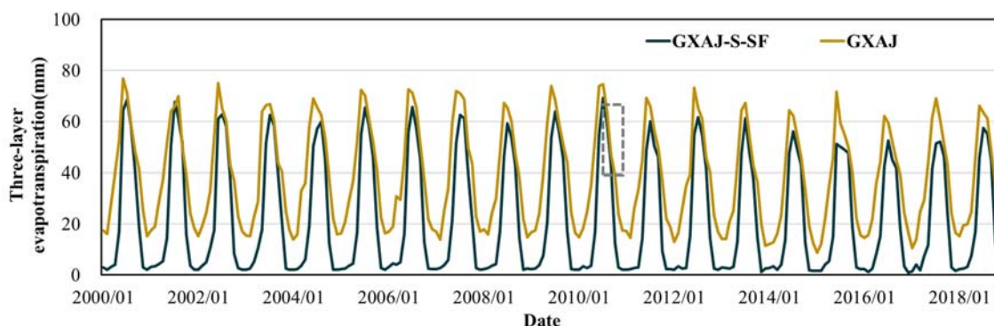
Figure 11. Simulated monthly evapotranspiration series during the study period. The dashed rectangle
