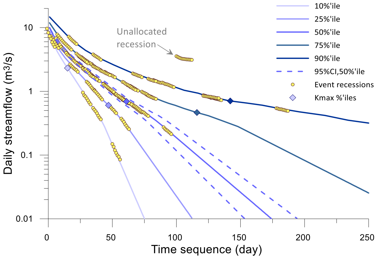
Figure 3 Comparison of daily MRCs computed using a constant bin correlation method with observed recessions during rainless periods for Gibbo River at Gibbo Park (401217). Three rainless days were required before data were acceptable in the analysis. The computed recessions are for five percentile values: 10%, 25%, 50%, 75% and 90%. Maximum recession constants are located in the figure. The 2.5% and 95.5% confidence limits (CL) for the 50% MRC estimated using bootstrapping are also included. One acceptable recession was not allocated to one of the five MRCs.
