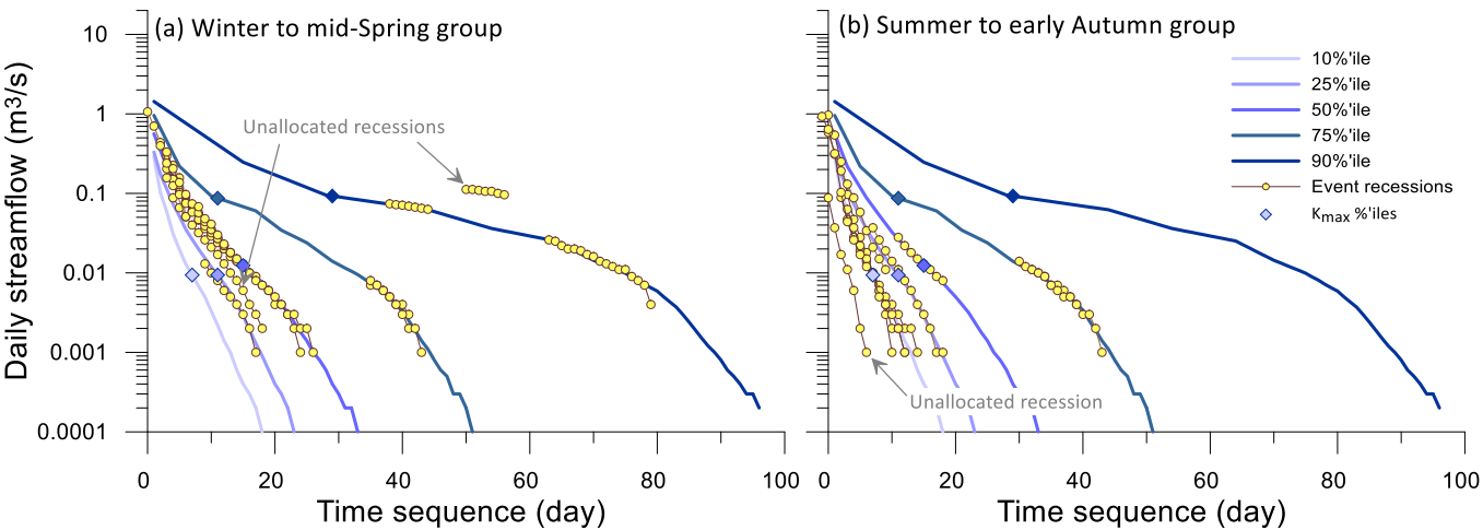
370 Figure 5 Comparison of computed daily MRCs for Northern Arthur River at Lake Toolibin Inflow (609010) with observed recessions during rainless periods for (a) winter to mid-spring and (b) summer to early autumn seasons. In both plots, the computed recessions are the same, based on all available data. Three rainless days were required before data were acceptable in the analysis. The recessions are for five percentile values: 10%, 25%, 50%, 75% and 90%. Maximum recession constants are shown in the figure. 375 Three acceptable recessions were not allocated to one of the five MRCs.
