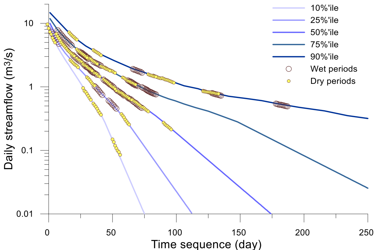
300 Figure 4 Comparison of observed daily recessions for data drawn separately from the wet 6-months and dry 6-months periods superimposed on the estimated MRCs for Gibbo River at Gibbo Park (401217).
