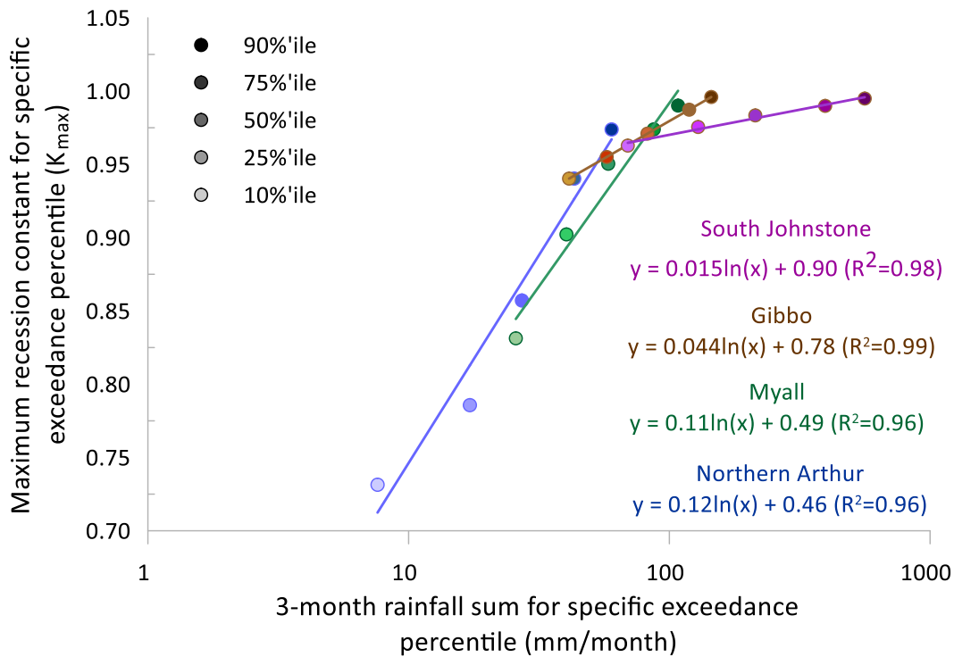
Figure 6 Maximum recession constant plotted against 3 monthly rainfall sums for specific exceedance percentiles: 10%, 25%, 50%, 75% and 90% (as indicated by degree of shading shown in plot legend). Results are provided for four catchments: Northern Arthur, Myall, Gibbo and South Johnstone.
