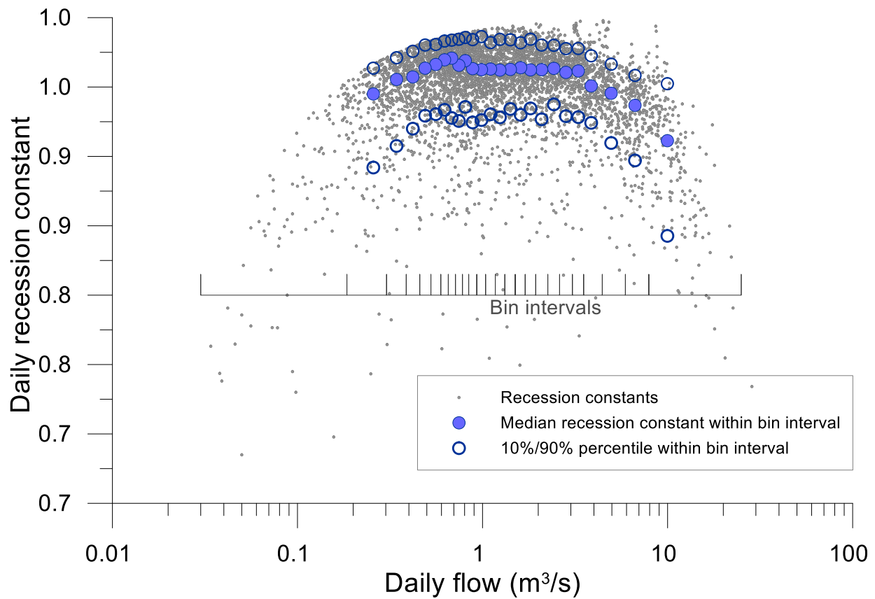
200 Figure 2 Relationship between daily recession constant and daily flow for Gibbo River at Gibbo Park 110 (401217) showing median, 10%ile, and 90%ile recession constants in each bin of 200 values.
