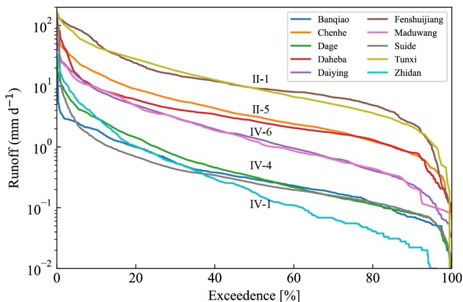
485 Figure 9. Event-scale flow-duration curves of the ten gauged catchments.
