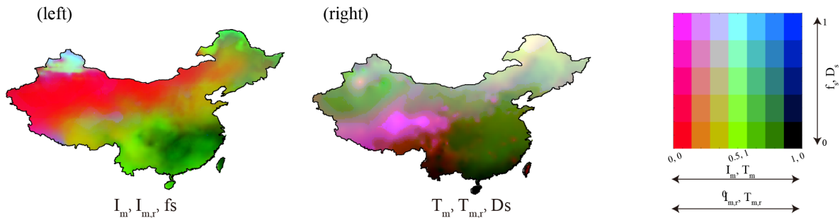
(g) Climate indices with RGB composite
