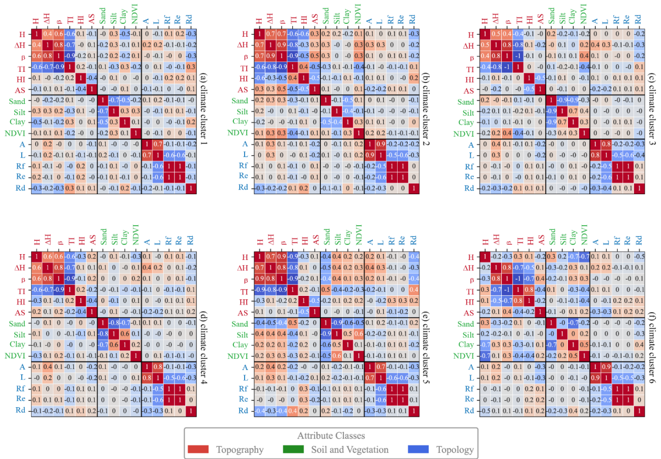
380 Figure 5. Spearman rank correlation coefficients for catchment attributes across different climate regions.
