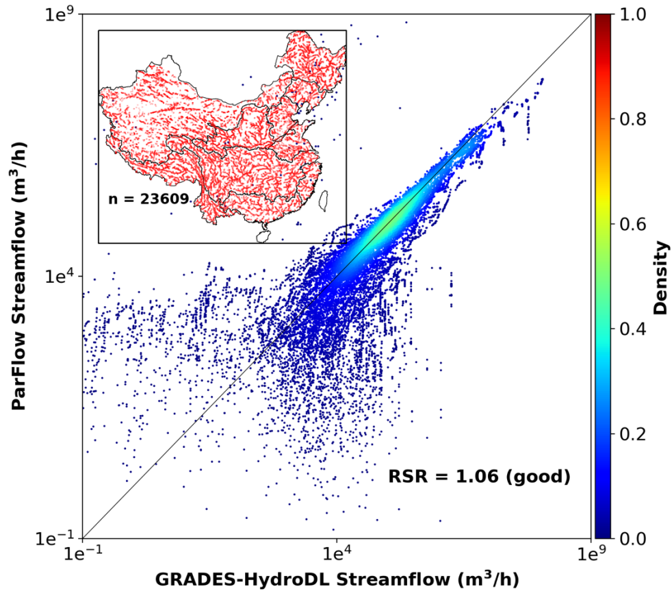
Figure 4. Scatterplot of simulated streamflow vs. GRADES-HydroDL. Locations of the selected reaches for comparison are shown in the upper left corner.
