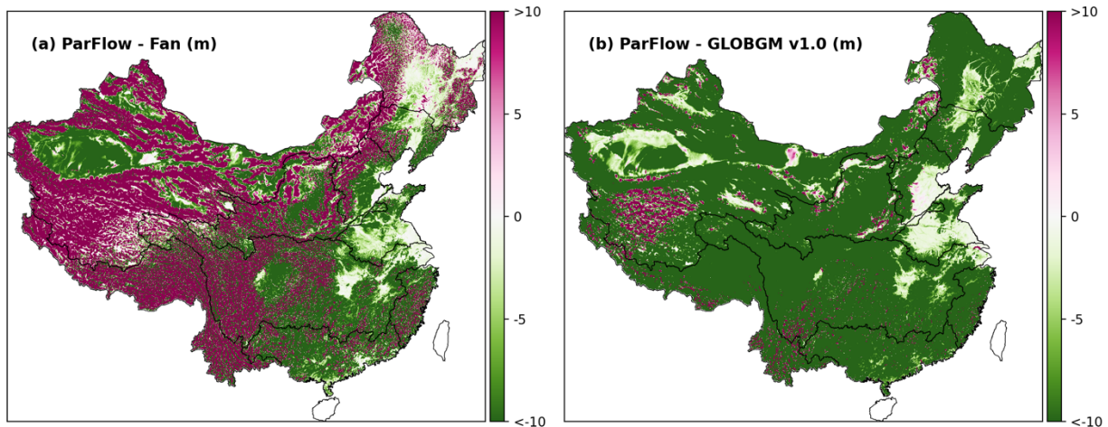
Figure 9. Differences of water table depth between CONCN 1.0 and two global models: (a) the difference between CONCN 1.0 and Fan’s model and (b) the difference between CONCN 1.0 and GLOBGM v1.0.
