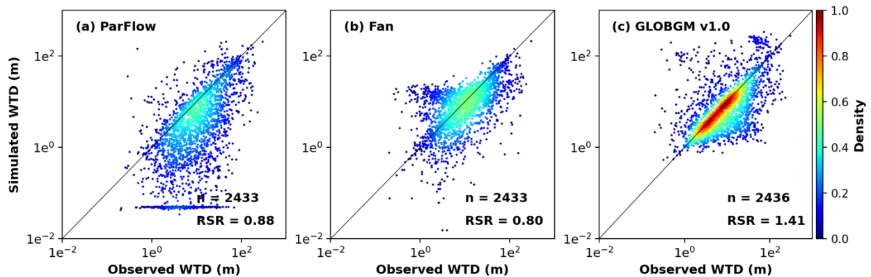
Figure 8. Scatterplots of simulations vs. observations of water table depth. The simulations are long-term average water table depths of 1981–2010 in current work, 2004–2014 in Fan's model, and 1958–2015 in GLOBGM v1.0. The observations are the averages of 2018.
