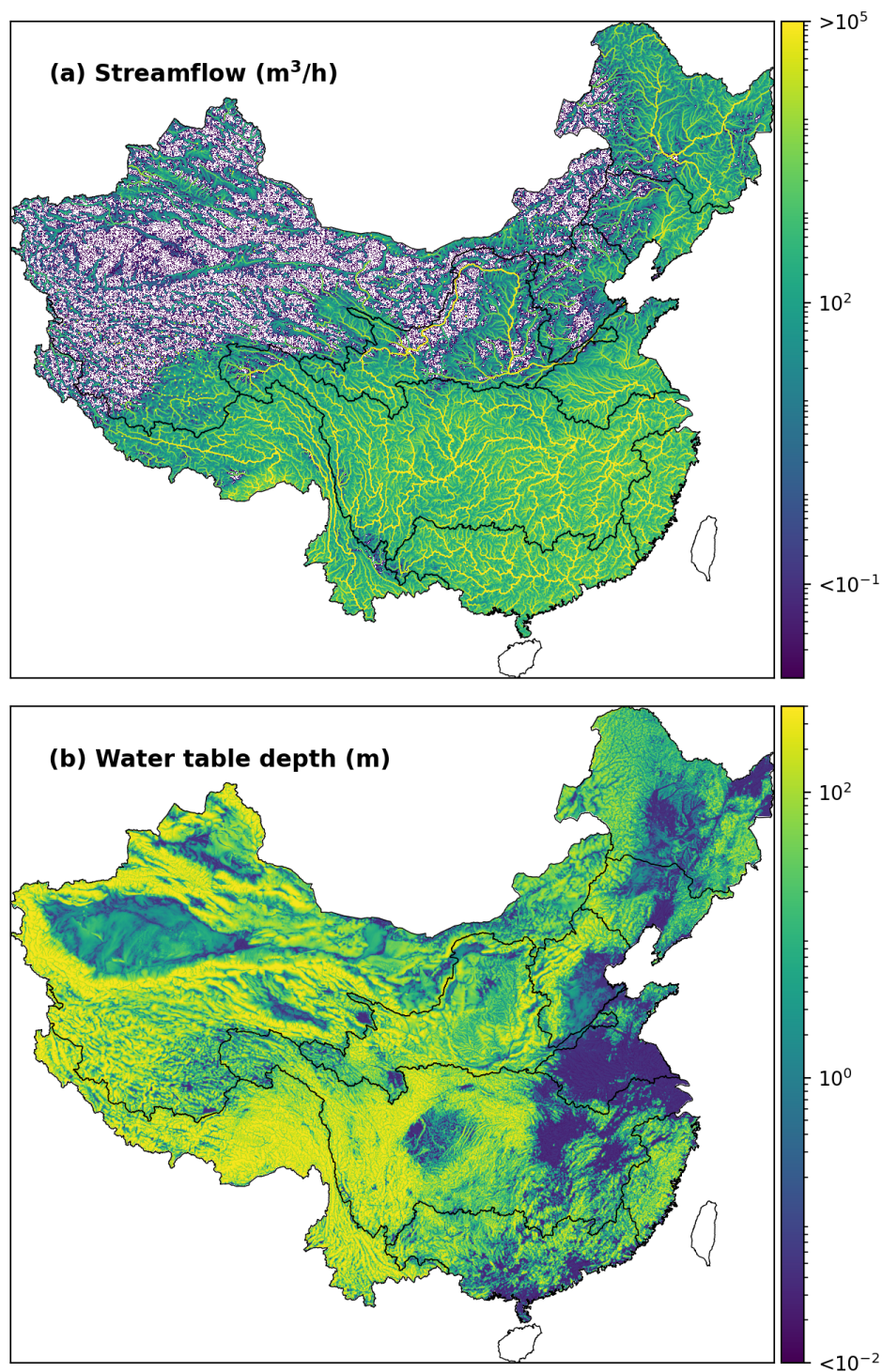
322 323 Figure 3. Simulated streamflow and water table depth by CONCN 1.0, representing the 324 average state from 1981 to 2010.
