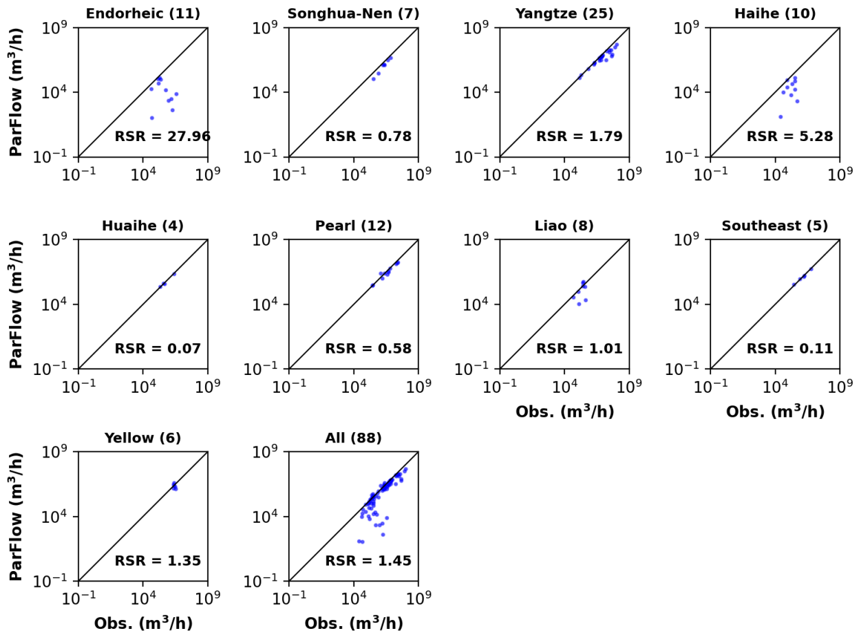
Figure 5. Scatterplots of simulated vs. observed streamflow for basins in Figure 1b and the entire CONCN 1.0 domain.
