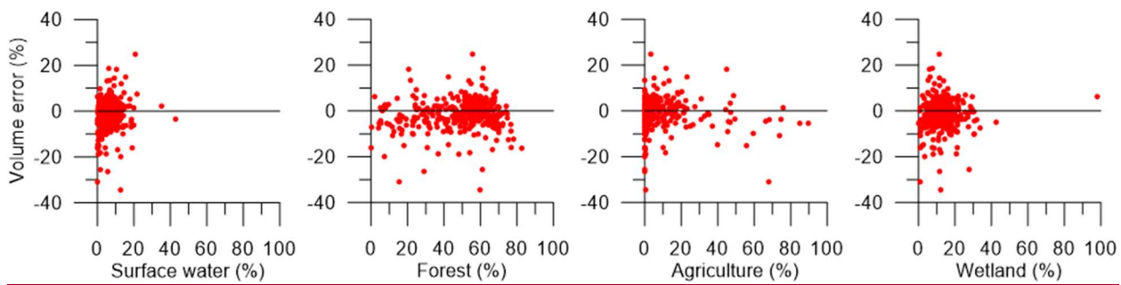
Figure B1. Scatter plot of volume errors versus percentages of surface water, forest, agriculture and wetland, 350 basins with at least 10 years of observations.
