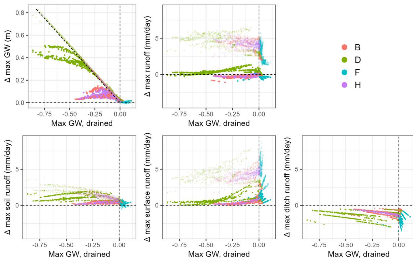
375 Figure 10: Changes in average yearly maximum groundwater level and runoff, including the runoff pathways at the time of maximum total runoff, as a function of the drained maximum groundwater level. Rewet1 cases in full color and Rewet2 cases shaded. At the diagonal line in the top left diagramsub-figure , a change with rewetting would bring the maximum groundwater level to the soil surface.
