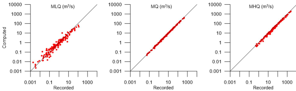
Figure B2. Evaluation of annual low flows, mean and annual high flows, daily means per station. NSE = 0.74, 0.99 and 0.95 respectively. 157 stations with at least 15 years of complete daily data, with negligible hydropower regulation.
