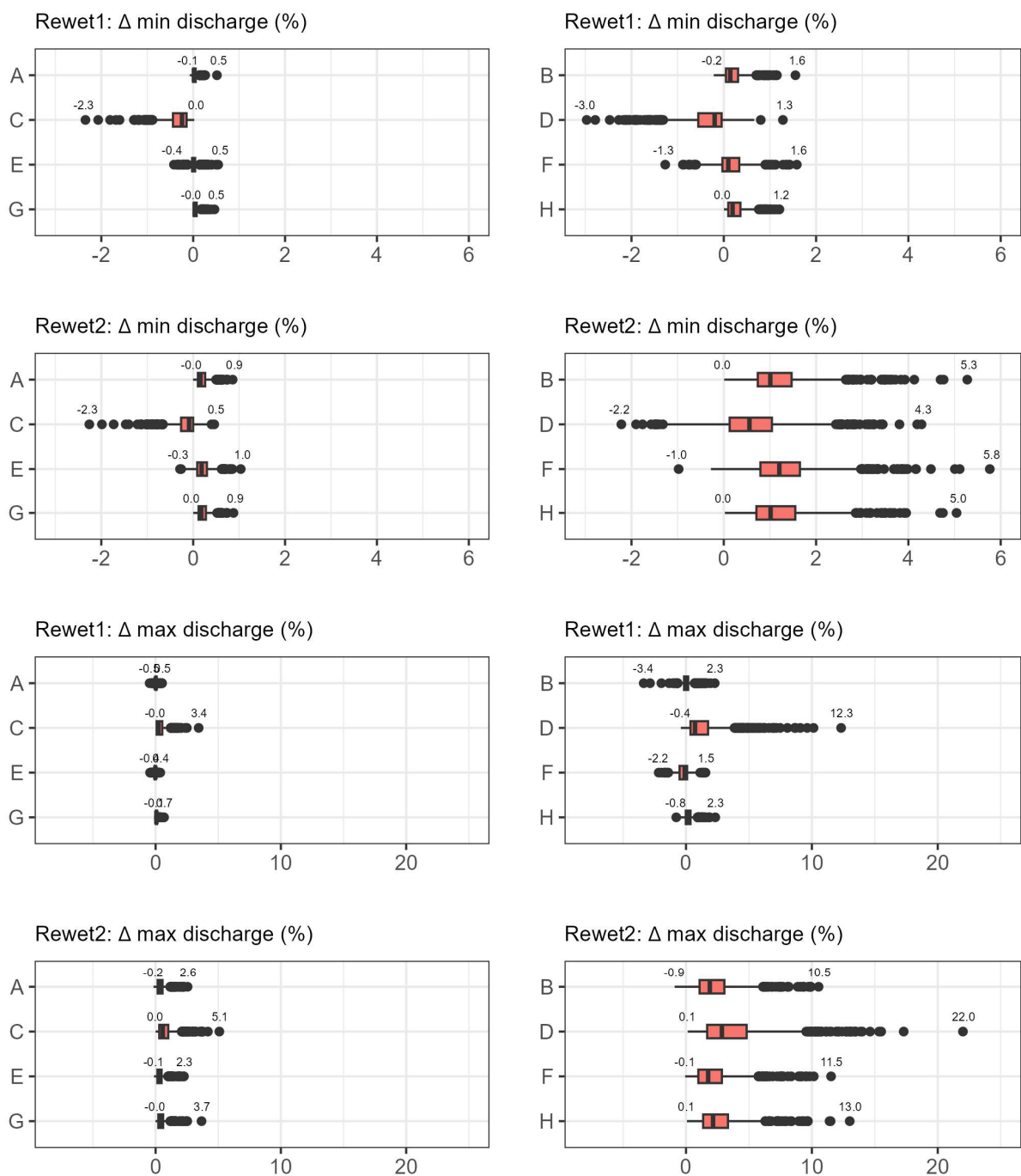
245 Figure 3: Changes in sub-catchment average yearly minimum and maximum discharge with rewetting. The statistics are based on the 656 sub-catchments that have coniferous forest on peatland (depth 1.5 m). Cases with 20 m influence (A, C, E, G) are presented in the left panels and cases with full influence (B, D, F, H) in the right panels.
