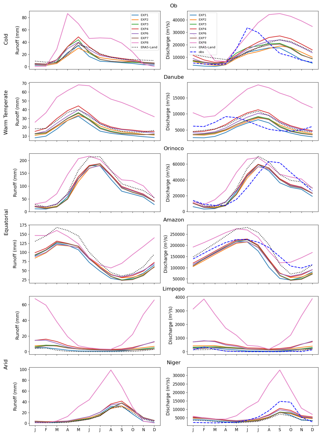
Figure 3: Mean seasonal cycle of runoff (mm) and river discharge ( m^3/s ) simulated by the different Noah-MP runoff schemes and CaMa-Flood, for 6 selected river basins representing four climate regions (cold, warm temperate, equatorial and arid). Discharge data includes simulated and observed values (obs) for the period 1985–2023. Observation years contributing to the monthly mean vary depending on their availability, with a minimum of 5 years per catchment.
