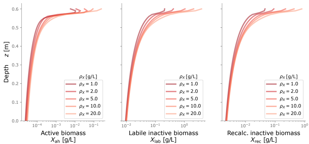
Figure C1. Biomass profiles under different values of biomass density \rho_X . Typical values are around 10 g/L.
