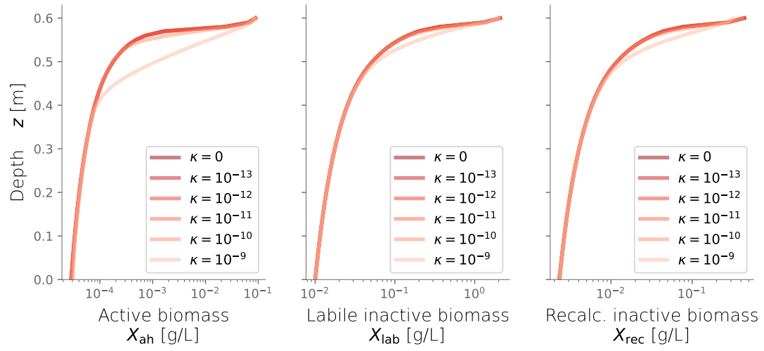
Figure C3. Biomass profiles under different values of diffusive growth coefficients \kappa . Values over 10^{-10} m/s are not expected.
