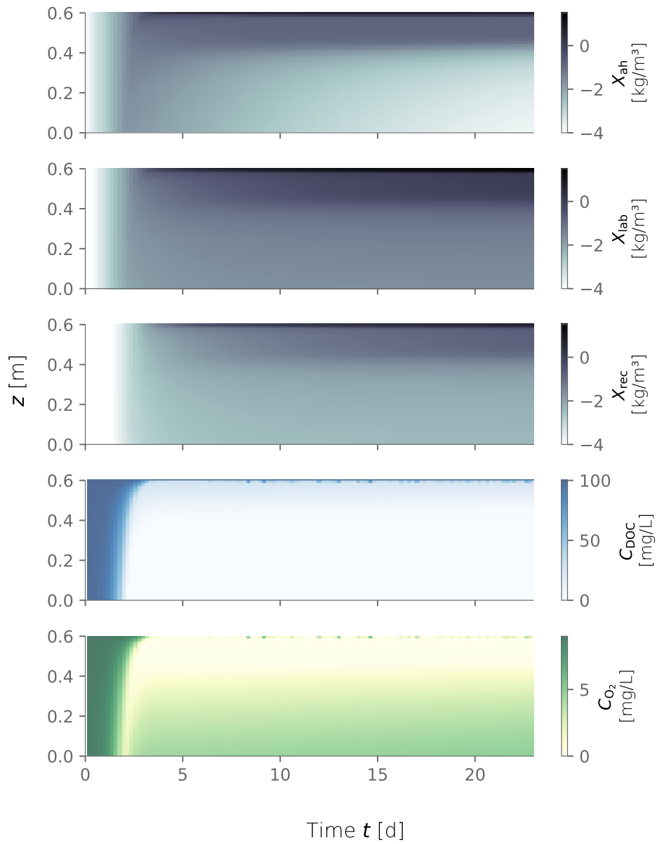
Figure D4. Biomass fractions, dissolved organic carbon (DOC) and dissolved oxygen ( O_2 ) over depth and over time for the constantly wet simulation.
