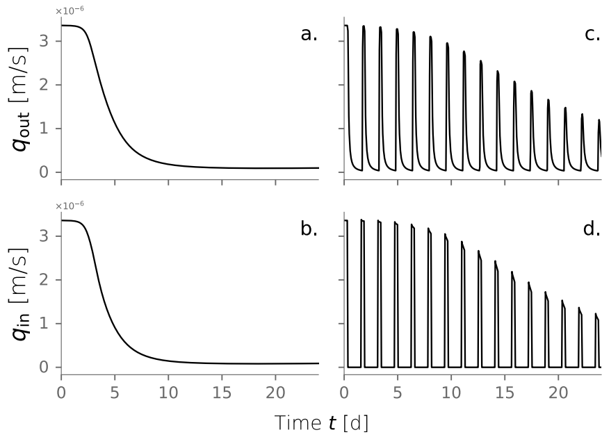
Figure D7. Water influx and outflux of the sand column simulations. Figures a-b correspond to the always wet experiment. Figures c-d show dry/wet cycles of 1800-450 min. This is a complement to data shown in Figure 5a and 5c.
