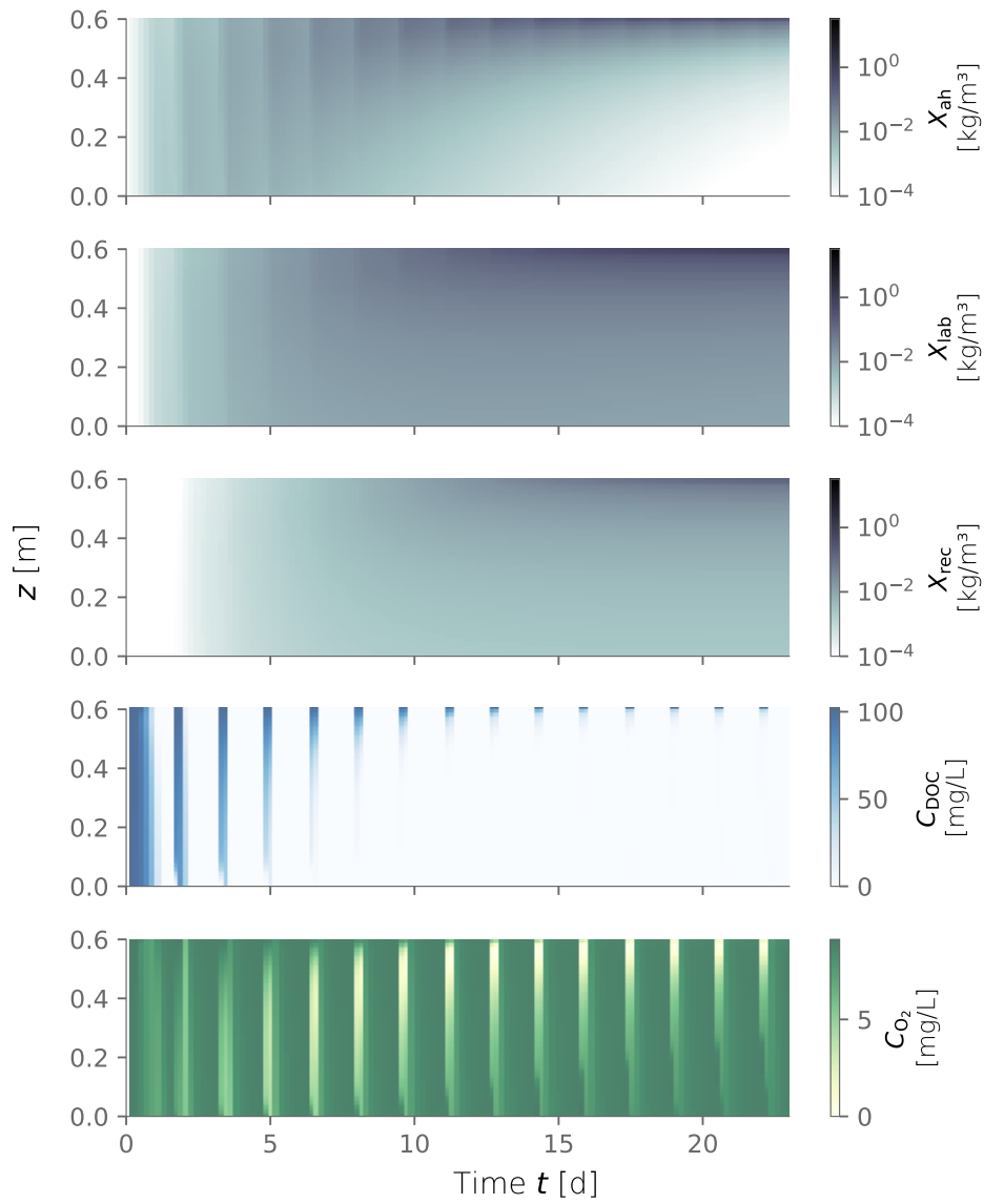
Figure D6. Biomass fractions, dissolved organic carbon (DOC) and dissolved oxygen ( O_2 ) over depth and over time for dry/wet cycles of 1800-450 min.
