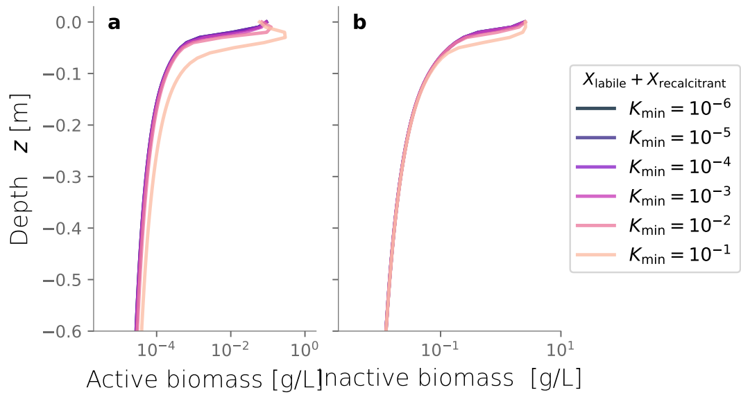
Figure C5. Biomass profiles under different values of biomass hydraulic conductivity K_{\min} . Values are relative to the porous medium's clean saturated hydraulic conductivity.
