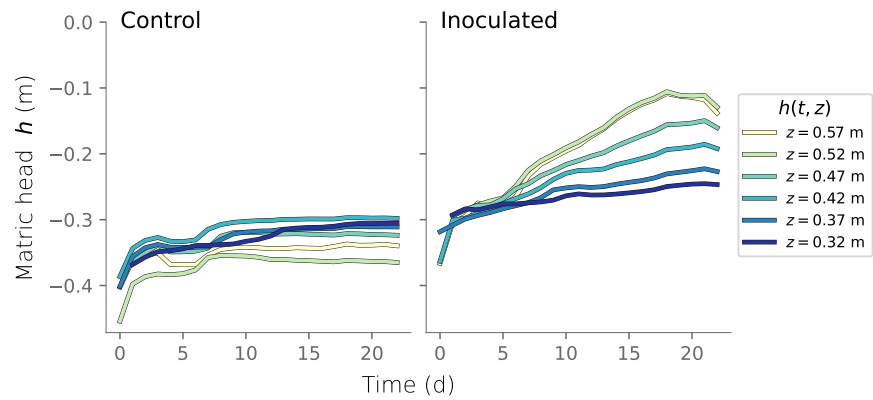
Figure B1. Time series of matric head measured at six different depths in the column experiments.
