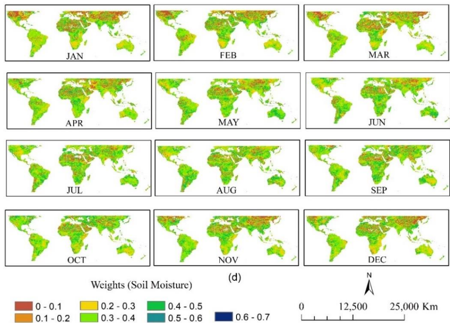
Figure C4. Monthly spatial distribution of PCA-derived weights for soil moisture (d), Colour scales indicate the relative contribution of each variable to CDI (brown = low weight, green = moderate weight, blue = high weight).
