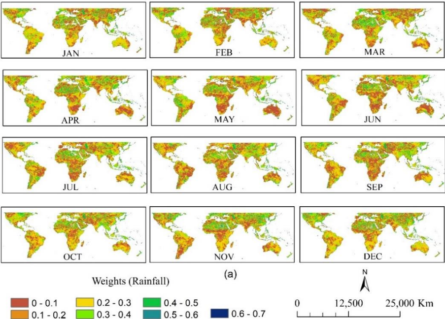
955 Figure C1. Monthly spatial distribution of PCA-derived weights for rainfall (a), Colour scales indicate the relative contribution of each variable to CDI (brown = low weight, green = moderate weight, blue = high weight).
