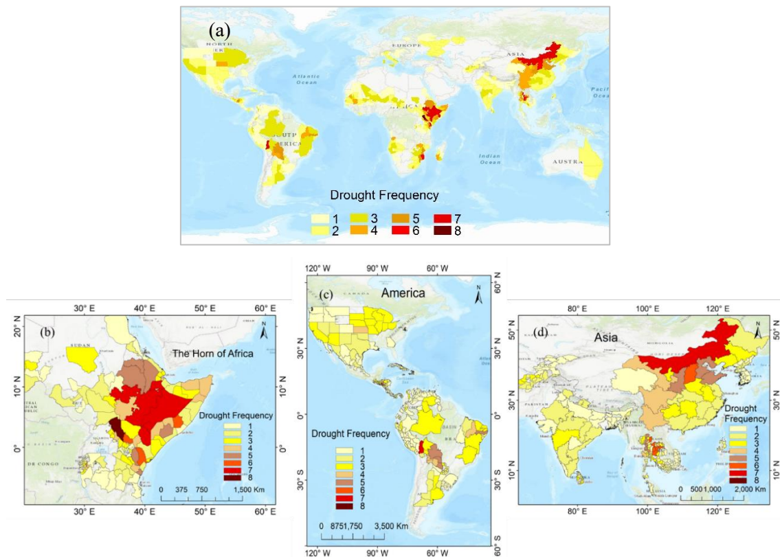
345 Figure 2. Spatial distribution of GDIS drought frequencies: (a) Global scale, (b) East Africa, (c) America, and (d) Asia. The drought frequencies range from one to eight, represented by shades from light yellow (low frequency) to dark brown (high frequency). Note: The color scheme used here is distinct from the CDI classification shown in Table 2 and represents event frequency, not drought intensity.
