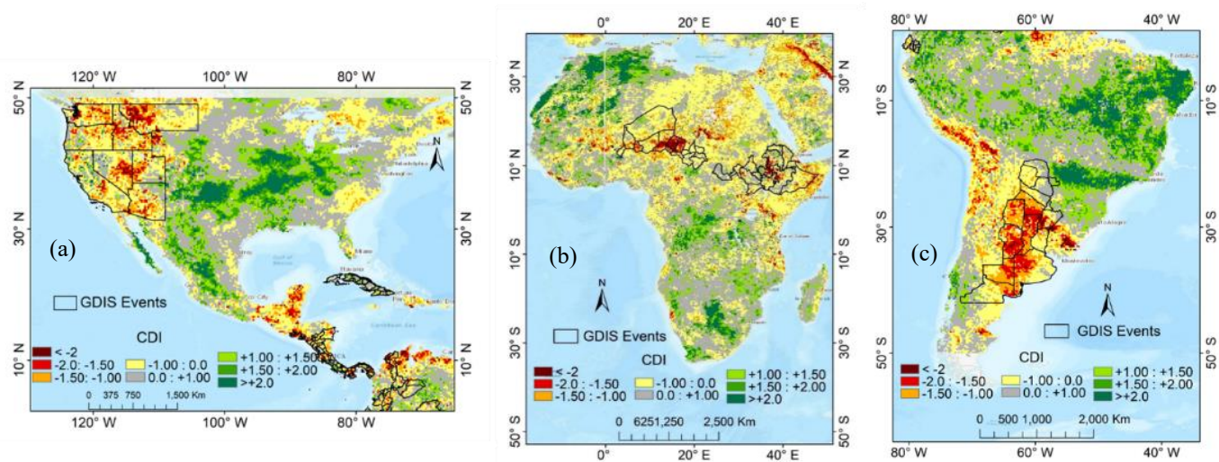
405 Figure 4. Assessment of Drought Using CDI with Overlay of GDIS Events over America (June 2015) (a), Africa (June 2009) (b), and South America (August 2009) (c). The black polygons represent GIS polygons from GDIS, indicating drought-affected administrative units based on GDIS data. The base maps display CDI results for the respective GDIS drought months, ranging from dark brown (indicating extreme dry conditions) to dark green (indicating extreme wet conditions). The alignment of GDIS polygons with droughts detected by CDI demonstrates the CDI's capability to accurately identify GDIS droughts during the respective periods.
