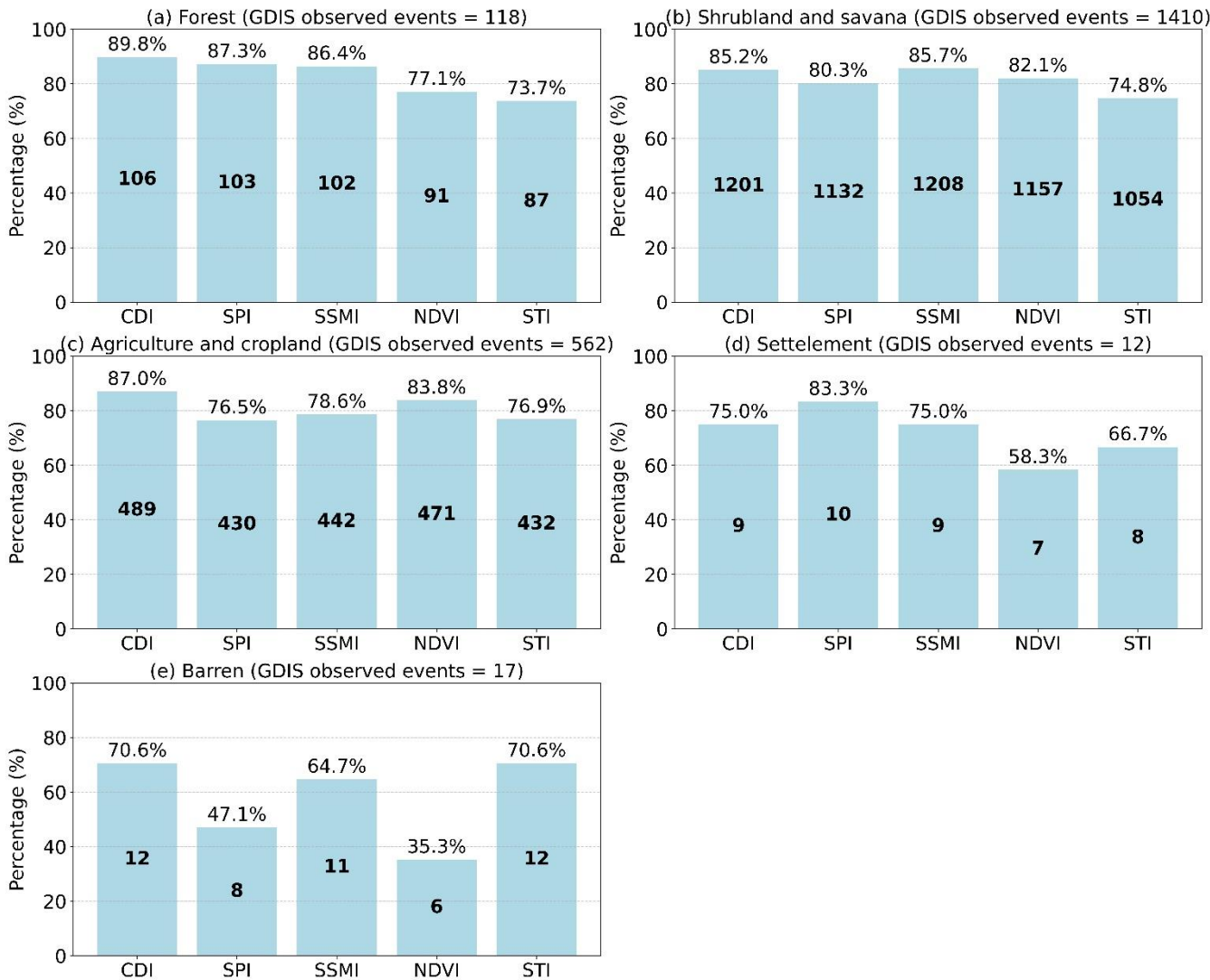
1045 Figure H1. Land cover-wise accuracy of drought indices (CDI, SPI, SSMI, NDVI, STI) in detecting GDIS events across five major land cover classes (Forest, Shrubland and Savanna, Agriculture and Cropland, Settlement, and Barren) based on MODIS land cover data. The bar heights represent the percentage of GDIS events accurately captured, while values inside the bars indicate the absolute number of consistent detections. The total number of GDIS events considered per land cover class is Forest – 118, Shrubland and Savanna – 1410, Agriculture and Cropland – 562, Settlement – 12, Barren – 17.
