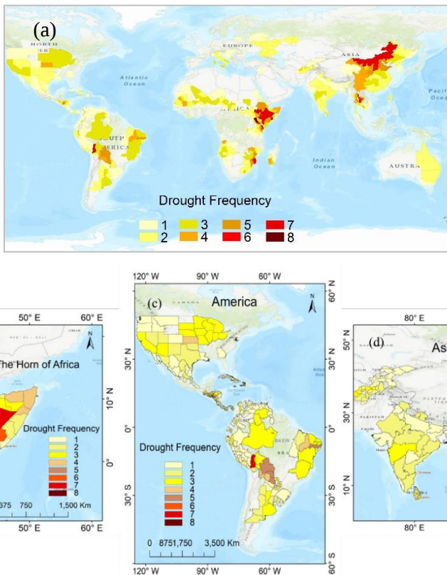
Figure 2. Spatial distribution of GDIS drought frequencies: (a) Global scale, (b) East Africa, (c) America, and (d) Asia. The drought frequencies range from one to eight, represented by shades from light yellow (low frequency) to dark brown (high frequency). Note: The color scheme used here is distinct from the CDI classification shown in Table 2 and represents event frequency, not drought intensity.
