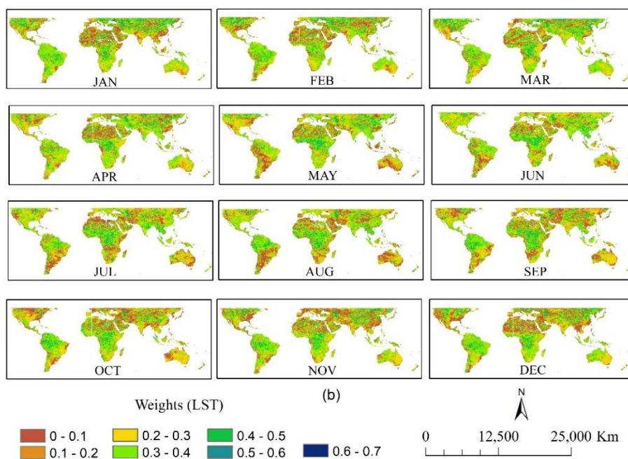
Figure B2. Monthly spatial distribution of PCA-derived weights for temperature (b), Colour scales indicate the relative contribution of each variable to CDI (brown = low weight, green = moderate weight, blue = high weight).
