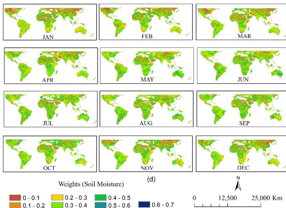
Figure B4. Monthly spatial distribution of PCA-derived weights for soil moisture (d), Colour scales indicate the relative contribution of each variable to CDI (brown = low weight, green = moderate weight, blue = high weight).
