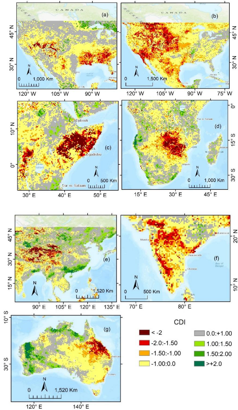
Appendix C: Significant drought events detected by CDI in various global regions include: (a) the USA in August 2007 and 970 (b) July 2012, (c) the Horn of Africa in July 2015, (d) Malawi and Zambia in February 2016, (e) western and northern China in July 2015, (f) India in July 2015, and (g) Australia in January 2019.
