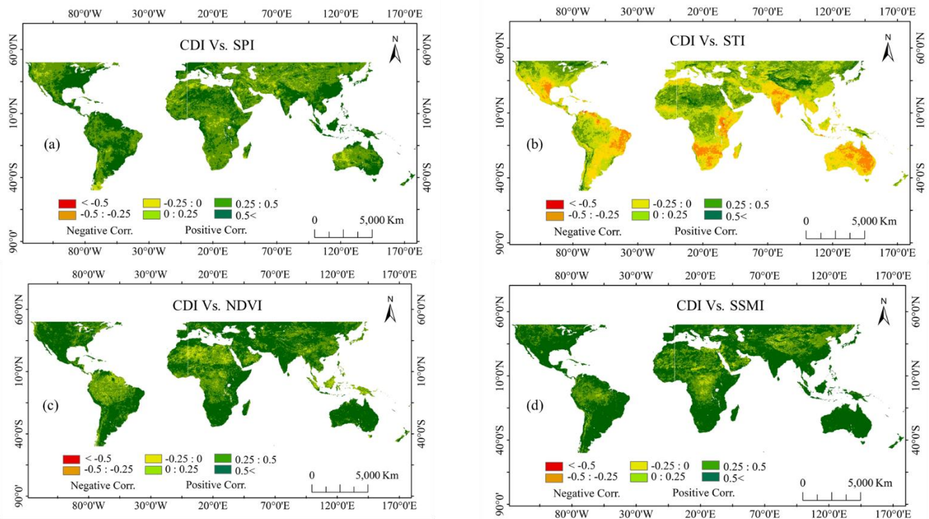
565 Figure 9. Spatial correlation between CDI and single input-based traditional indices for a sample month (April): (a) CDI vs. SPI, (b) CDI vs. STI, (c) CDI vs. NDVI, and (d) CDI vs. SSMI. Negative correlations are represented in shades from yellow to red, while positive correlations are shown in shades from light green to dark green.
