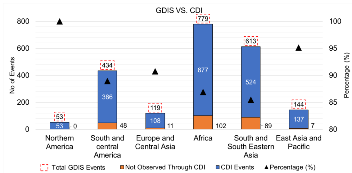
445 Figure 5. Performance of CDI in Detecting GDIS Events Across Different Geographic Regions. A total of 2142 drought events were identified from GDIS. CDI successfully detected events marked in blue, with counts indicated by red dotted boxes. Events missed by CDI are represented in orange. The black triangles indicate the percentage of GDIS events captured by CDI.
