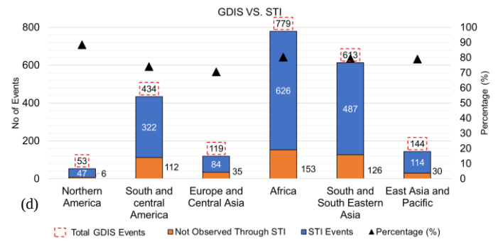
Appendix D: Performance of Traditional Drought Indices in Capturing GDIS Events Across Global Regions: Comparative Assessment of (a) NDVI, (b) SPI, (c) SSMI, and (d) STI
