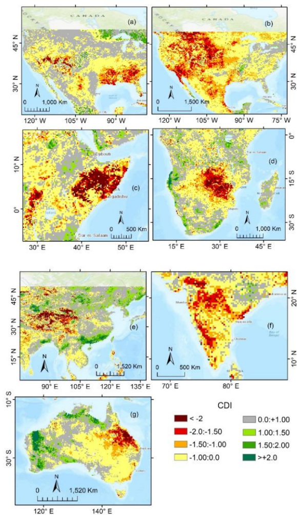
Figure 3: Major drought events detected by CDI in various global regions include: (a) the USA in August 2007 and (b) July 2012, (c) the Horn of Africa in July 2015, (d) Malawi and Zambia in February 2016, (e) western and northern China in July 2015, (f) India in July 2015, and (g) Australia in January 2019.
