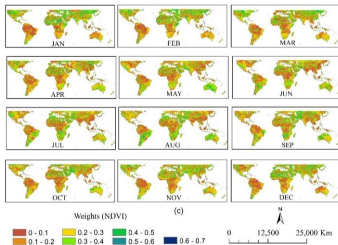
Figure C3. Monthly spatial distribution of PCA-derived weights for NDVI (c), Colour scales indicate the relative contribution of each variable to CDI (brown = low weight, green = moderate weight, blue = high weight).
