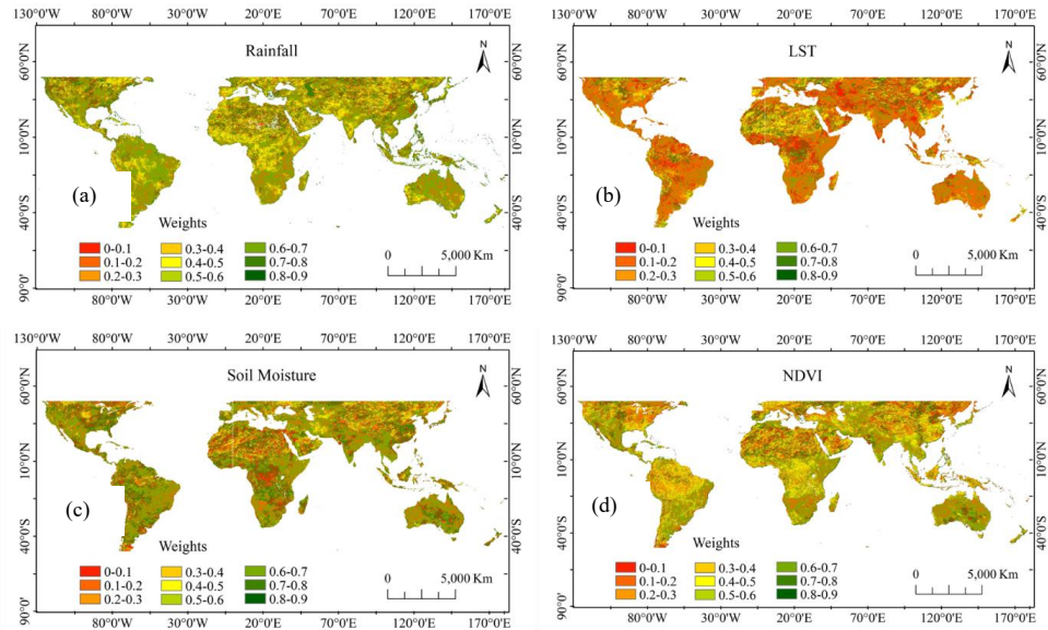
Figure B1. Example of pixel-based weights for the four input variables of CDI: rainfall (a), LST (b), soil moisture (c), and NDVI (d), calculated using the PCA method for a sample month (April). The weights range from 0 to 1, with colors varying from dark red (lower weights) to dark green (higher weights).
