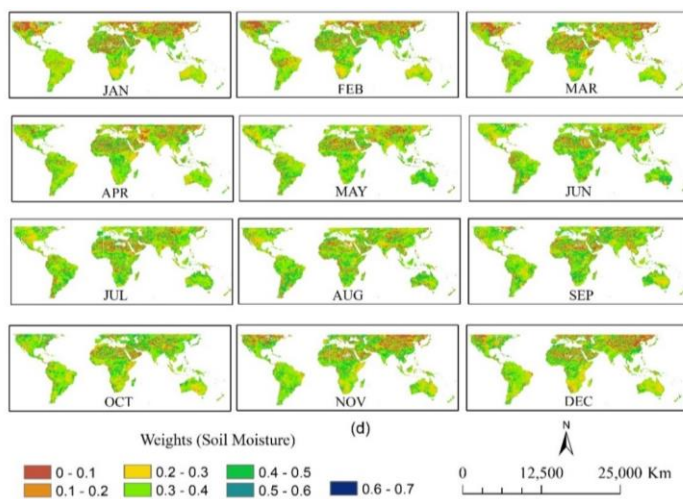
Figure C4. Monthly spatial distribution of PCA-derived weights for soil moisture (d), Colour scales indicate the relative contribution of each variable to CDI (brown = low weight, green = moderate weight, blue = high weight).
