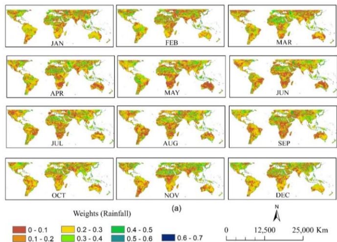
Figure C1. Monthly spatial distribution of PCA-derived weights for rainfall (a), Colour scales indicate the relative contribution of each variable to CDI (brown = low weight, green = moderate weight, blue = high weight).
