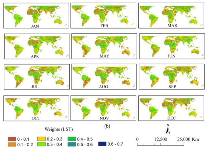
Figure C2. Monthly spatial distribution of PCA-derived weights for temperature (b), Colour scales indicate the relative contribution of each variable to CDI (brown = low weight, green = moderate weight, blue = high weight).
