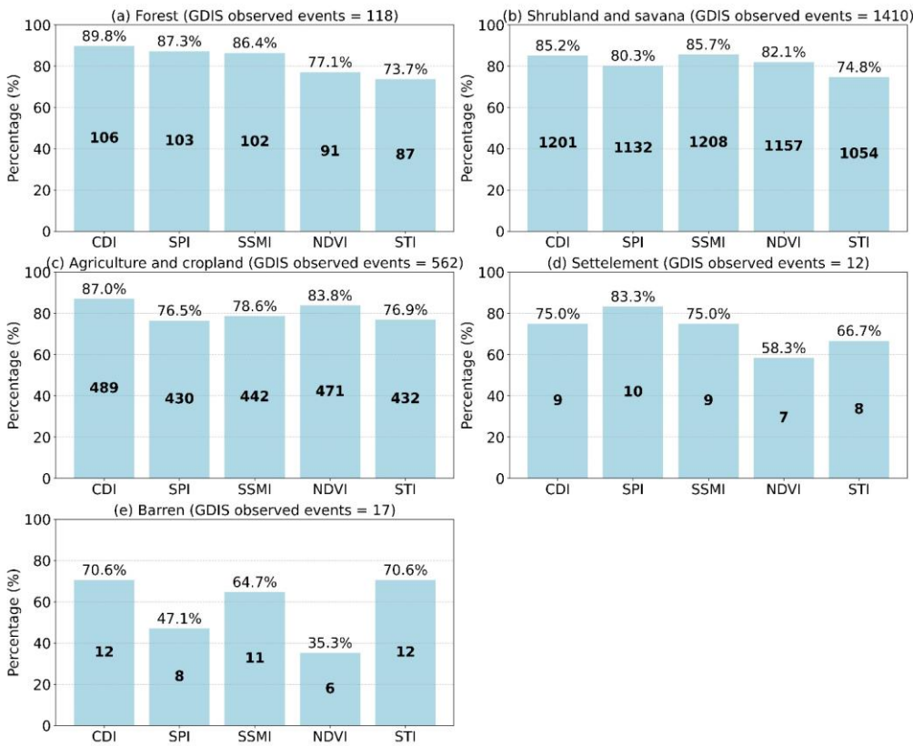
Figure H11. Land cover-wise accuracy of drought indices (CDI, SPI, SSMI, NDVI, STI) in detecting GDIS events across five major land cover classes (Forest, Shrubland and Savanna, Agriculture and Cropland, Settlement, and Barren) based on MODIS land cover data. The bar heights represent the percentage of GDIS events accurately captured, while values inside the bars indicate the absolute number of consistent detections. The total number of GDIS events considered per land cover class is Forest – 118, Shrubland and Savanna – 1410, Agriculture and Cropland – 562, Settlement – 12, Barren – 17.
