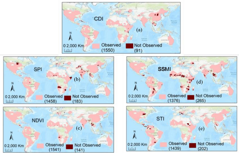
Figure E1. Spatial locations-wise performance of CDI (a), SPI (b), NDVI (c), SSMI (d), and STI (e) in detecting GDIS events, where consistent events detected by each index are shown in pink, while inconsistent GDIS events (not observed) are shown in dark brown. The drought identification criteria were set to events during the actual drought period without considering short droughts (total GDIS events count = 1641).
