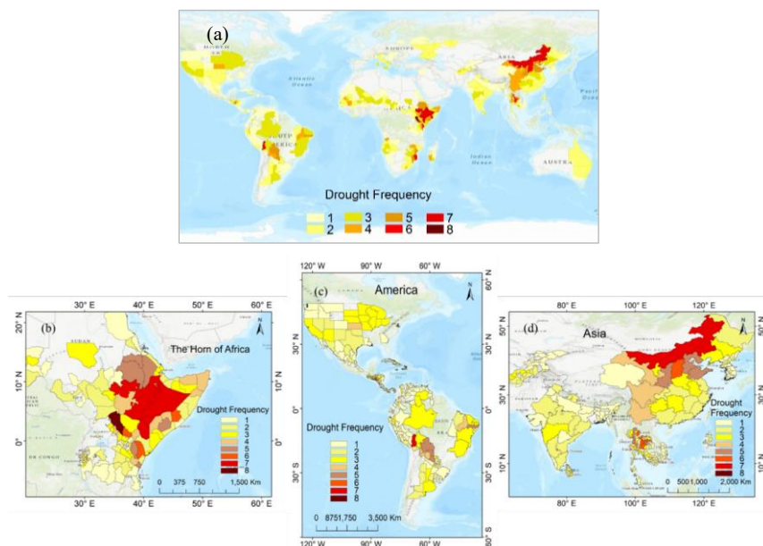
Figure 2. Spatial distribution of GDIS drought frequencies: (a) Global scale, (b) East Africa, (c) America, and (d) Asia. The drought frequencies range from one to eight, represented by shades from light yellow (low frequency) to dark brown (high frequency). Note: The color scheme used here is distinct from the CDI classification shown in Table 2 and represents event frequency, not drought intensity.
