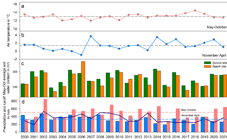
Figure 2: Average air temperatures in summer (a) and winter seasons (b) , May-October average soil water content (c) and precipitation sums and runoff (d) . The red columns represent the summer seasons (May–October), and the blue columns represent the winter seasons (November–April), dashed lines represent season average values , and dark blue line represents runoff .
