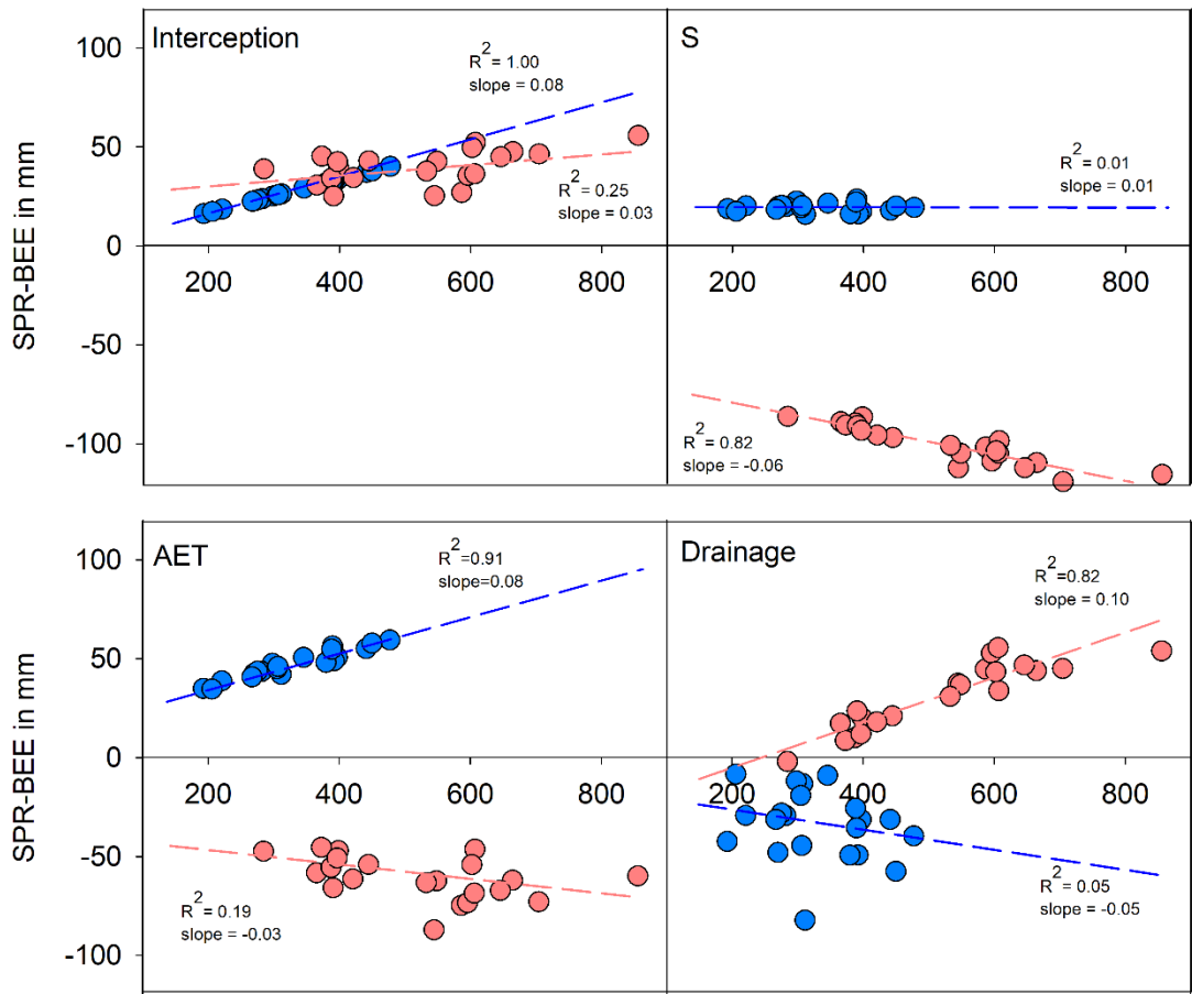
400 Figure 6: Differences between spruce and beech modelled soil water fluxes (AET, D) during summer (May to October, orange colour) and winter (November to April, blue colour) in relation to precipitation. AET can also be divided into INT and S (upper panel).
