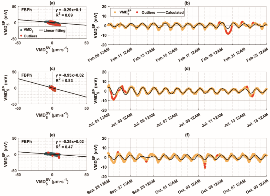
Figure 8: The relationship between the fifth decomposed modes of sap velocity ( VMD_5^{SV} ) and tree SP signals ( VMD_5^{SP} ) in (a–b) winter, (c–d) summer, and (e–f) autumn of 2023 for the Aleppo pine (FBPh) at the Font-Blanche. (a, c, e) Scatter plots of the decomposed modes of sap velocity and SP signals with black lines indicating linear regression results and red dots indicating points (outliers) outside the 95% confidence level of the regression. (b, d, f) Corresponding decompositions of SP signals (orange dots) and calculated SP (black lines) based on the linear relationship between VMD_5^{SV} and VMD_5^{SP} , with red dots as outliers outside the 95% confidence level of the linear regression.
