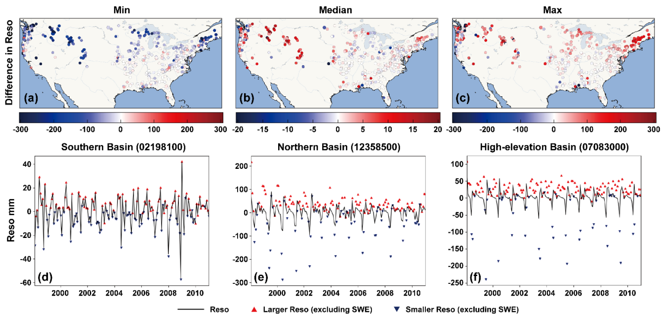
620 Figure 14. Comparison of Res_o obtained from residual decomposition excluding SWE with the original values. (a-c) Spatial distribution of monthly mean Res_o excluding SWE minus its original values. (d-f) Time series of Res_o excluding SWE and its original values at the southern basin (02198100, 32.96°N), northern basin (12358500, 48.33°N), and high-elevation basin (07083000, elevation of 3.56 km) at monthly scale. The unit of residuals is “mm”.
