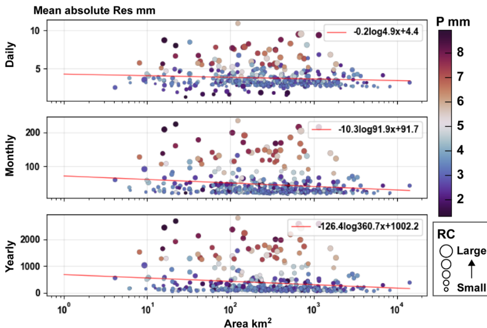
555 Figure 12. Relationship between the mean absolute of water budget residuals, basin area, long-term average daily precipitation, and runoff coefficient (RC) over 475 CAMELS basins with reliable simulations. The respective red lines represent the linear regression of residuals with basin area for each timescale.
