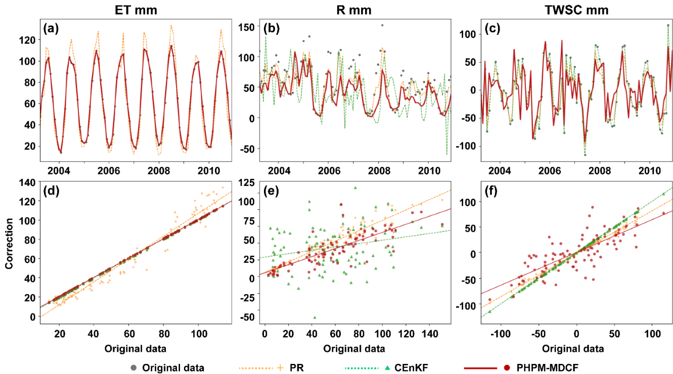
530 Figure 11. Comparison of monthly correction results between the PHPM-MDCF and existing methods (PR and CEnKF) at basin 1539000. (a-c) Time series of the original and corrected measurements of evaporation, runoff, and terrestrial water storage change. (d-f) Scatter plots and regression lines of the original and corrected measurements.
