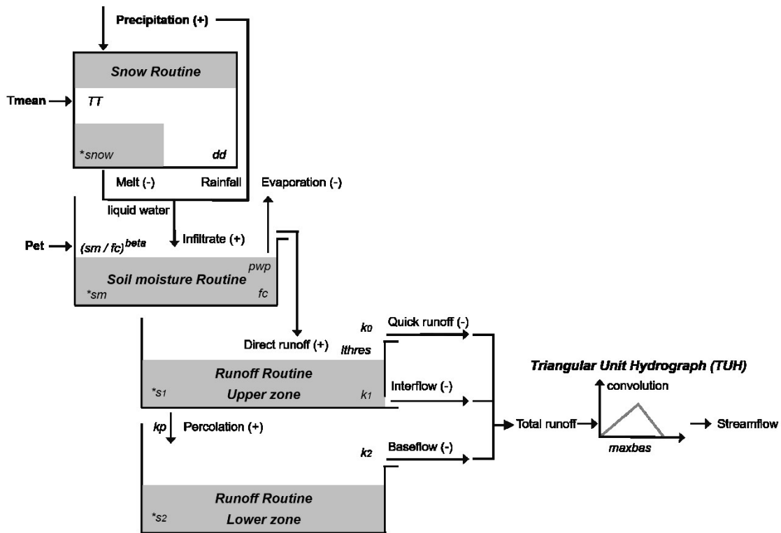
845 Figure A1. Schematic structure of the HBV model. The variables marked with asterisk (*) denote water storage, whereas those annotated with positive (+) and negative (-) signs represent the inputs and outputs of the storage.
